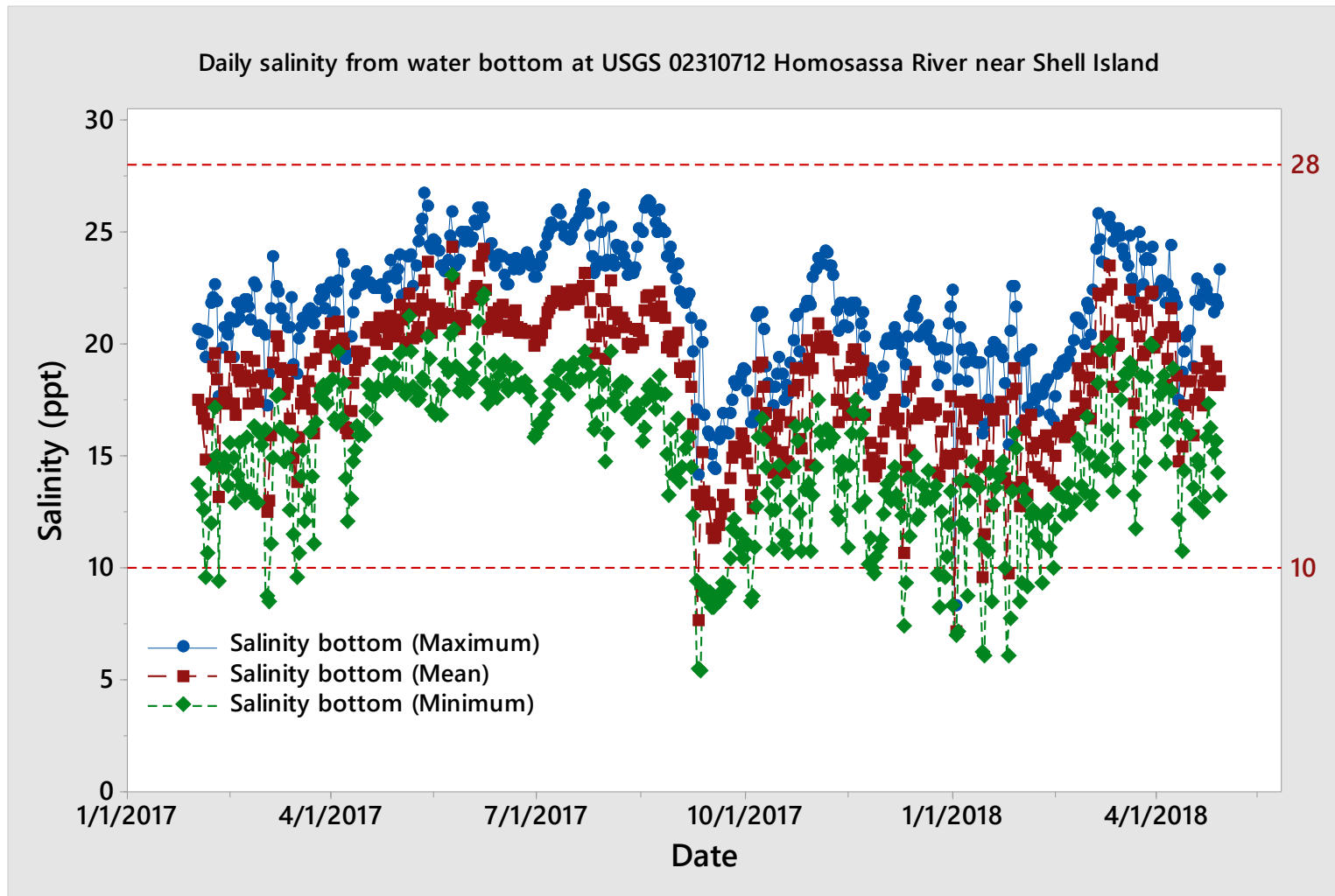
Figure 26. Maximum, mean, and minimum daily salinity (ppt) values from water bottom samples at USGS Station 02310712 Homosassa River near Shell Island from 2/1/2017 to 4/30/2018. Dashed lines at 10 ppt and 28 ppt mark the minimum and maximum salinity tolerance level for optimal growth and reproduction of Crassostrea virginica .
