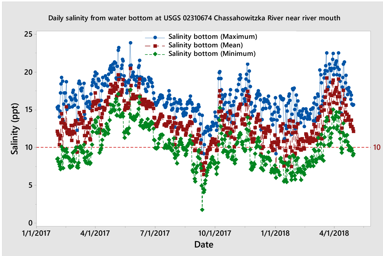
Figure 19. Maximum, mean, and minimum daily salinity (ppt) values from water bottom samples at USGS Station 02310674 Chassahowitzka River near river mouth from 2/1/2017 to 4/30/2018. Dashed line at 10 ppt marks the minimum salinity tolerance level for optimal growth and reproduction of Crassostrea virginica .
