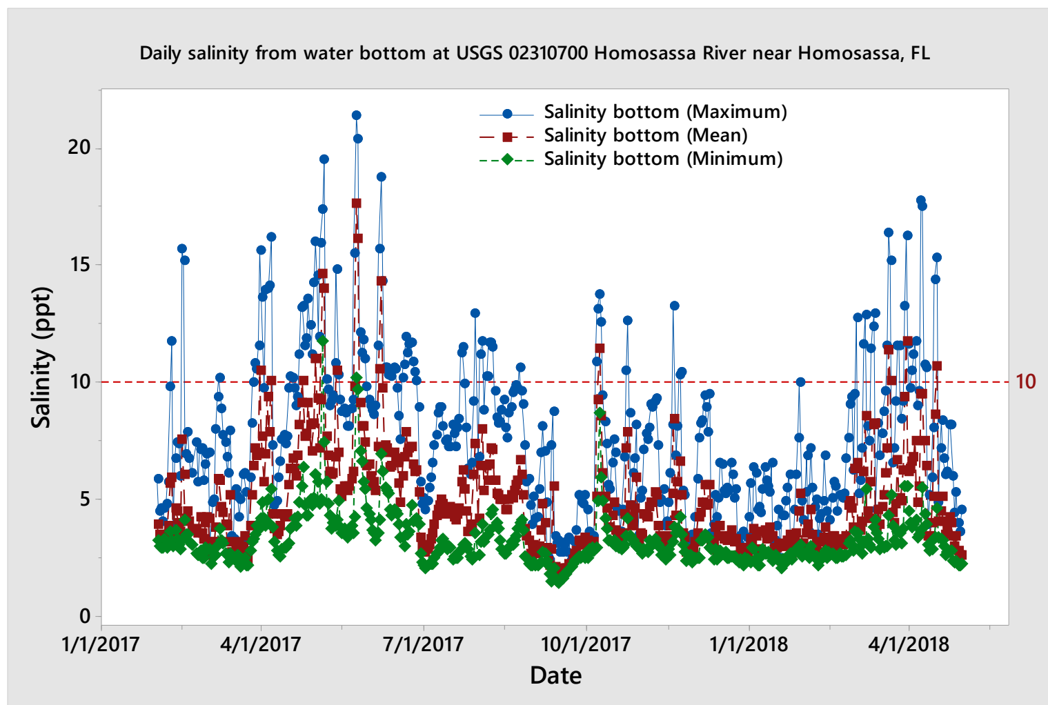
Figure 24. Maximum, mean, and minimum daily salinity (ppt) values from water bottom samples at USGS Station 02310700 Homosassa River near Homosassa, Florida from 2/1/2017 to 4/30/2018. Dashed line at 10 ppt marks the minimum salinity tolerance level for optimal growth and reproduction of Crassostrea virginica .
