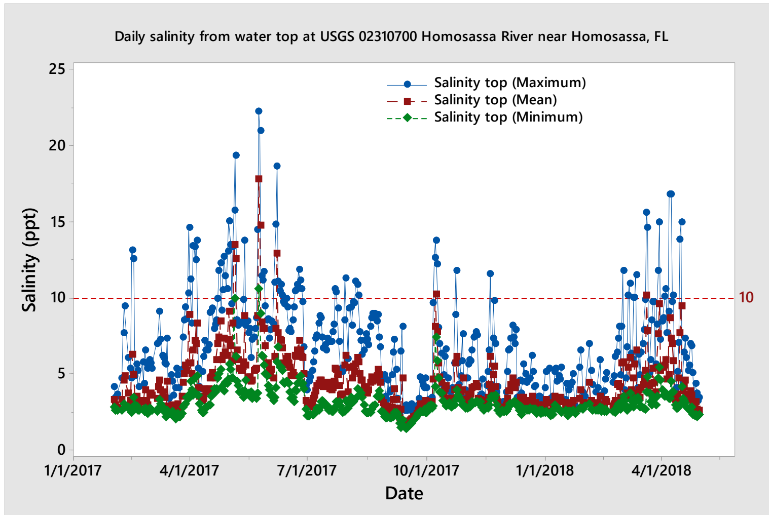
Figure 23. Maximum, mean, and minimum daily salinity (ppt) values from water top samples at USGS Station 02310700 Homosassa River near Homosassa, Florida from 2/1/2017 to 4/30/2018. Dashed line at 10 ppt marks the minimum salinity tolerance level for optimal growth and reproduction of Crassostrea virginica .
