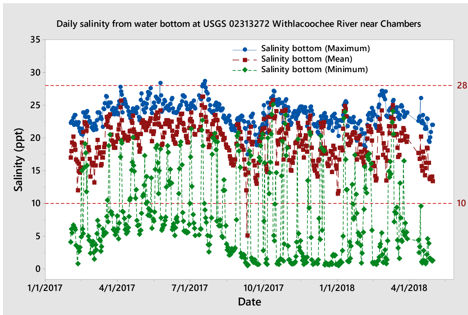
Figure 28. Maximum, mean, and minimum daily salinity (ppt) values from water bottom samples at USGS Station 02313272 Withlacoochee River near Chambers from 2/1/2017 to 4/30/2018. Dashed lines at 10 ppt and 28 ppt mark the minimum and maximum salinity tolerance level for optimal growth and reproduction of Crassostrea virginica .
