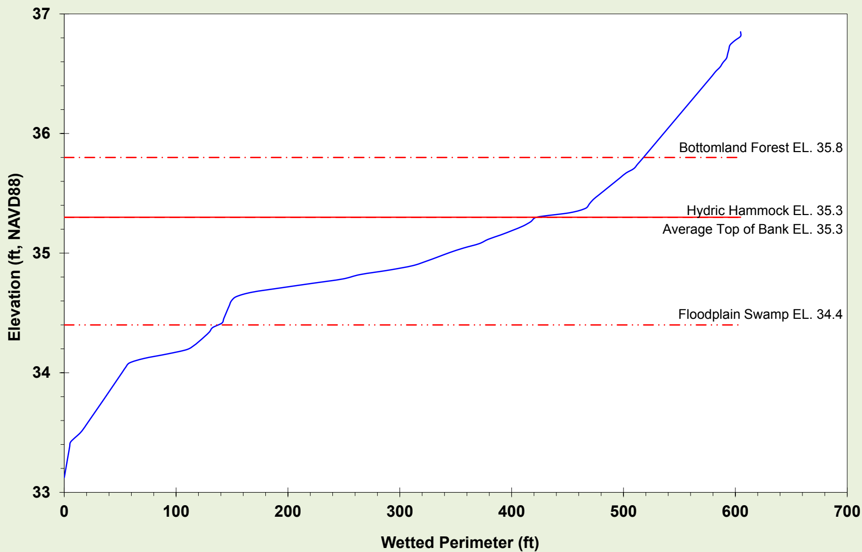
Figure 37. Wetted Perimeter for Transect 9
