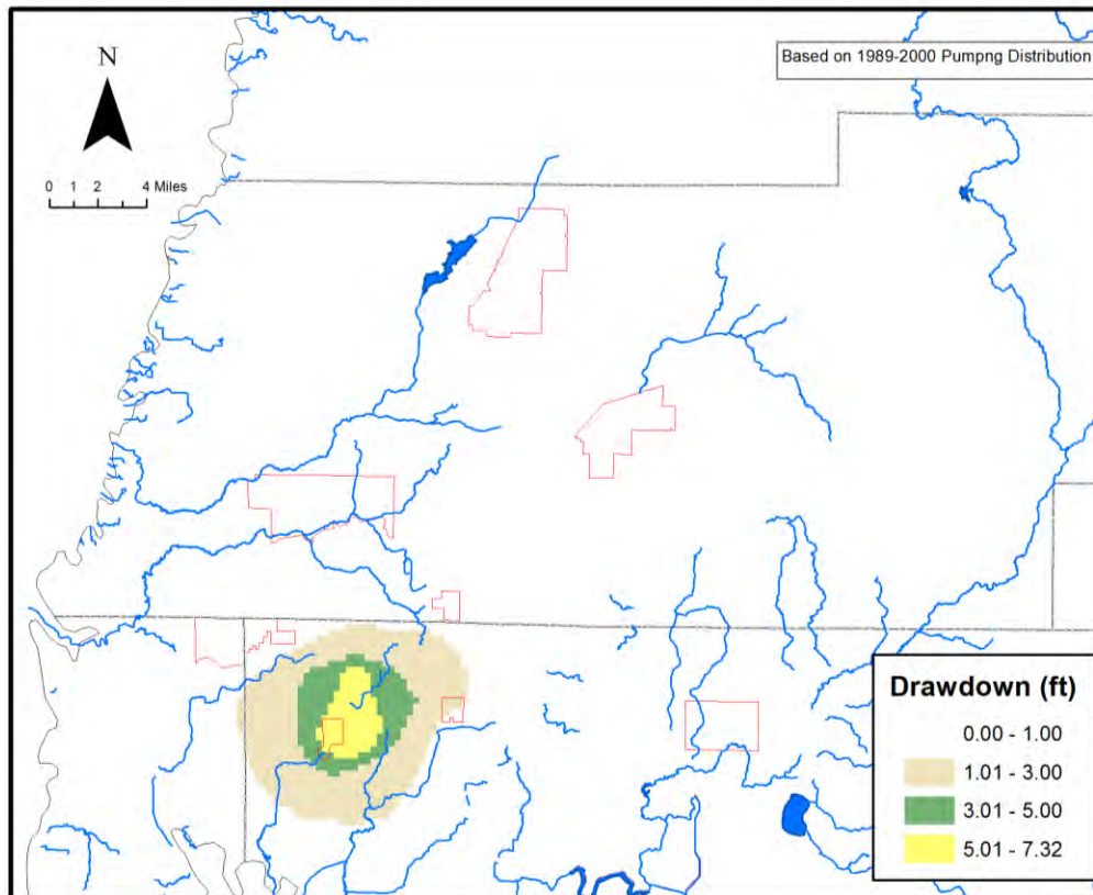
Predicted mean drawdown in the Upper Floridan aquifer due to Cosme-Odessa wellfield withdrawals from 1989-2000.
