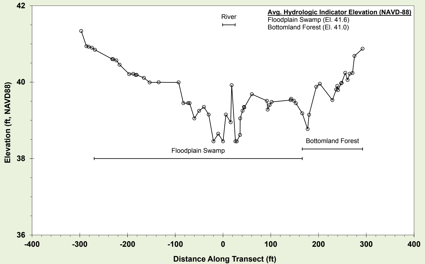
Figure 19. Pithlachascotee River, Transect 13
