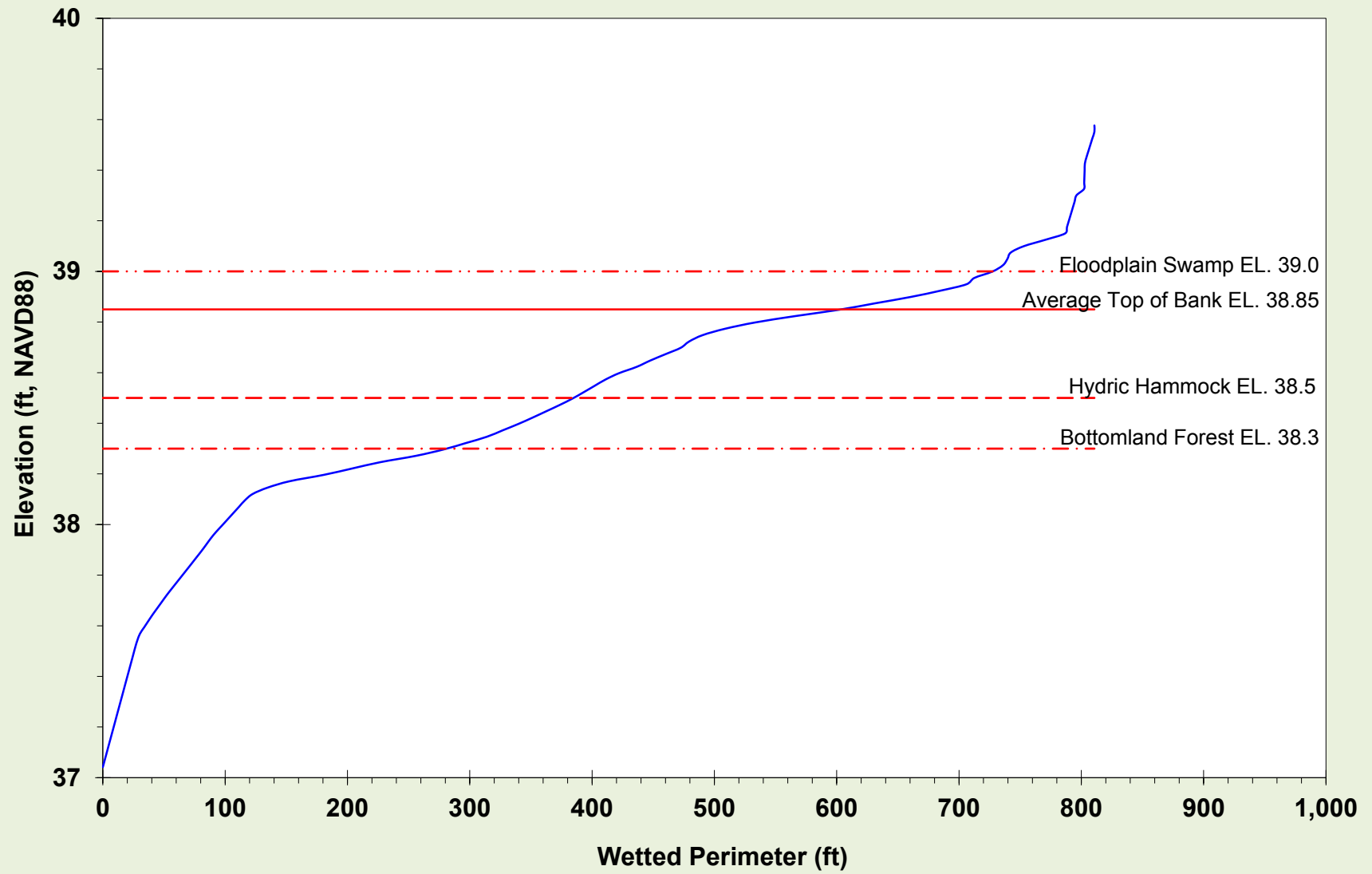
Figure 39. Wetted Perimeter for Transect 11
