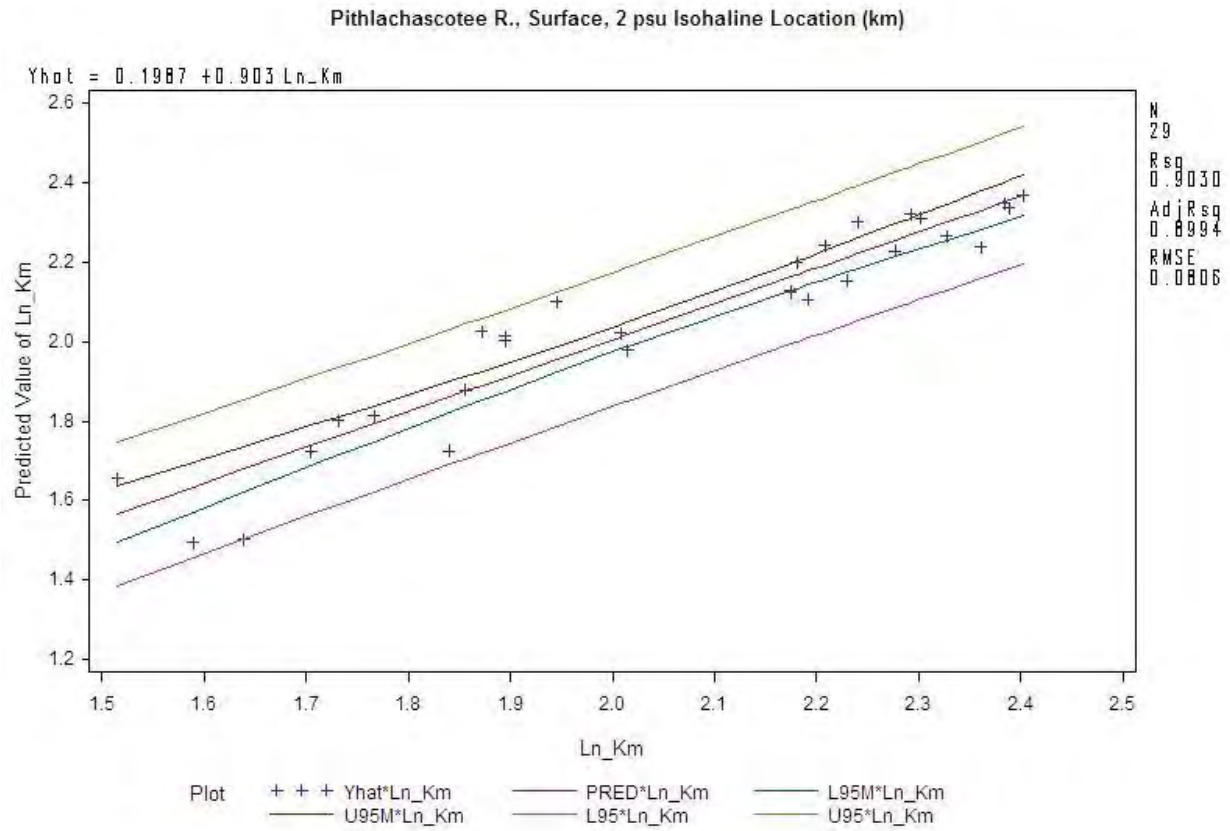
Figure 4B 09. Comparison between model predicted and observed isohaline position (as natural log RKm) for Pithlachascotee River, 2 psu, surface isohaline.
