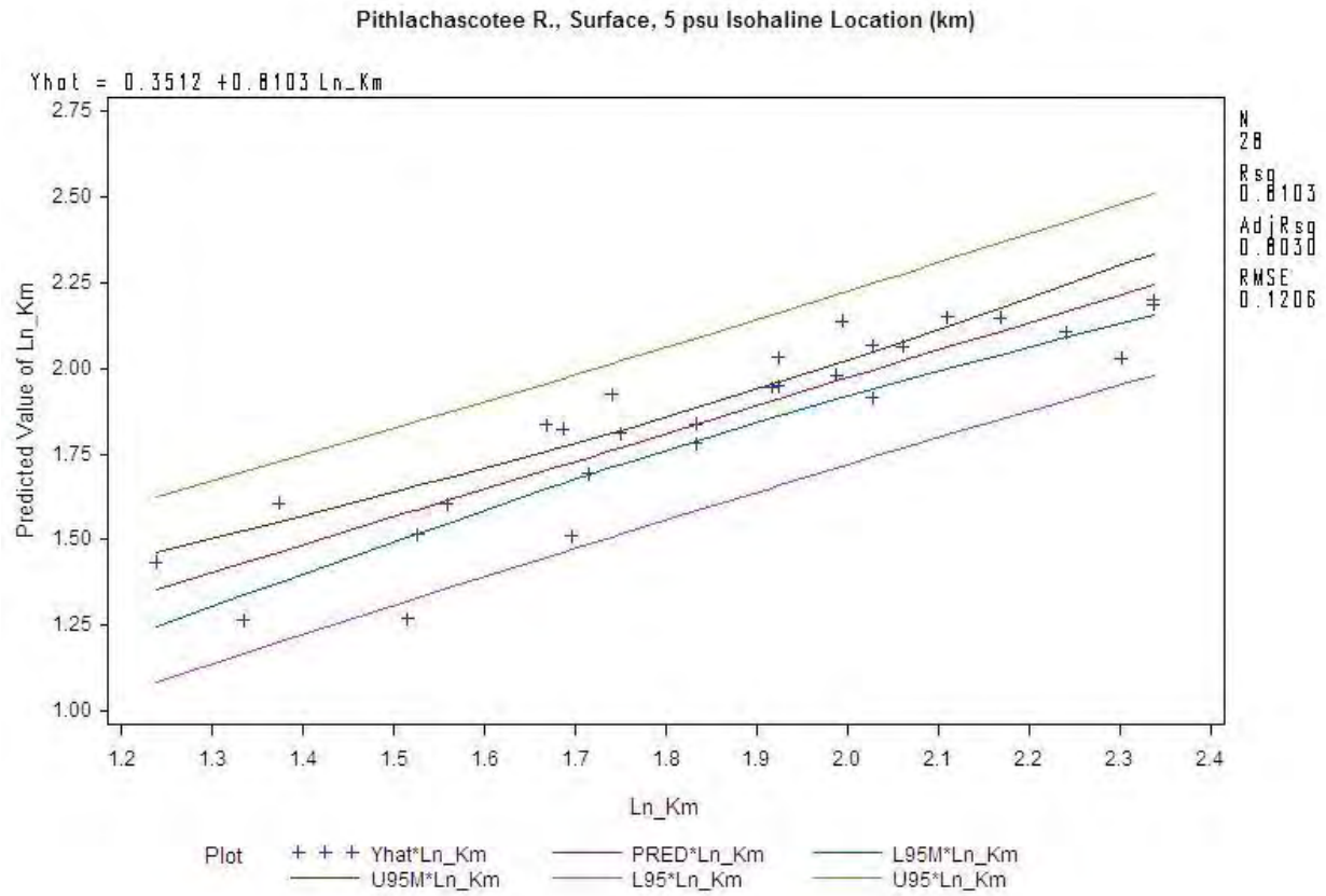
Figure 4B 10. Comparison between model predicted and observed isohaline position (as natural log RKm) for Pithlachascotee River, 5 psu, surface isohaline.
