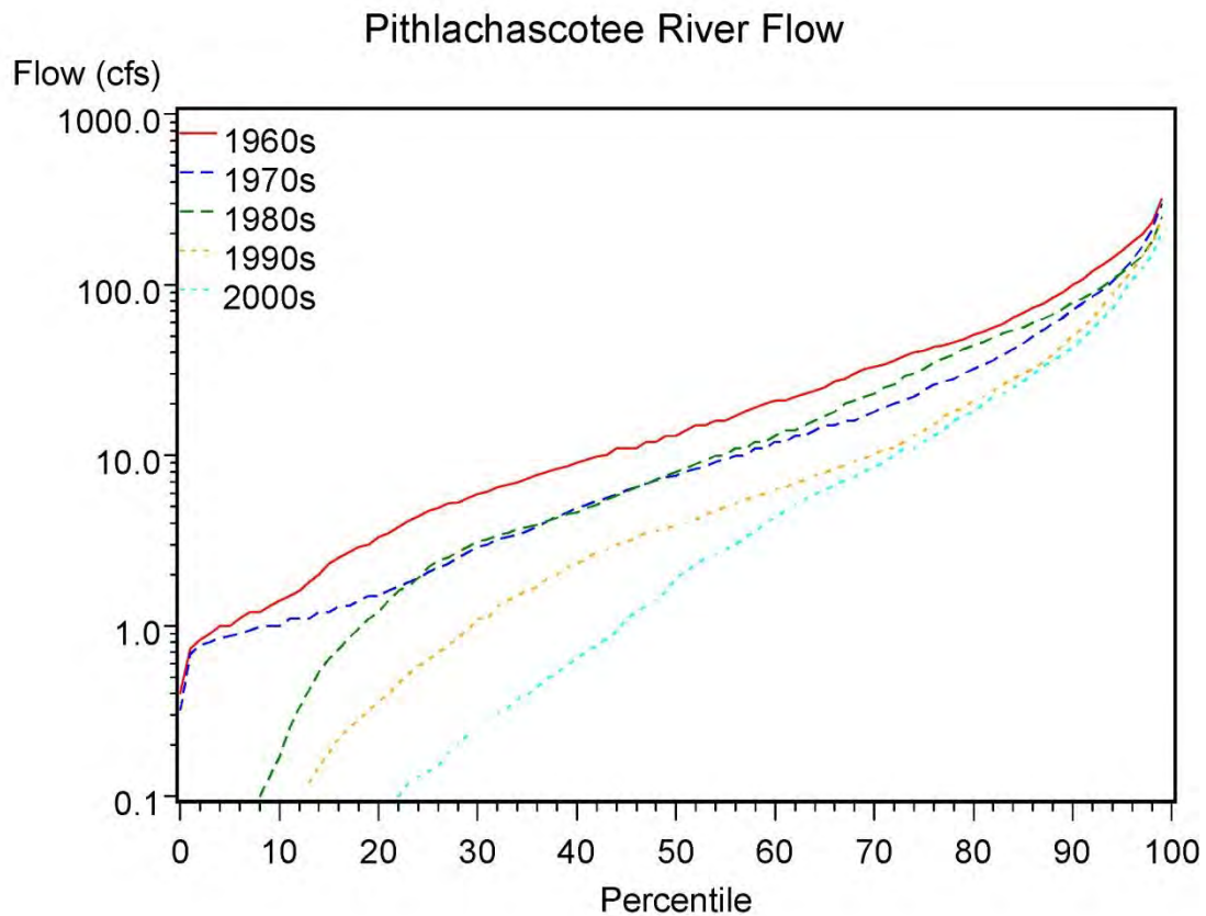
Figure 2-1. Pithlachascotee River flow duration curves by decade.
