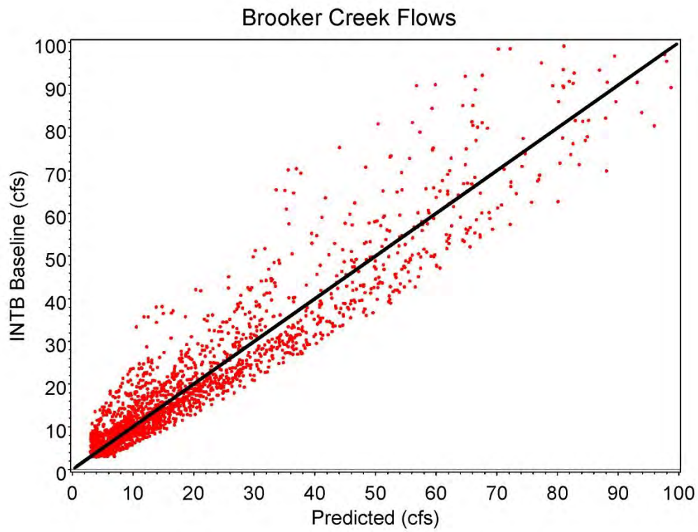
Figure 3-4. Brooker Creek regression predictions versus INTB Baseline flows (0- 100 cfs).
