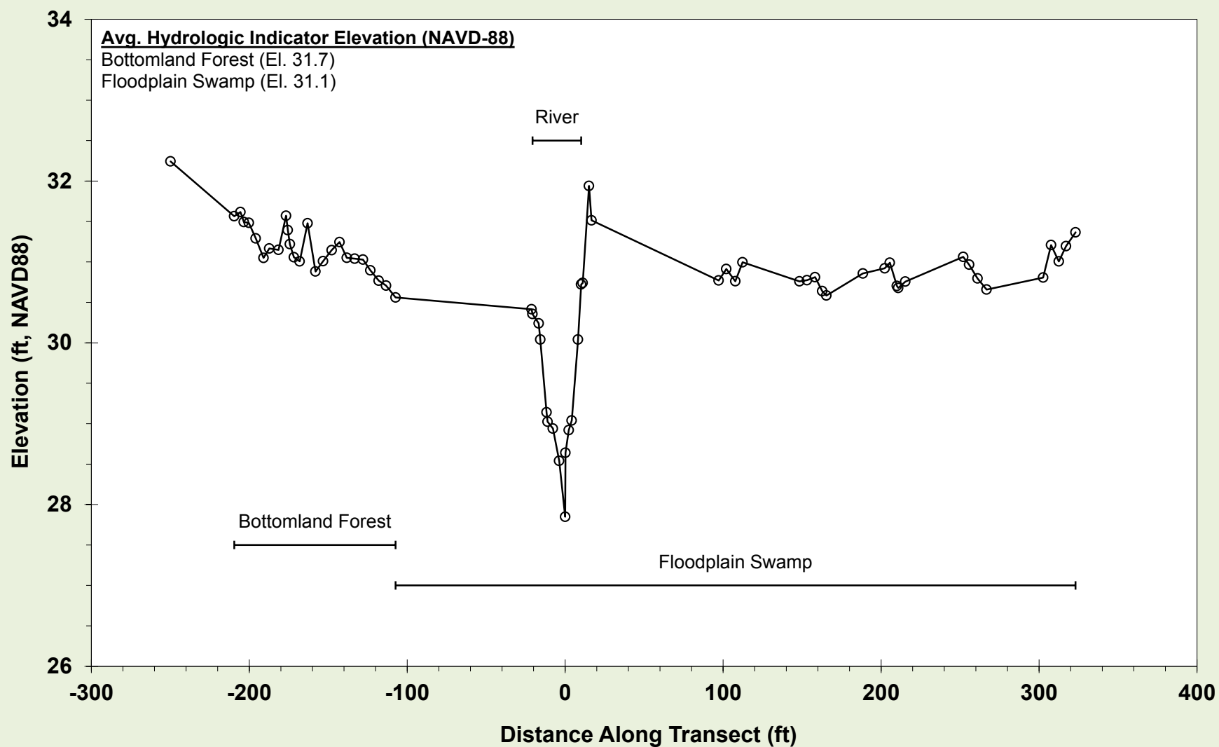
Figure 13. Pithlachascotee River, Transect 7
