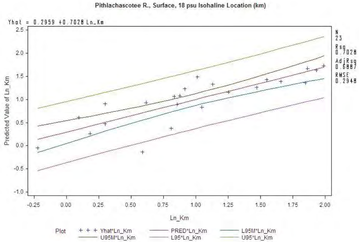
Figure 4B 12. Comparison between model predicted and observed isohaline position (as natural log RKm) for Pithlachascotee River, 18 psu, surface isohaline.
