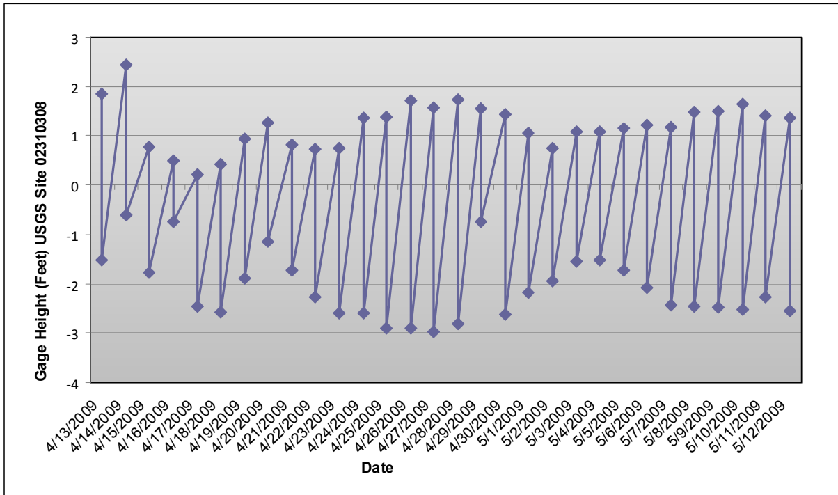
Figure 3.1.1-2. Gage height daily minim and maxima recorded for USGS flow station 02310308 near the mouth of the Pithlachascotee River.
