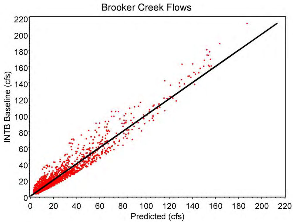
Figure 3-3. Brooker Creek regression predictions versus INTB Baseline flows.
