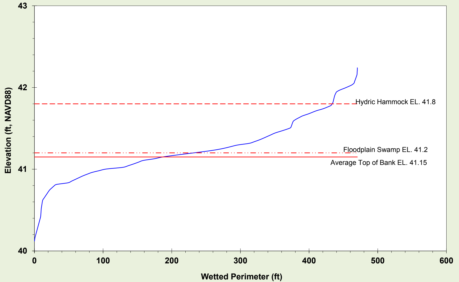
Figure 42. Wetted Perimeter for Transect 14
