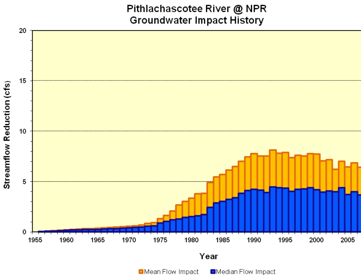
Figure 9. Projected mean and median annual stream flow impact to the Pithlachascotee River at New Port Richey gage due to groundwater withdrawals in the region (1955-2007).
