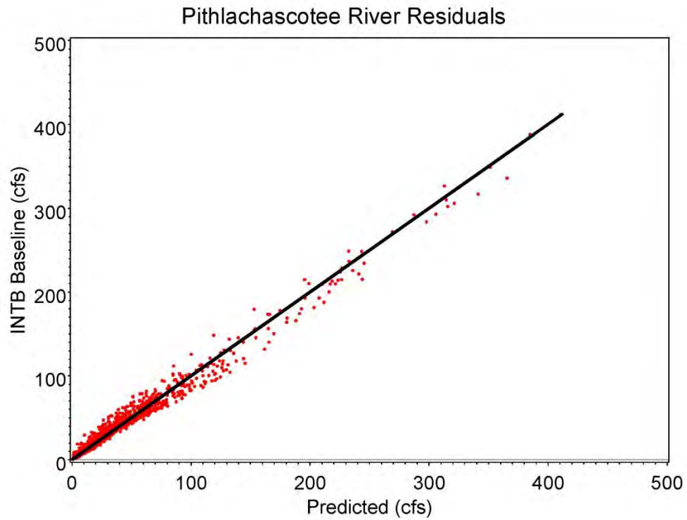
Figure 3-1. Pithlachascotee River regression predictions versus INTB Baseline flows.
