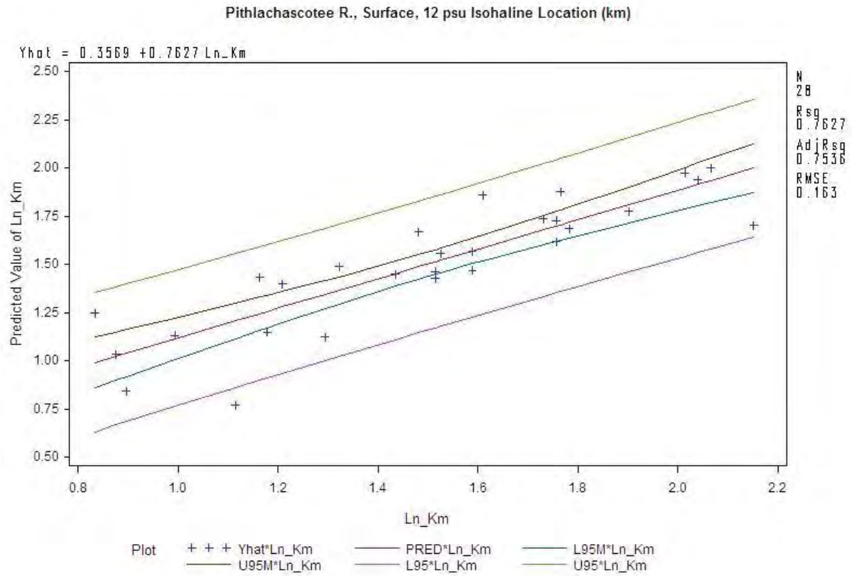
Figure 4B 11. Comparison between model predicted and observed isohaline position (as natural log RKm) for Pithlachascotee River, 12 psu, surface isohaline.
