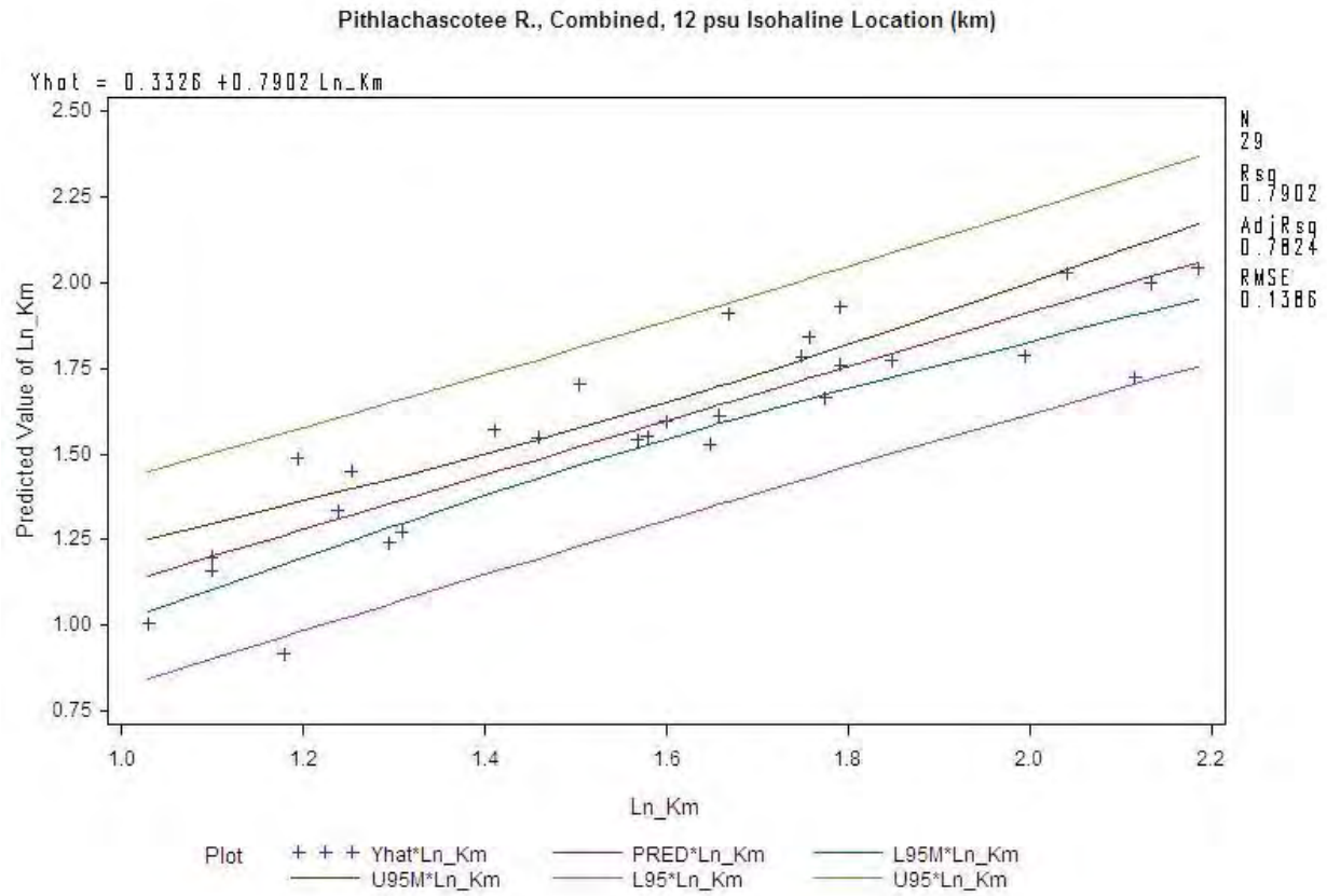
Figure 4B 07. Comparison between model predicted and observed isohaline position (as natural log RKm) for Pithlachascotee River, 12 psu, combined water column isohaline.
