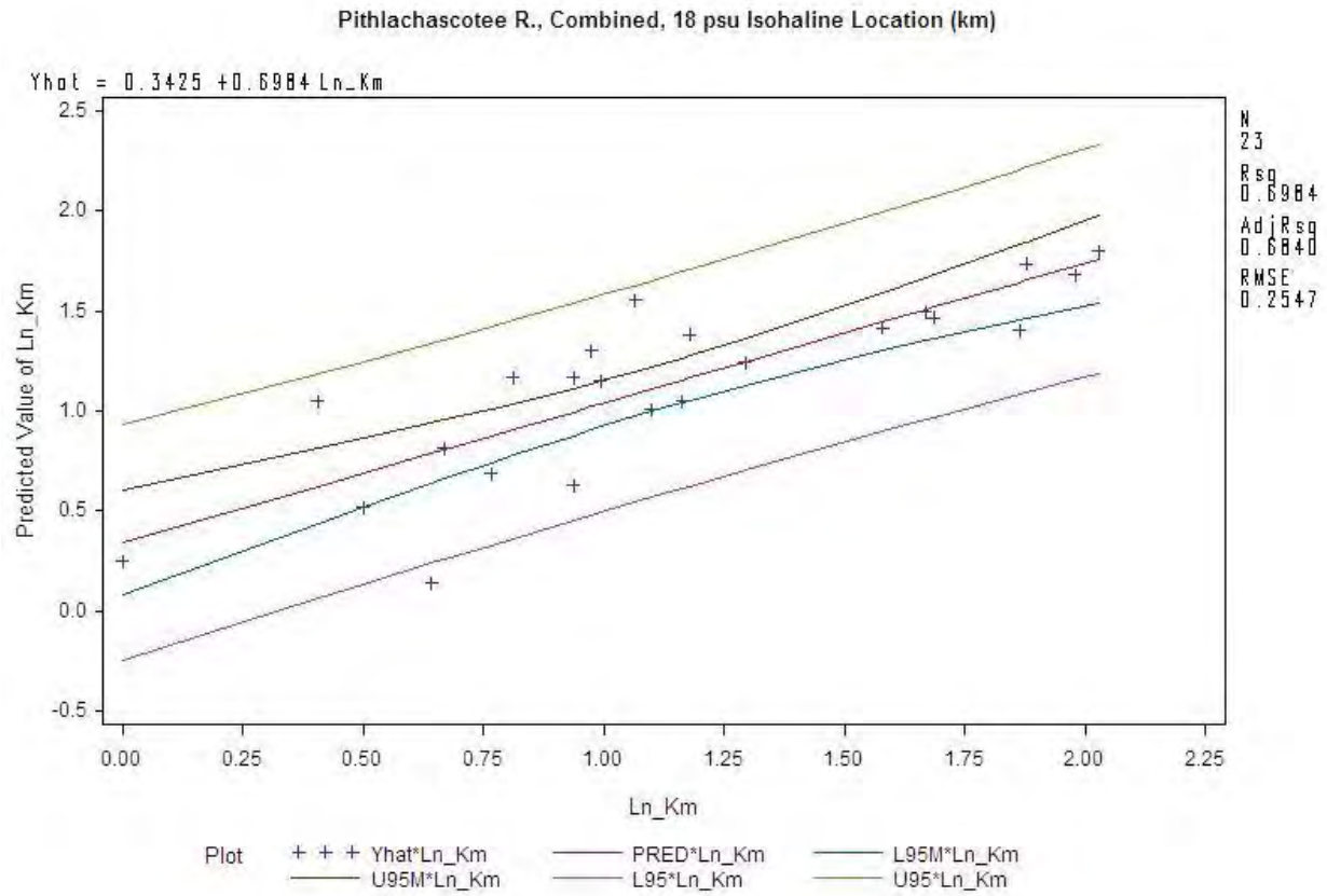
Figure 4B 08. Comparison between model predicted and observed isohaline position (as natural log RKm) for Pithlachascotee River, 18 psu, combined water column isohaline.
