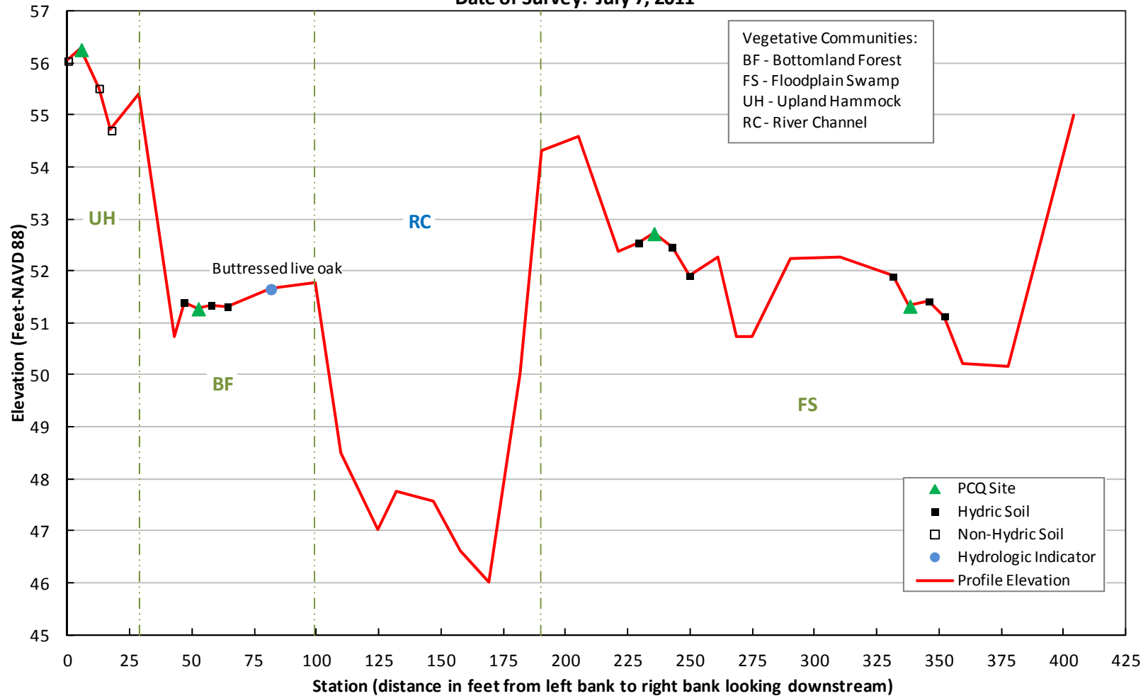
Figure C-3. Elevation profile for Horse Creek transect 3
