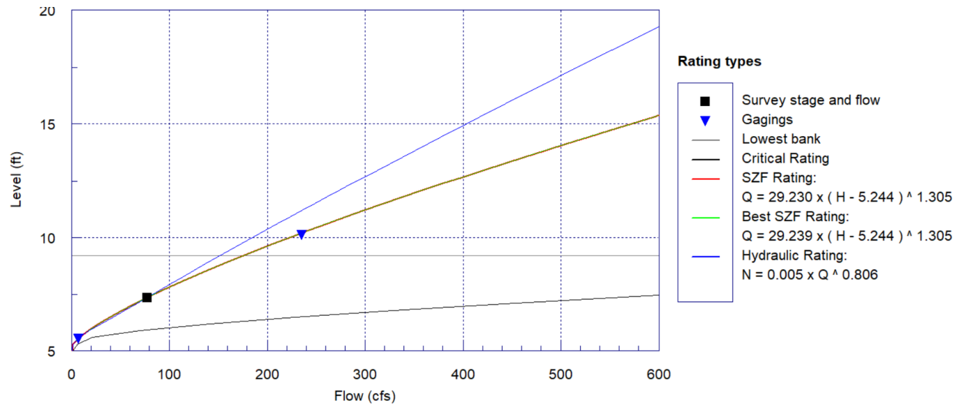
Figure m. Shoal Transect Rating Curve
