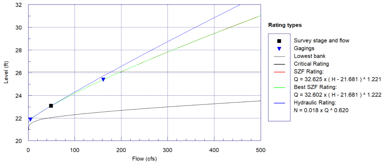
Figure g. Shoal Transect Rating Curve
