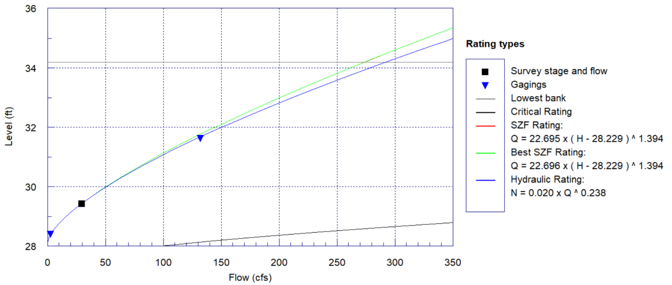
Figure e. Run Transect Rating Curve
