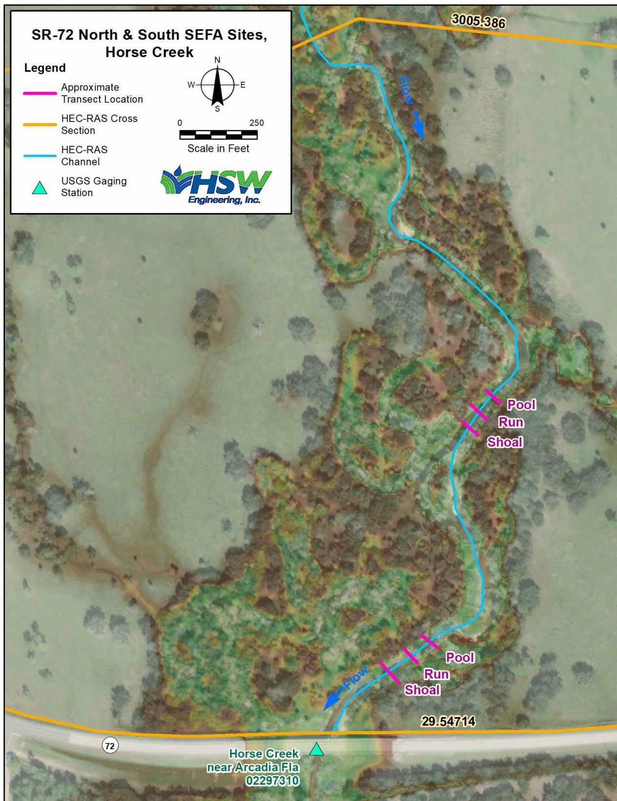
Figure 9. SR-72N and SR-72S Sites transects
