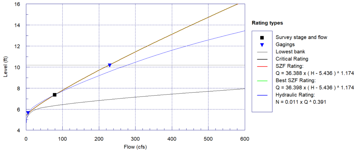
Figure n. Run Transect Rating Curve
