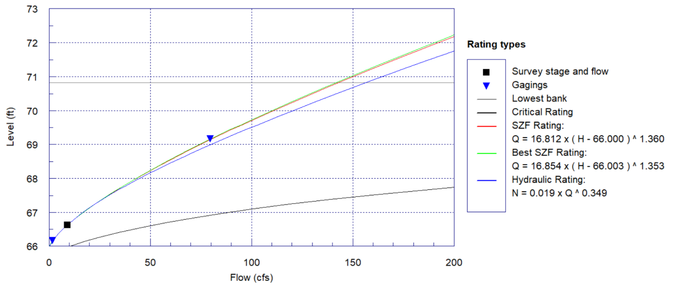
Figure b. Run Transect Rating Curve
