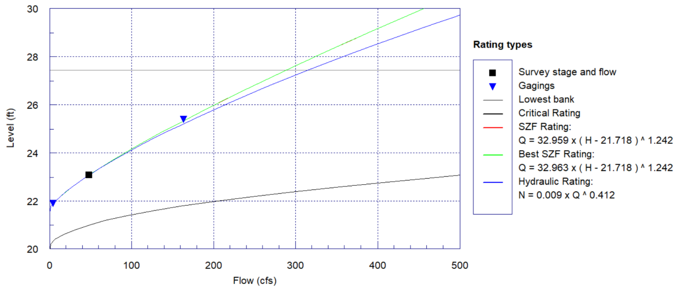
Figure h. Run Transect Rating Curve
