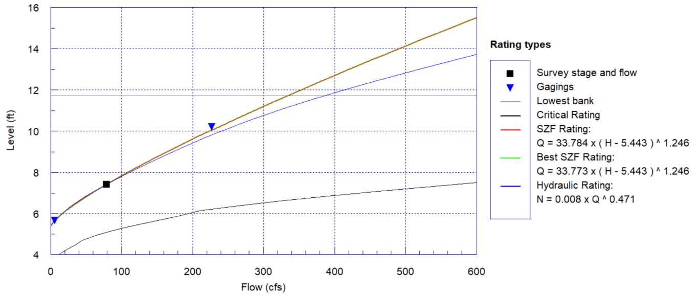
Figure o. Pool Transect Rating Curve
