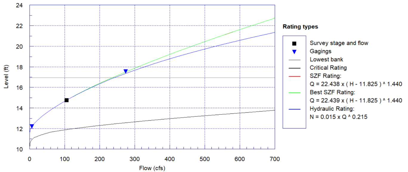
Figure k. Run Transect Rating Curve
