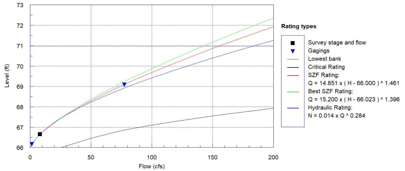
Figure c. Pool Transect Rating Curve
