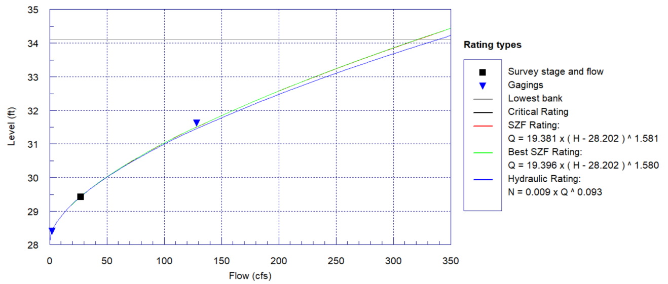
Figure f. Pool Transect Rating Curve
