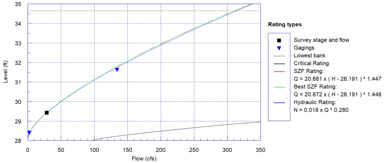
Figure d. Shoal Transect Rating Curve
