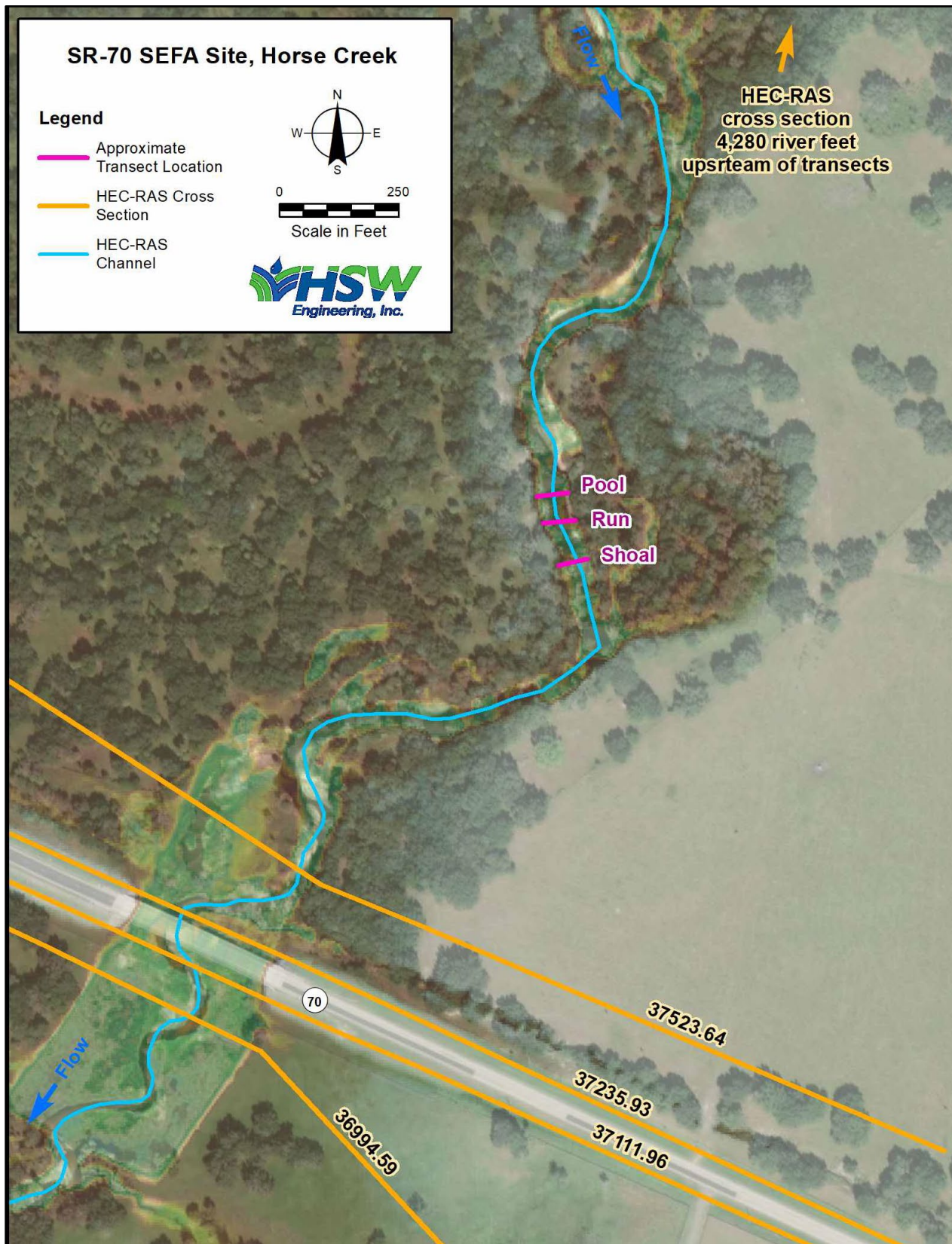
Figure 4. Site SR-70 Site transects
