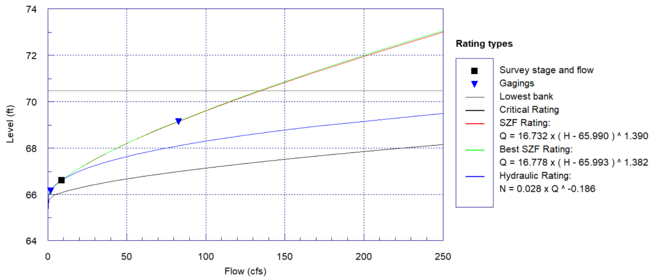
Figure a. Shoal Transect Rating Curve
