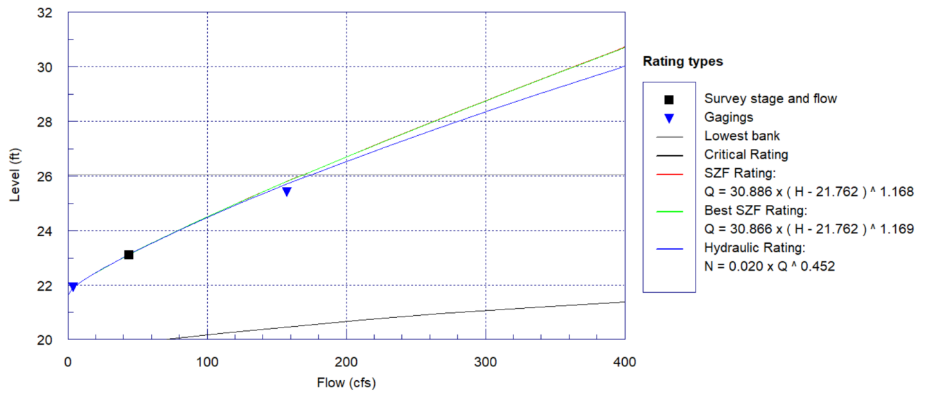
Figure i. Pool Transect Rating Curve
