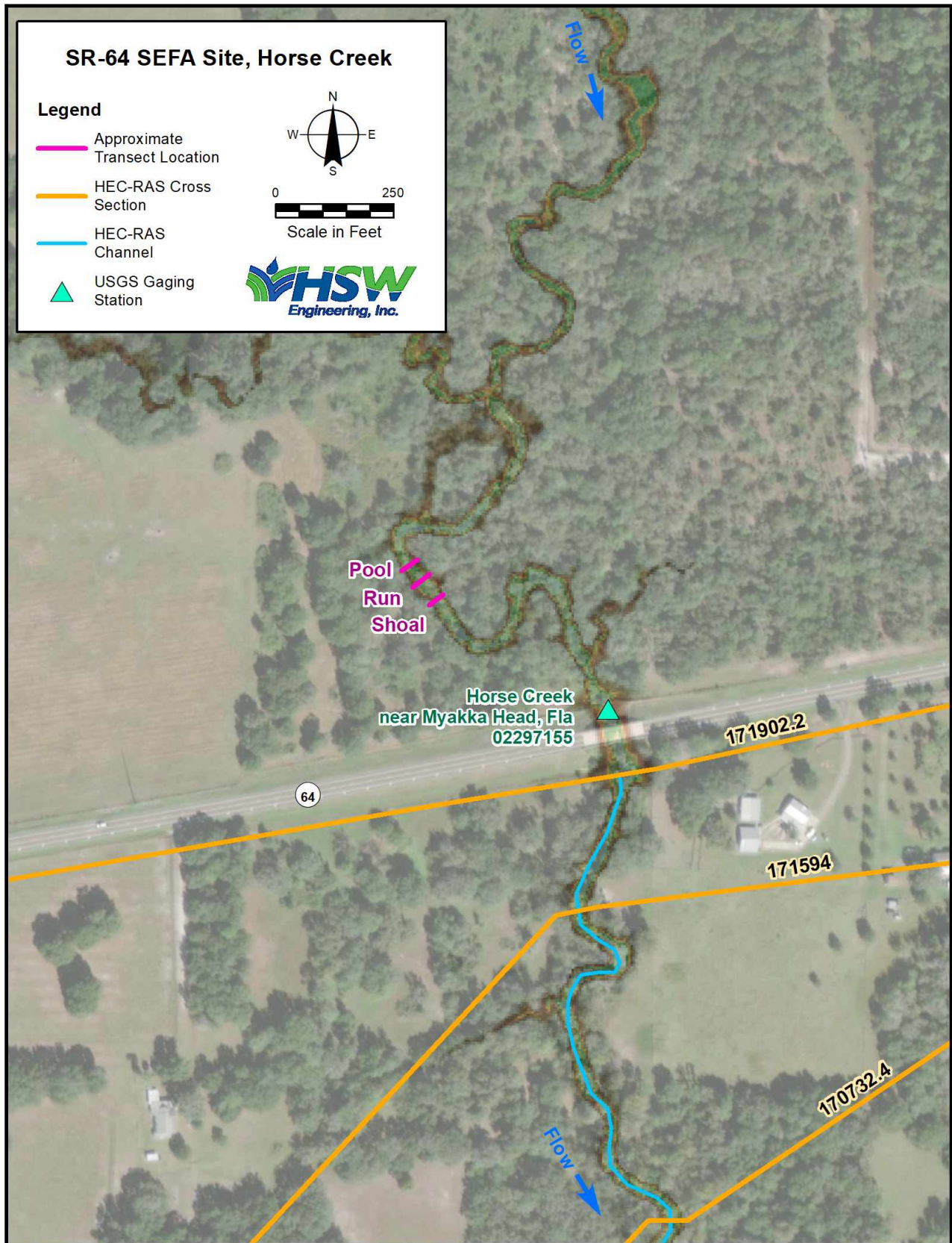
Figure 2. Site SR-64 Site transects
