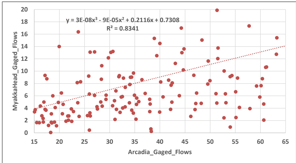
Figure 5. Arcadia vs. Myakka Head flows
