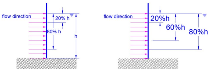
Figure 2. Two-point and three-point USGS methods.
