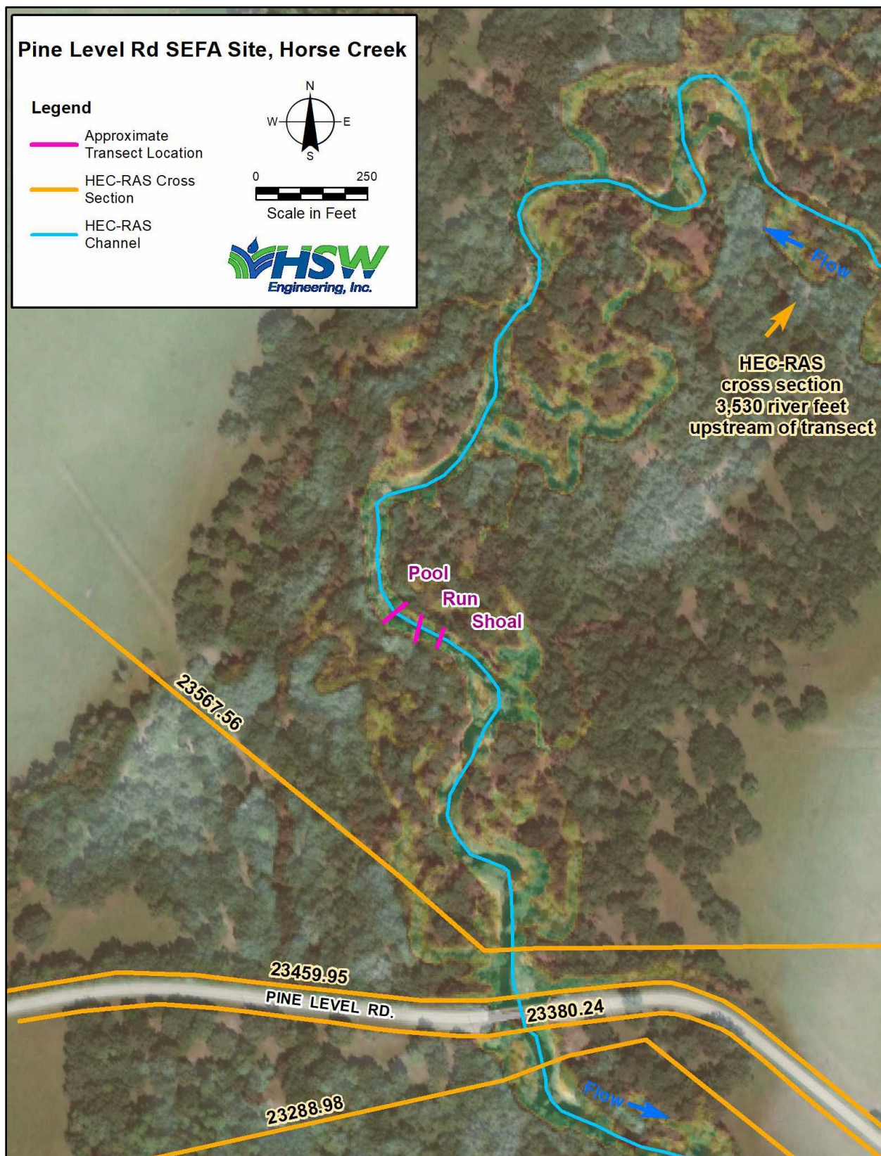
Figure 6. Pine Level Road Site transects
