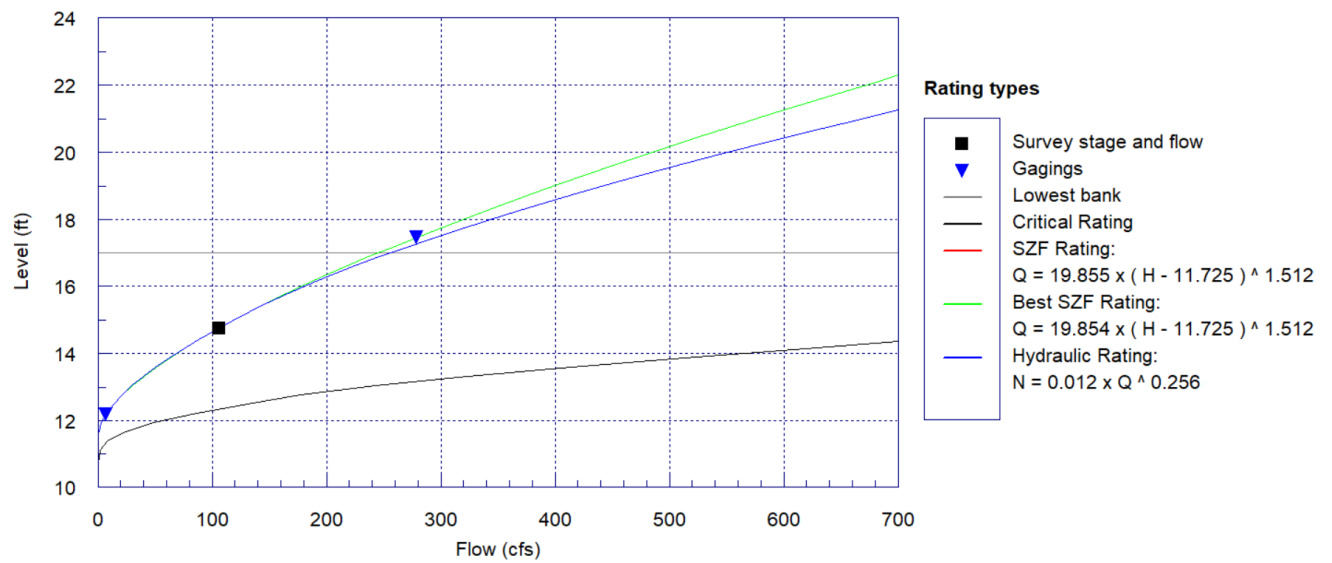
Figure j. Shoal Transect Rating Curve
