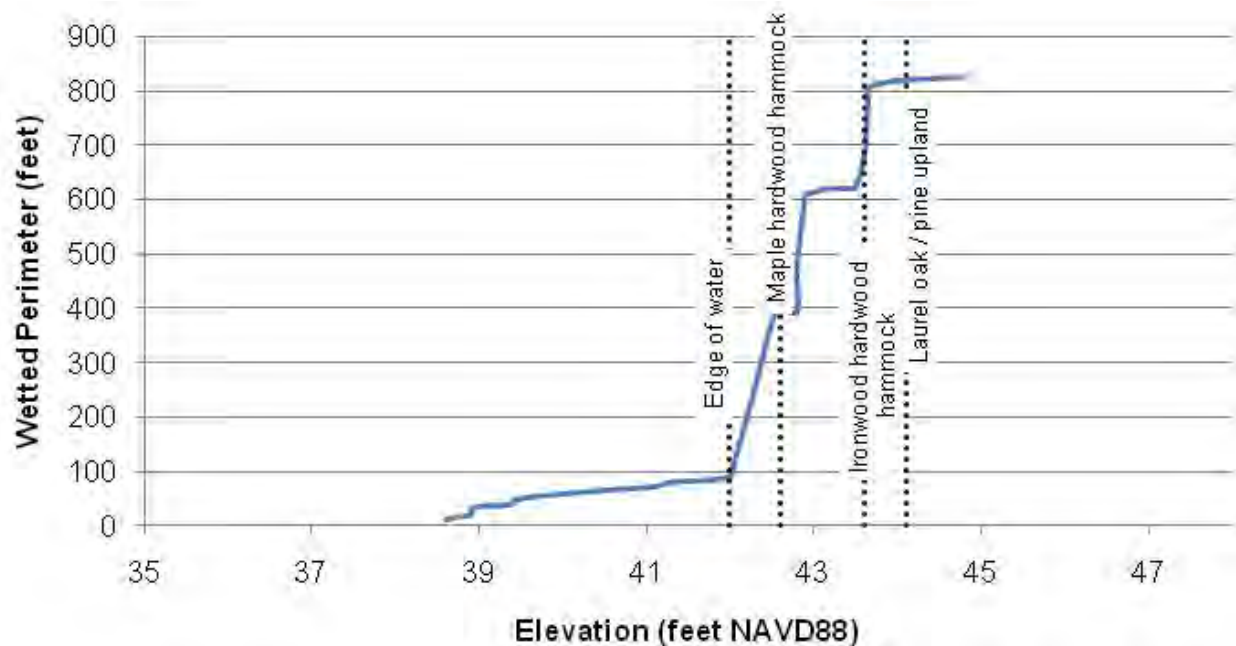
Figure 3-18 Wetted Perimeter and Median Vegetation Class Elevations along Transect 2
