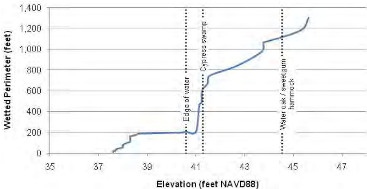
Figure 3-23 Wetted Perimeter and Median Vegetation Class Elevations along Transect 7
