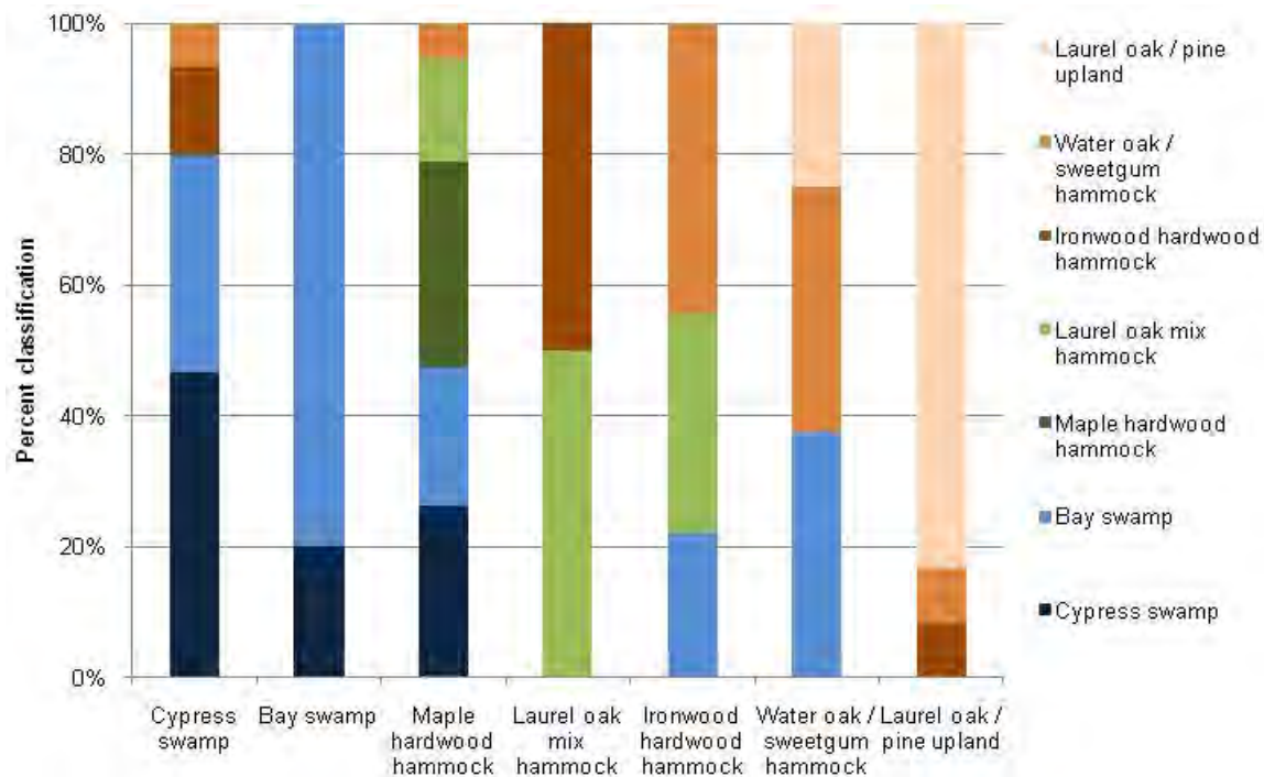
Figure 3-15 Percent Correct Classifications of Vegetation Classes
