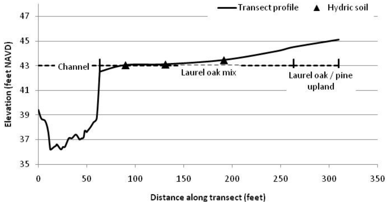
Figure 3-2 Elevation, Vegetation, and Hydric Soil Profile along Transect PHABSIM1
