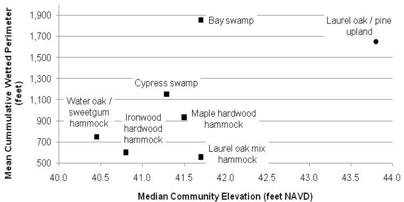
Figure 3-16 Mean Wetted Perimeter and Median Elevations Associated with Vegetation Classes
