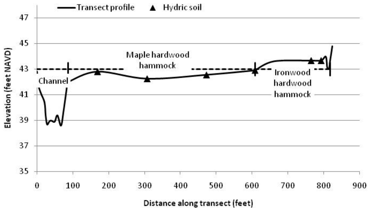
Figure 3-3 Elevation, Vegetation, and Hydric Soil Profile along Transect 2
