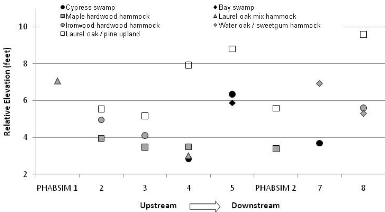
Figure 3-13 Median Relative Elevation (feet above channel bottom) of Vegetation Classes along the Gum Slough Transects
