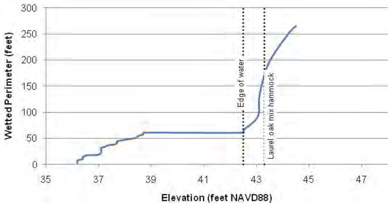
Figure 3-17 Wetted Perimeter and Median Vegetation Class Elevations along Transect PHABSIM1
