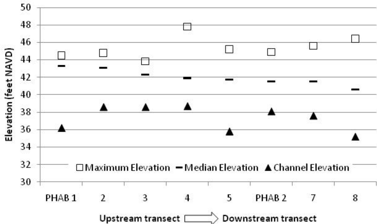
Figure 3-1 Channel Bottom, Maximum, and Median Elevations along Gum Slough Transects
