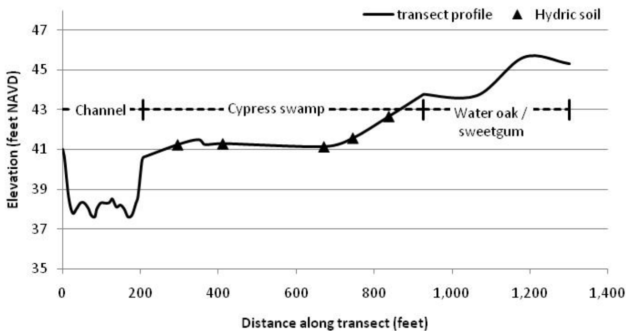
Figure 3-8 Elevation, Vegetation, and Hydric Soil Profile along Transect 7
