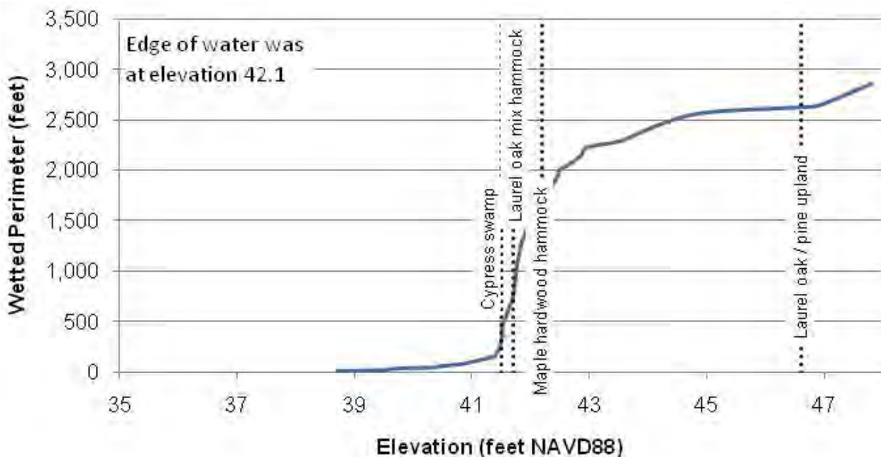
Figure 3-20 Wetted Perimeter and Median Vegetation Class Elevations along Transect 4
