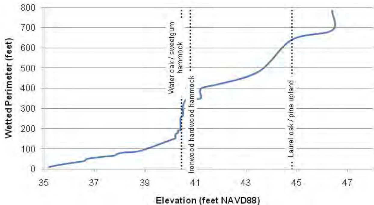
Figure 3-24 Wetted Perimeter and Median Vegetation Class Elevations along Transect 8
