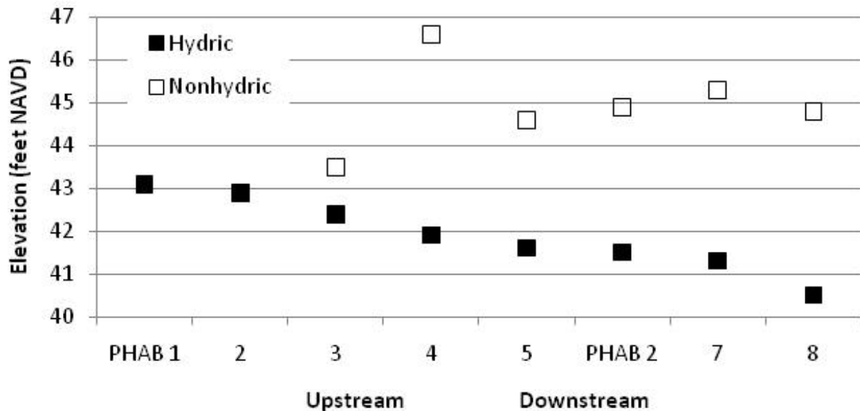
Figure 3-10 Median Elevations of Hydric and Nonhydric Soils along Gum Slough Transects
