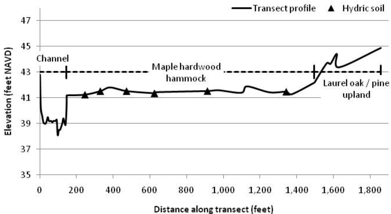
Figure 3-7 Elevation, Vegetation, and Hydric Soil Profile along Transect PHABSIM2
