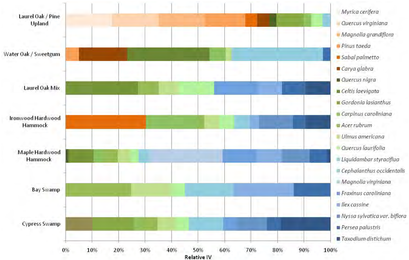
Figure 3-11 Importance Values for Tree Species in Vegetation Classes along the Gum Slough Transects
