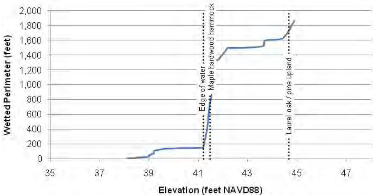
Figure 3-22 Wetted Perimeter and Median Vegetation Class Elevations along Transect PHABSIM2
