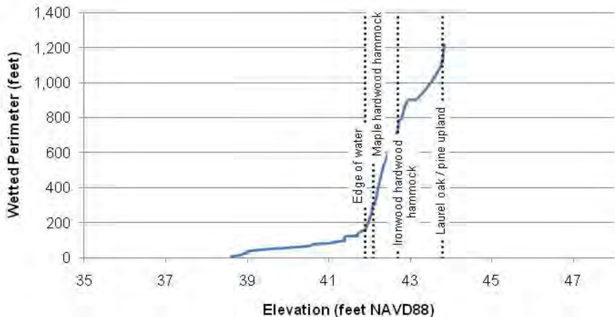
Figure 3-19 Wetted Perimeter and Median Vegetation Class Elevations along Transect 3
