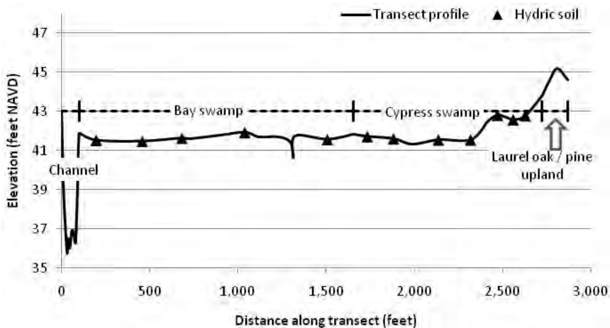
Figure 3-6 Elevation, Vegetation, and Hydric Soil Profile along Transect 5
