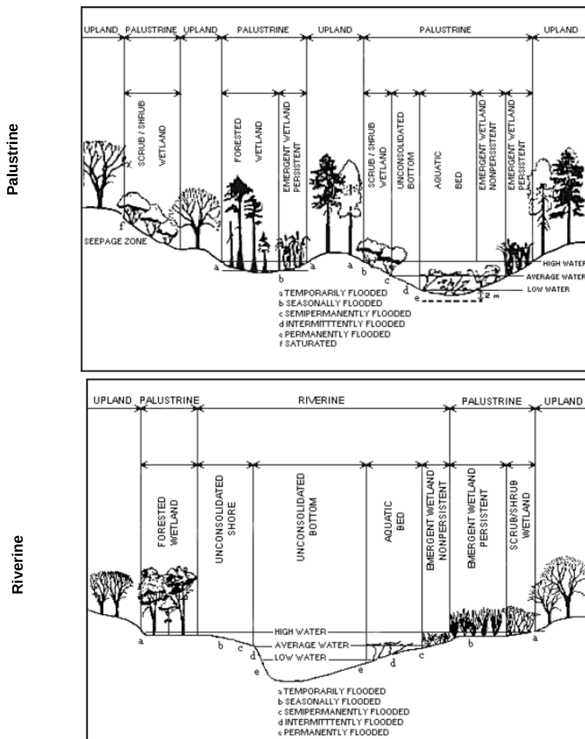
Figure 2-1 Features and Examples of Habitats in the Palustrine and Riverine Systems*
