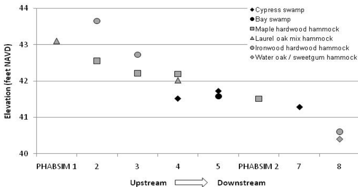
Figure 3-14 Median Elevations (feet NAVD) of Hydric Soils by Vegetation Class along the Gum Slough Transects
