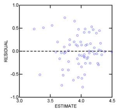
Plot of residuals against predicted values
