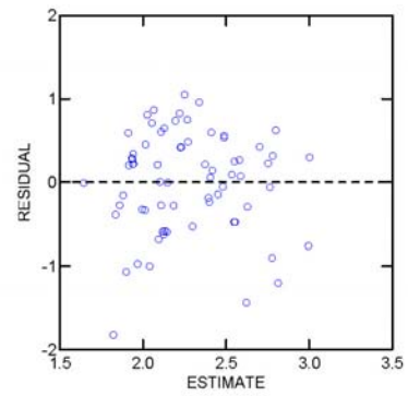
Plot of residuals against predicted values
