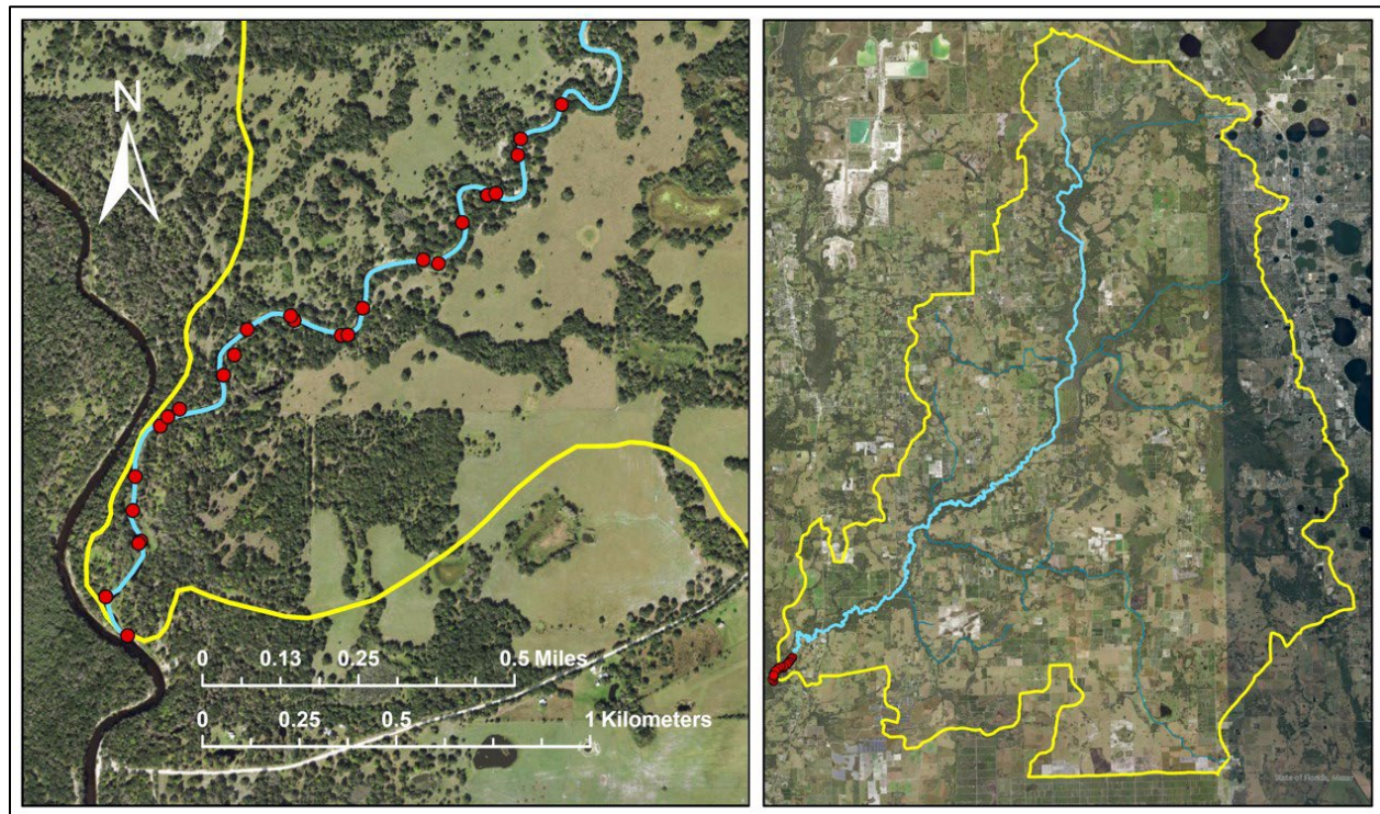
Figure 4-2. Electrofishing sample locations by the FWC (Call et al. 2011; left) with their location relative to the entire Charlie Creek system and watershed (yellow outline; right).
