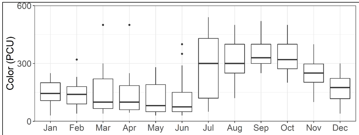
Figure 3-14: Monthly distribution of mean color at DEP station 21FLGW 3561 from 1998-2017. Boxed values indicate the 25 th to 75 th percentiles with centerline reflecting the 50 th percentile value. Dots represent outliers, indicative of values outside of the 1.5*interquartile range.
