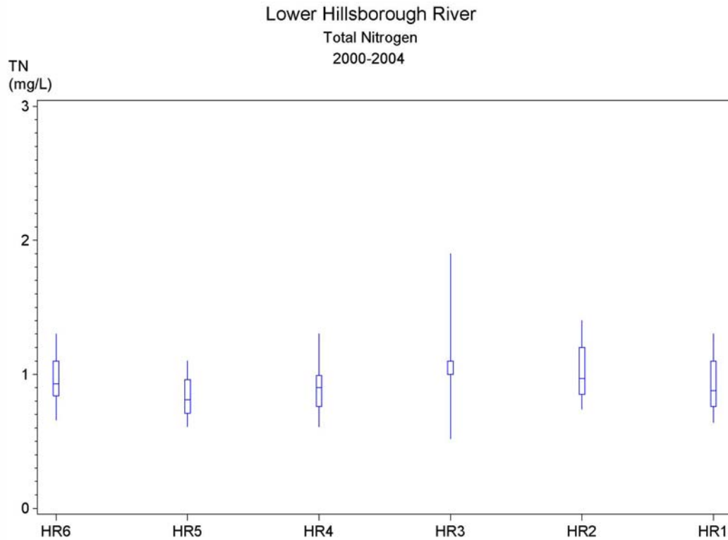
Figure 4-23 Observed longitudinal distributions of total nitrogen for the Tampa Bay Water HBMP program period of record.
