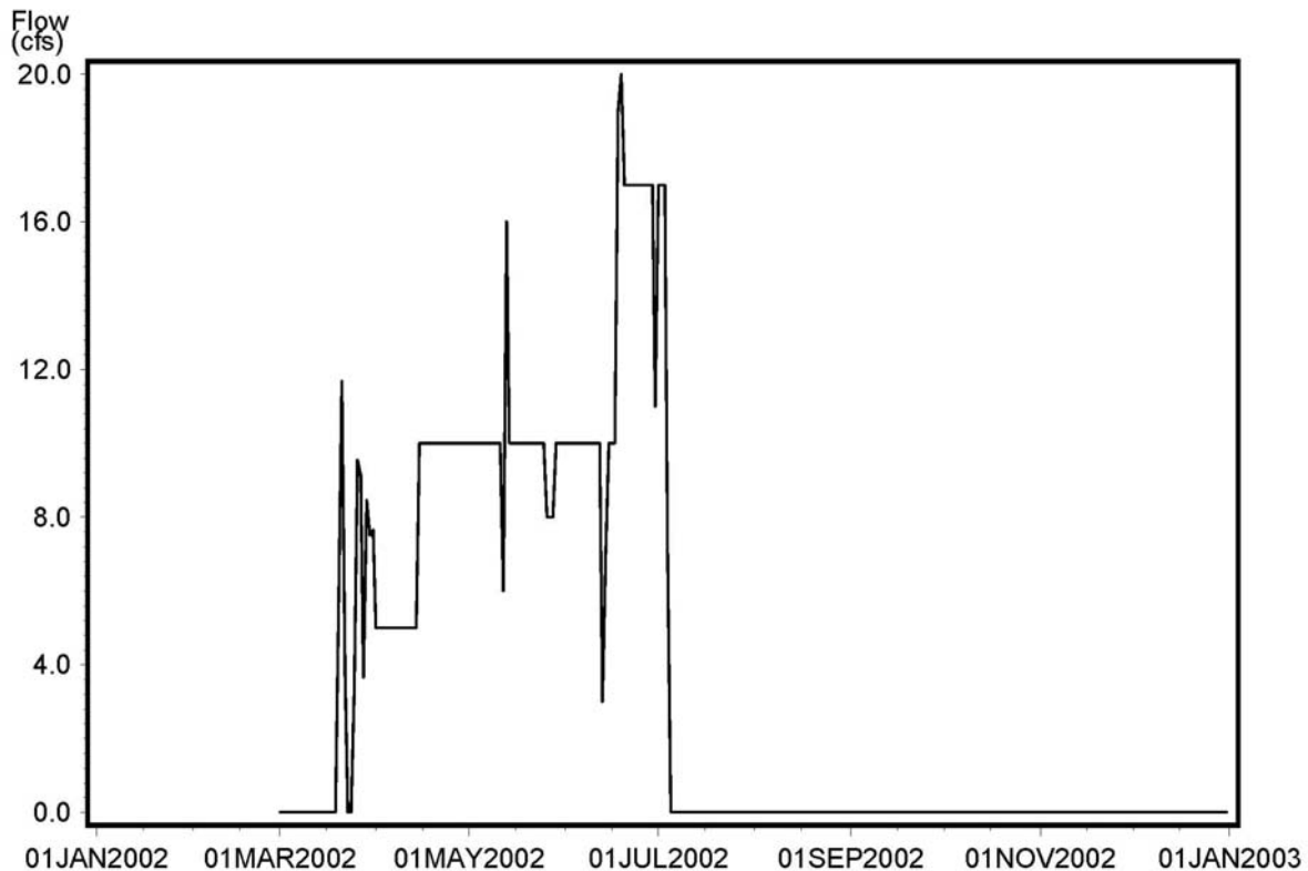
Figure 2-15 Time series of daily Sulphur Springs diversions to the base of the dam for MFL compliance.
