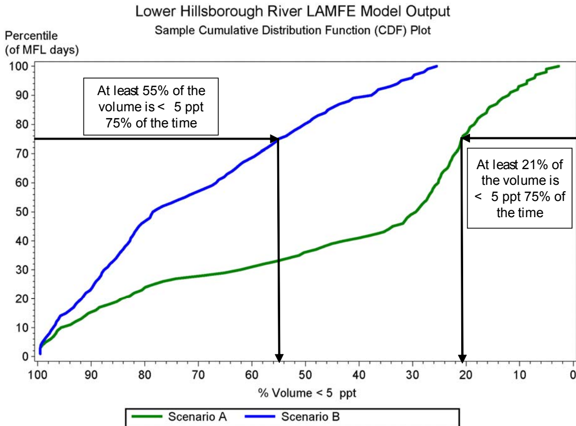
Figure 7-1b Example CDF plot. See discussion above.
