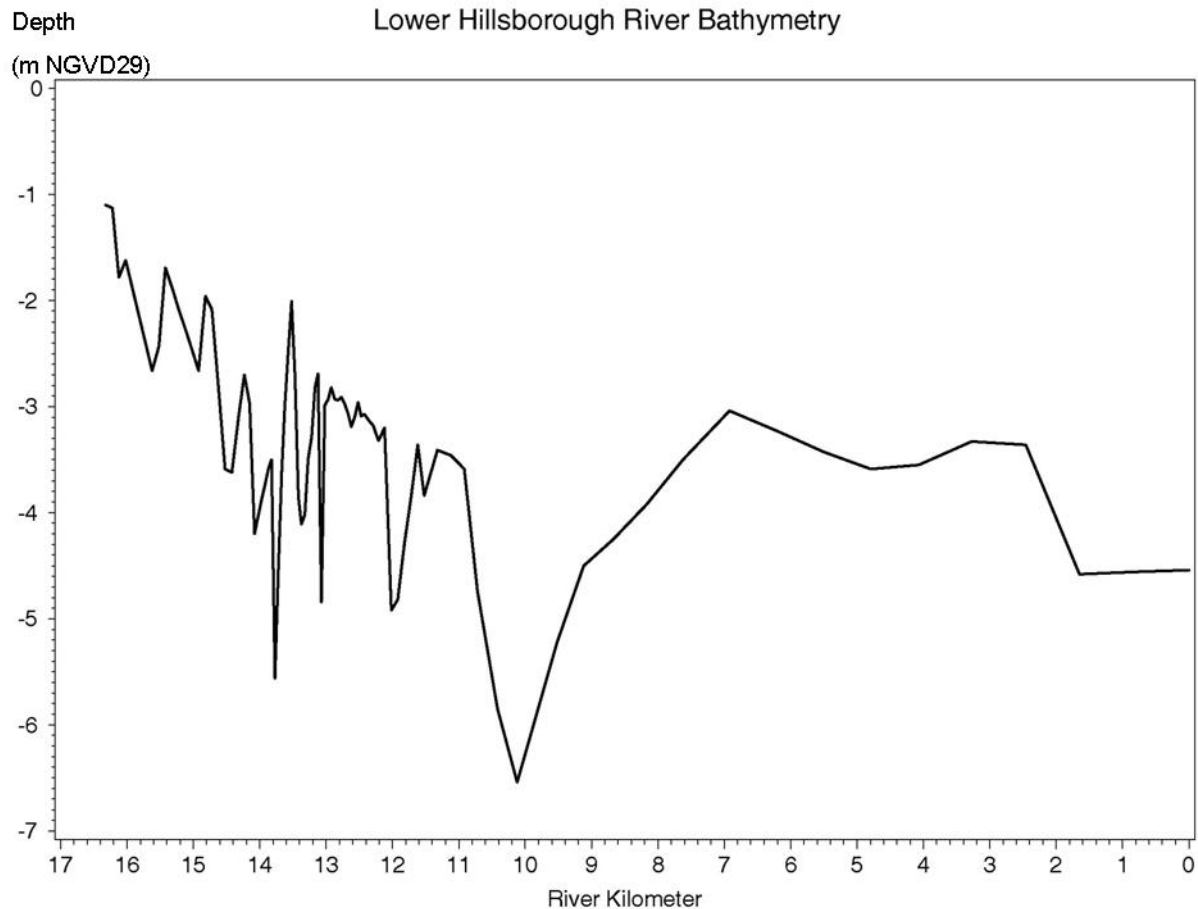
Figure 3-2 Longitudinal representation of bottom depths in the LHR. RKM16=Hillsborough River Dam; RKM0=mouth of the river.
