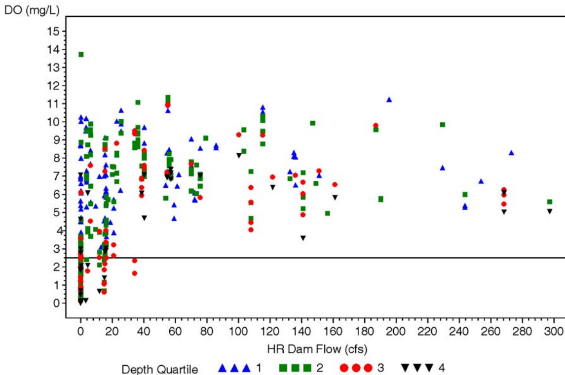
Figure 6-21 Bottom DO between Km 14 and the dam as a function of dam flow and depth for flows between 0 and 300 cfs. Symbols are categorized by depth quartiles based on bottom area bathymetry for this region of the river.
