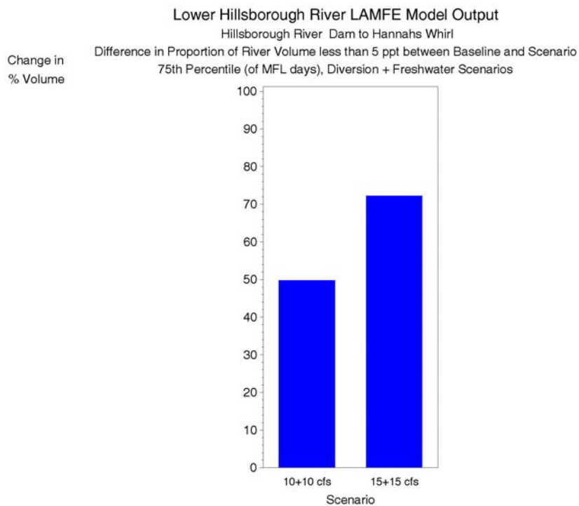
Figure 7-46 Difference in the proportion of volume less than 5 ppt between the baseline and Hannah's Whirl for the diversion scenarios (scenario - baseline), 75 th percentile of MFL days.
