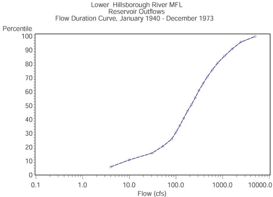
Figure 2-11 Flow duration curve of outflows from the Hillsborough River Reservoir, 1940-1973.
