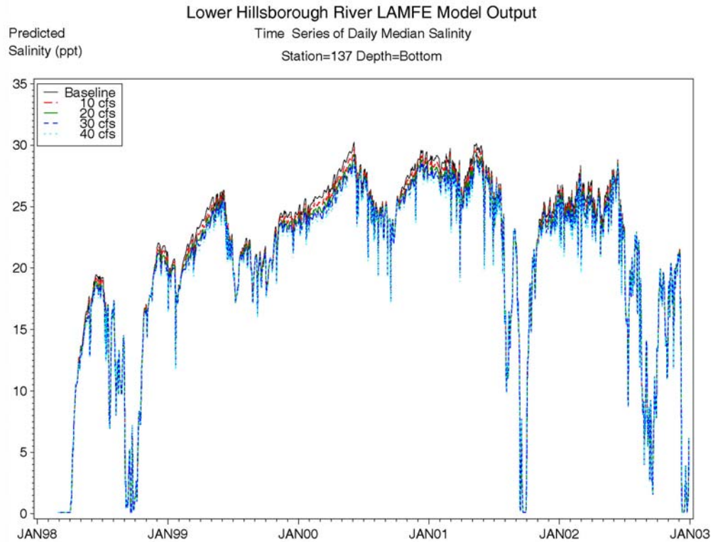
Figure 6-56 Predicted daily median salinity for the baseline and freshwater scenarios at EPCHC station 137, bottom layer.
