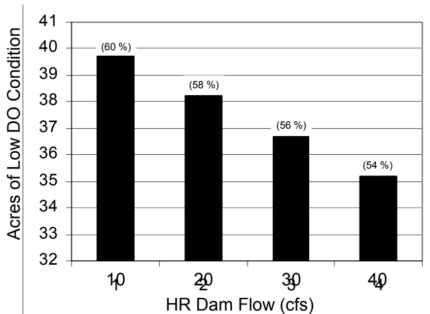
Figure 6-28 Acres of bottom DO<2.5 mg/L between Km 10 and 14 as a function of dam flow. Corresponding percent of bottom habitat in this region of the river indicated in parentheses.
