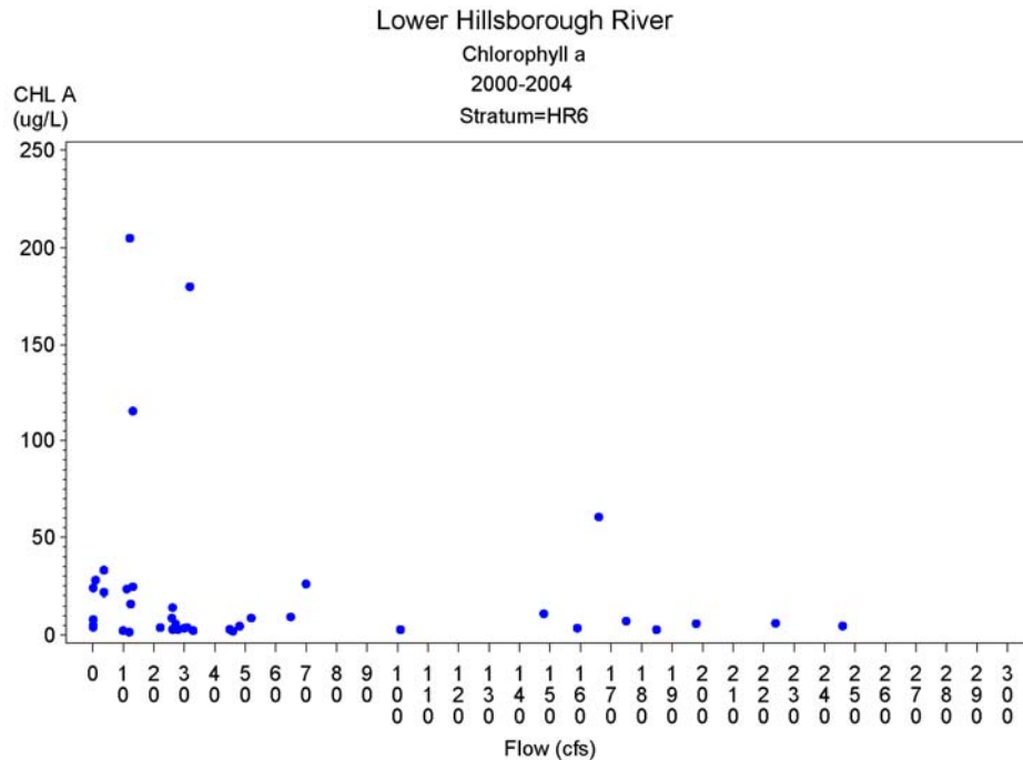
Figure 6-38 Observed response of Chlorophyll a concentrations to total freshwater inflow in Tampa Bay Water HBMP Monitoring Program Stratum 6. Data subset to flows less than 300 cfs for this figure.
