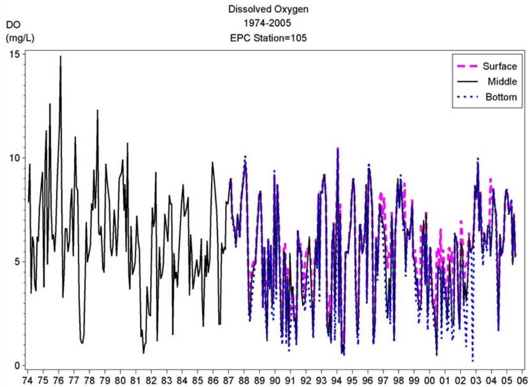
Figure 4-4 Monthly time series of surface and bottom DO at EPCHC Station 105 (near Rowlett Park).
