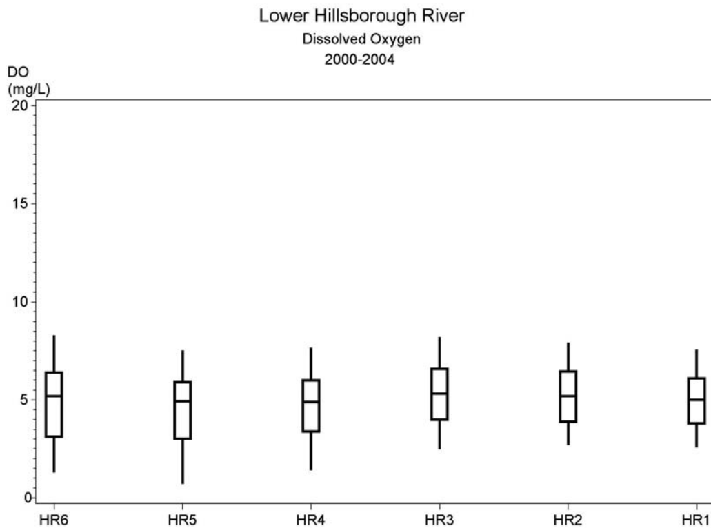
Figure 4-21 Observed longitudinal distributions of DO for the Tampa Bay Water HBMP program period of record.
