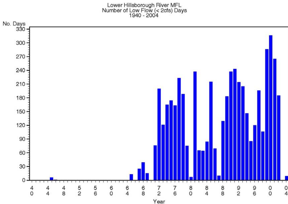
Figure 2-8 Hillsborough River Dam low flow (< 2 cfs) days by year, 1940-2004.
