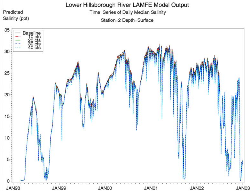
Figure 6-57 Predicted daily median salinity for the baseline and freshwater scenarios at EPCHC station 2, surface layer.
