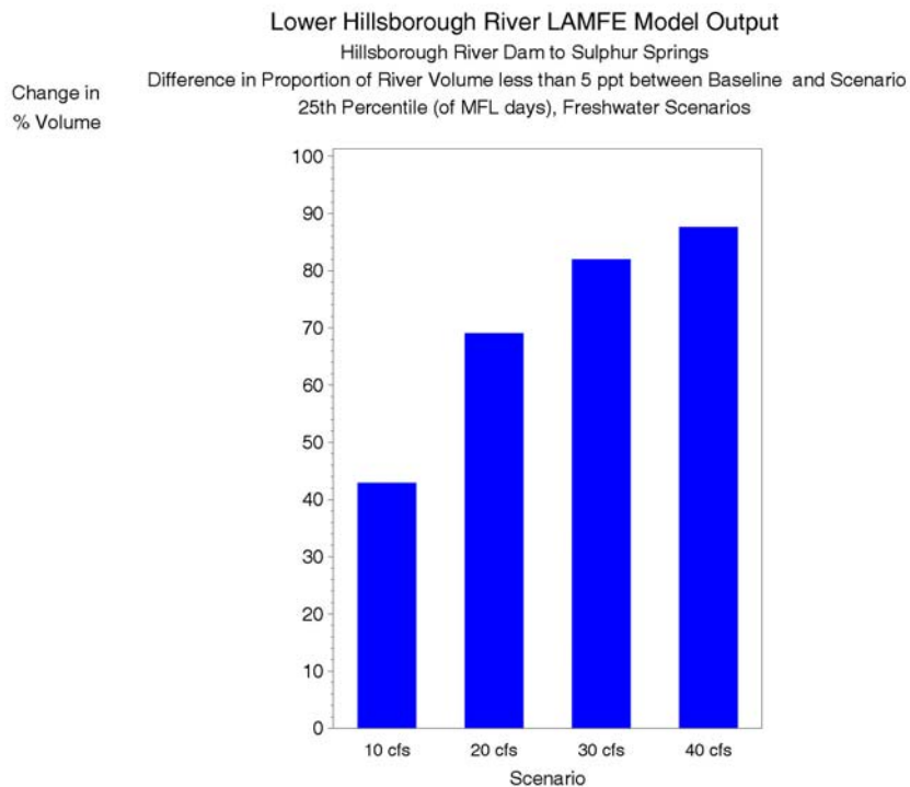
Figure 7-2 Difference in the proportion of volume less than 5 ppt between the baseline and freshwater Scenarios (Scenario - Baseline), 25 th percentile of MFL days, Dam to Sulphur Springs.
