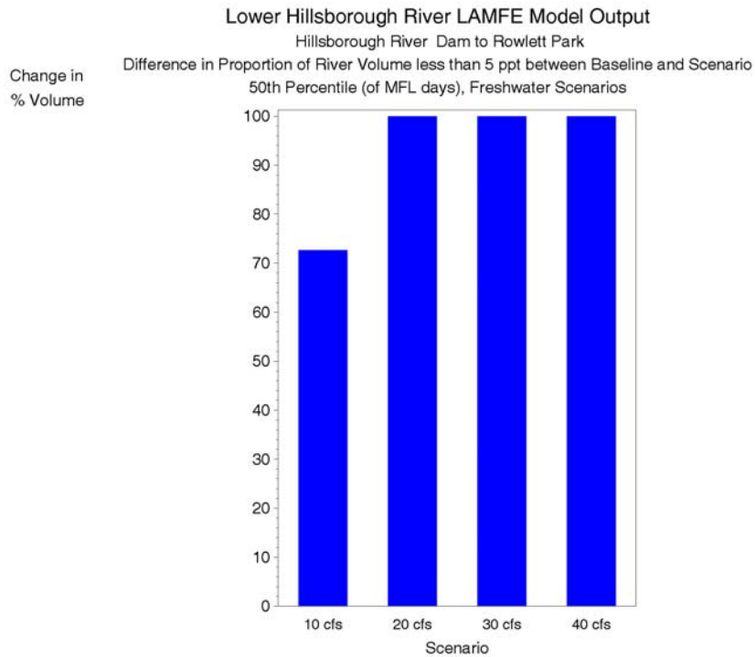
Figure 7-9 Difference in the proportion of volume less than 5 ppt between the baseline and freshwater Scenarios (Scenario - Baseline), 50 th percentile of MFL days, Dam to Rowlett Park.
