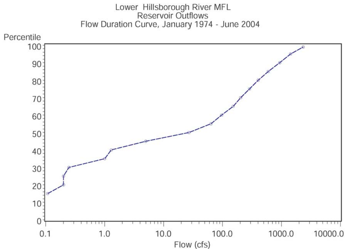
Figure 2-10 Flow duration curve of outflows from the Hillsborough River Reservoir, 1974-2004.
