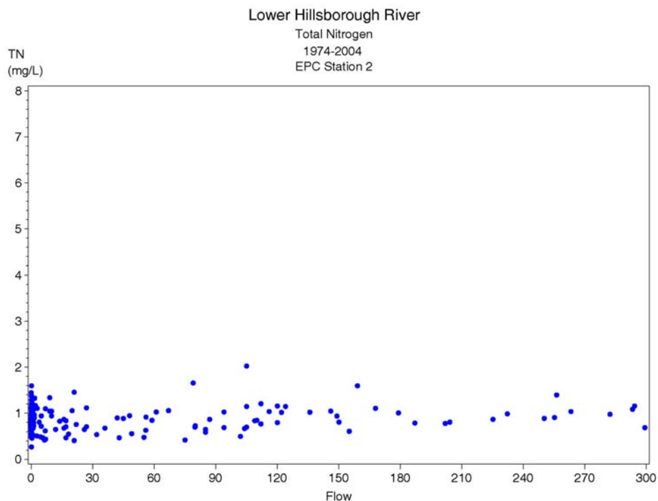
Figure 6-41. Observed response of total nitrogen concentration at EPC Station 2 as a function of flow at the Hillsborough River Dam (Dam flow + Sulphur Springs diversions to the base of the dam). Data were subset to flows less than 300 cfs for this figure.
