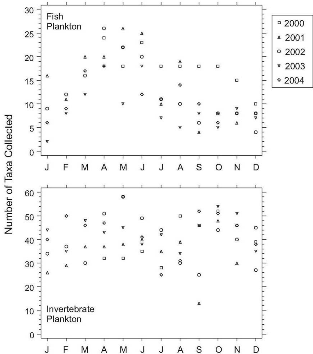
Figure 5-11 Number of taxa collected by month by plankton net (Figure from MacDonald et al. , 2005).
