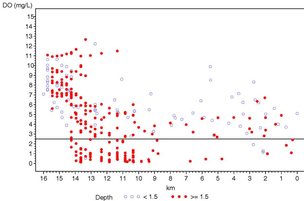
Figure 6-18 Bottom DO in the LHR as a function of river kilometer and depth for dam flows between 20 and 60 cfs.
