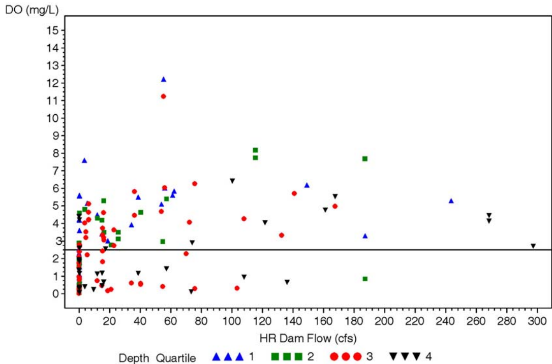
Figure 6-25c. Bottom DO for river km 12 as a function depth for dam flows between 0 and 300 cfs. Symbols are categorized by depth quartiles based on bottom area bathymetry for this region of the river.
