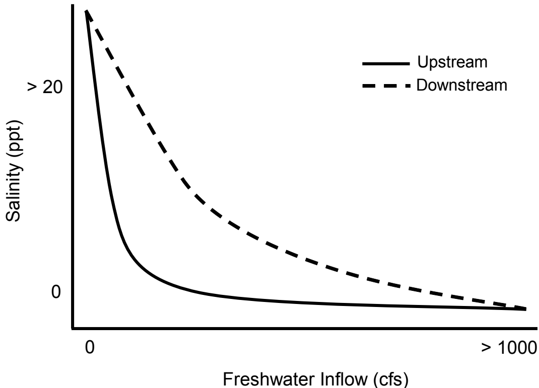
Figure 6-1 Conceptual expected response of salinity in the Lower Hillsborough River to freshwater inflow.
