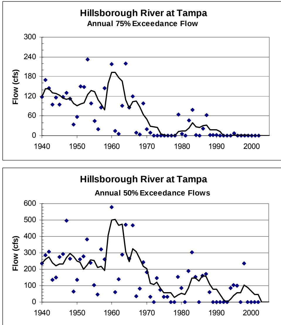
Figure 2-16 Annual 75% and 50% exceedance flows as measured on the Hillsborough River below the dam. The dark line is the 5-year moving average.
