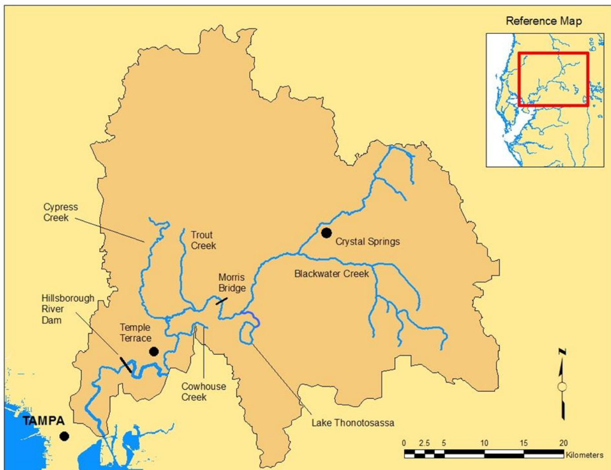
Figure 2-1 The Hillsborough River drainage basin and major tributaries.
