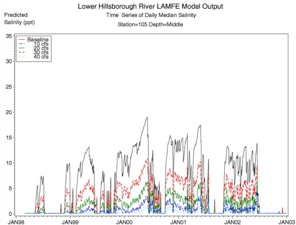
Figure 6-49 Predicted daily median salinity for the baseline and freshwater scenarios at EPCHC station 105, middle layer.
