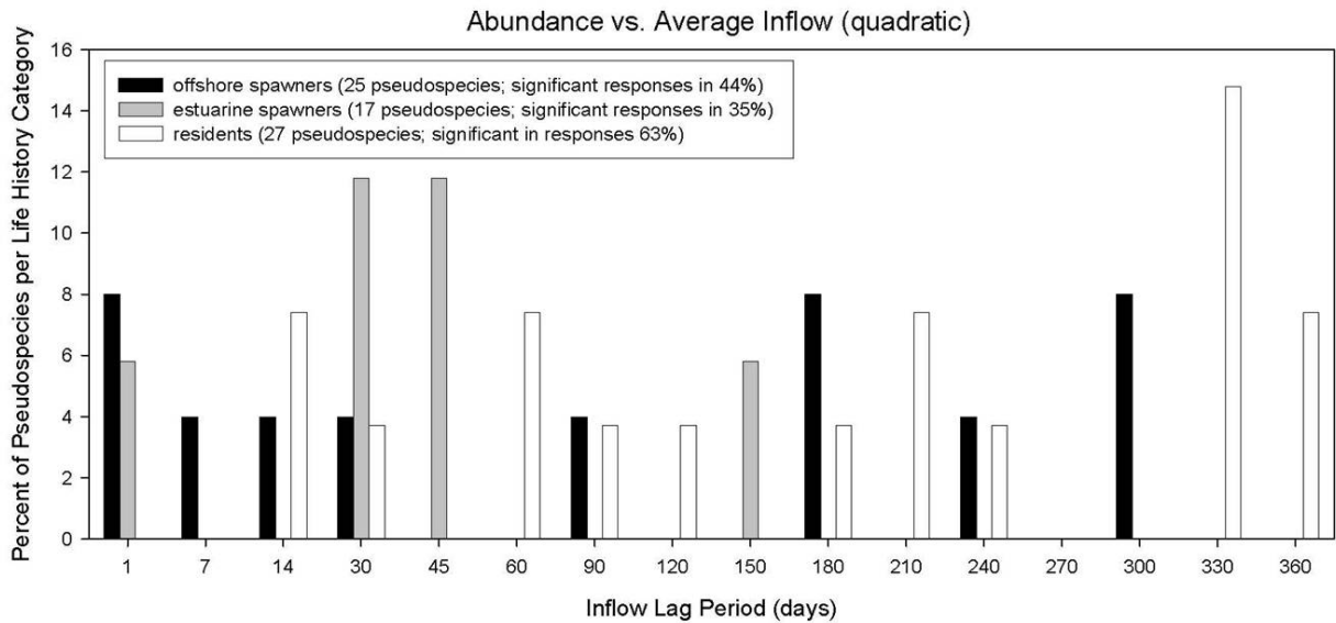
Figure 5-20 Summary of regression results assessing abundance in relation to inflow and lag period. (From MacDonald et al. , 2005).
