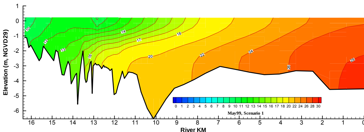
Figure 6-60 Predicted monthly median salinity for the Baseline Scenario, May 1999.
