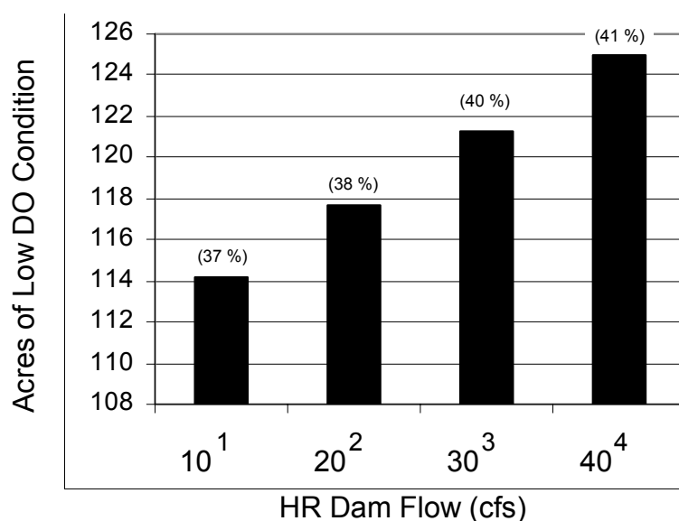
Figure 6-32 Acres of bottom DO<2.5 mg/L between Km 10 and Platt Street as a function of dam flow. Corresponding percent of bottom habitat in this region of the river indicated in parentheses.
