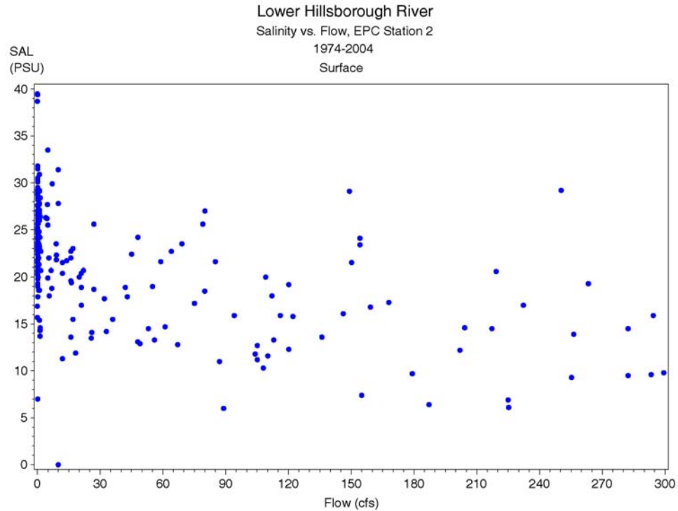
Figure 6-4 Long term EPCHC surface salinity observations at EPC Station 2 as a function of flow at the Hillsborough River Dam (Dam flow + Sulphur Springs diversions to the base of the dam). Data subset to flows less than 300 cfs for this figure.
