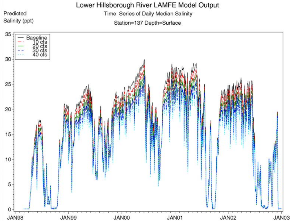
Figure 6-54 Predicted daily median salinity for the baseline and freshwater scenarios at EPCHC station 137, surface layer.
