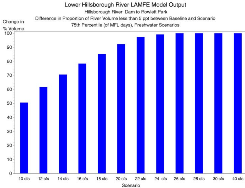
Figure 7-22 Difference in the proportion of volume less than 5 ppt between the baseline and freshwater Scenarios (Scenario - Baseline), 75 th percentile of MFL days, Dam to Rowlett Park.
