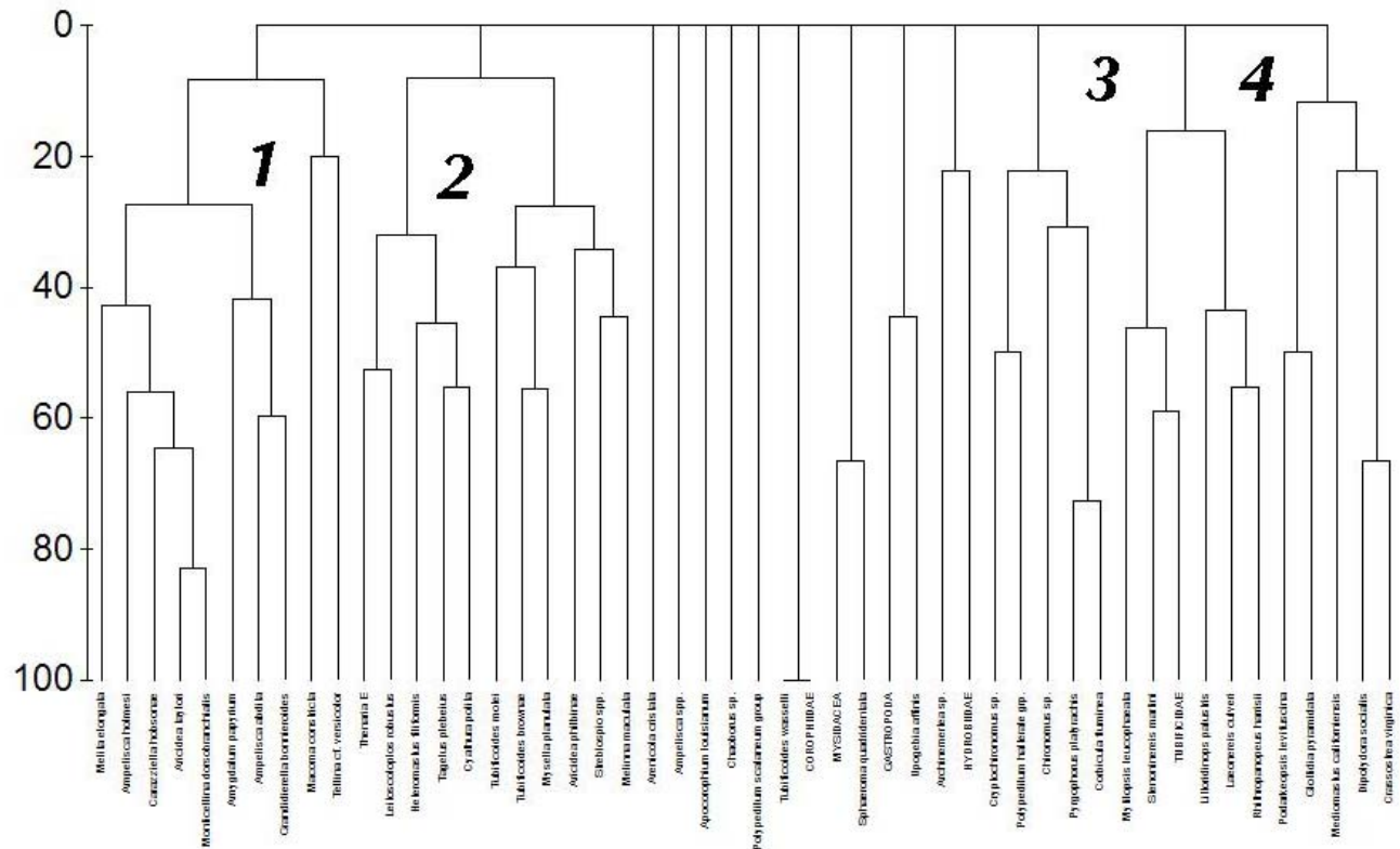
Figure 5-3. Dendrogram depicting the resemblance of taxonomic groups in the Lower Hillsborough River, 1995-2002: Presence-absence of 50 most frequently occurring taxa; complete linkage clustering. (From Grabe et al. 2004).
