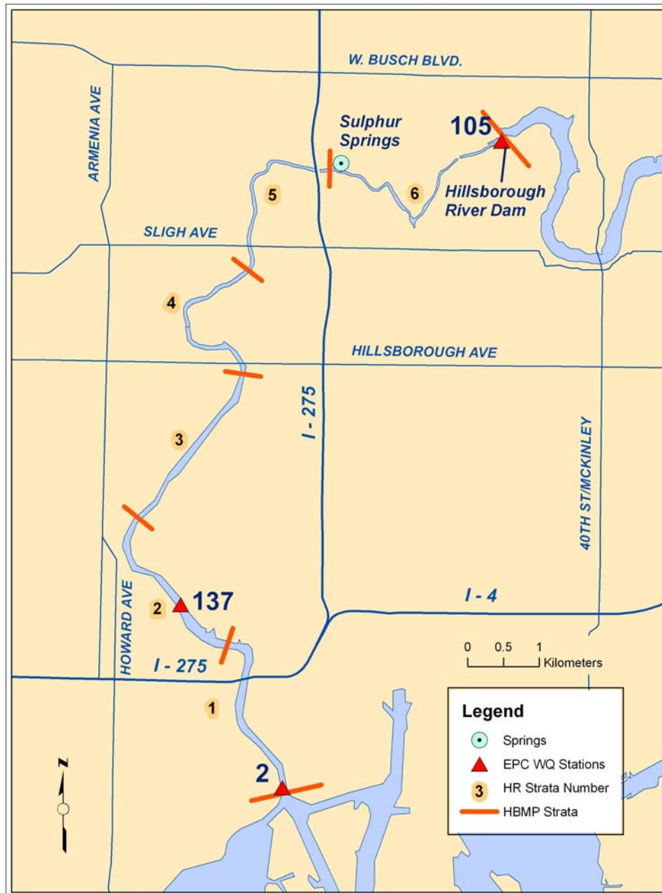
Figure 3-1 The LHR, including locations of EPCHC Ambient Water Quality sampling stations (2, 137, and 105) and HBMP sampling strata (1-6).
