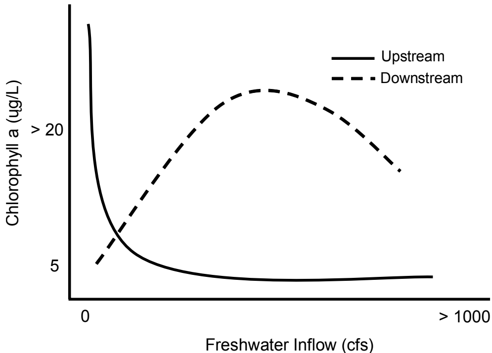
Figure 6-33 Conceptual expected response of chlorophyll a concentrations in the Lower Hillsborough River to freshwater inflow.
