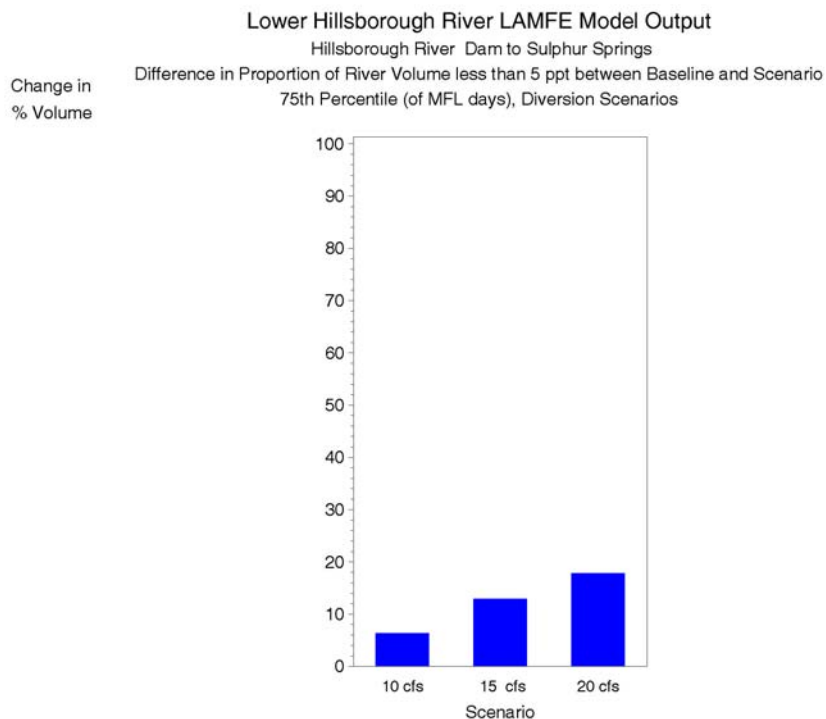
Figure 7-31 Difference in the proportion of volume less than 5 ppt between the baseline and Sulphur Springs diversion scenarios (scenario - baseline), 75 th percentile of MFL days.
