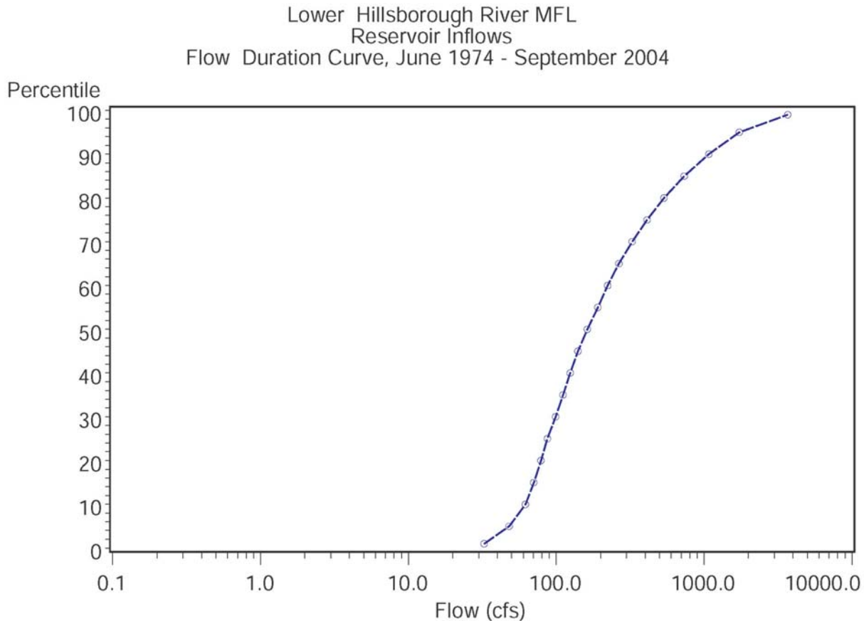
Figure 2-6 Flow duration curve of estimated inflows to the Hillsborough River Reservoir, 1974-2004.
