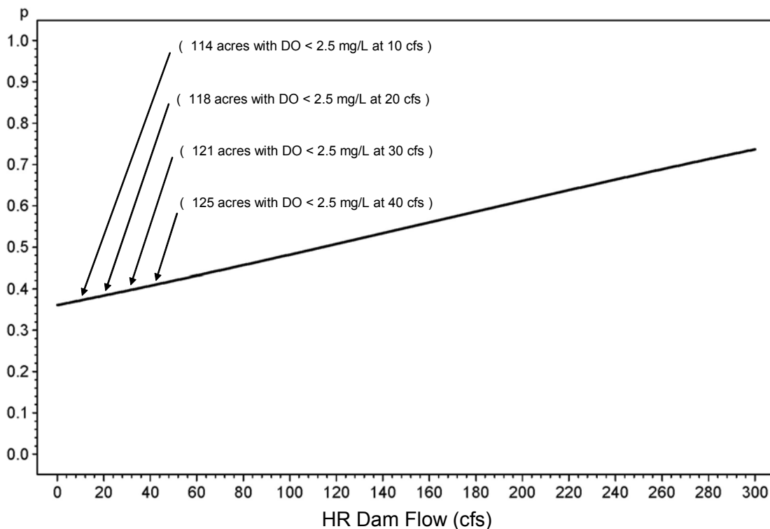
Figure 6-31 Probability of bottom DO<2.5 mg/L between Km 10 and Platt Street as a function of dam flow (calculated as the mean of estimates by 0 th , 25 th , 50 th , 75 th , and 100 th depth percentile). For reference, the probabilities are expressed as acres of river bottom for several example flow values (more precisely, the probabilities represent joint probabilities over time and space).
