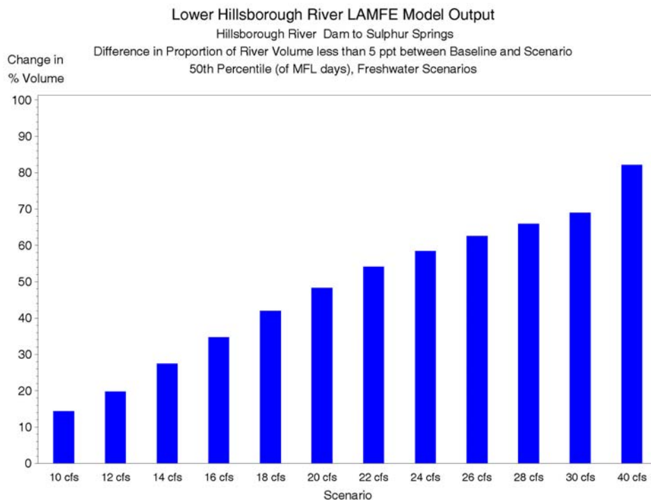
Figure 7-15 Difference in the proportion of volume less than 5 ppt between the baseline and freshwater Scenarios (Scenario - Baseline), 50 th percentile of MFL days, Dam to Sulphur Springs.
