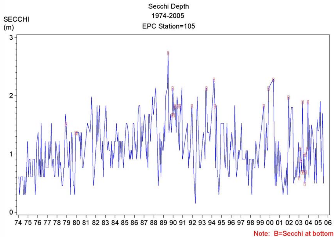
Figure 4-8 Monthly time series of Secchi disk depth at EPCHC Station 105 (near Rowlett Park).
