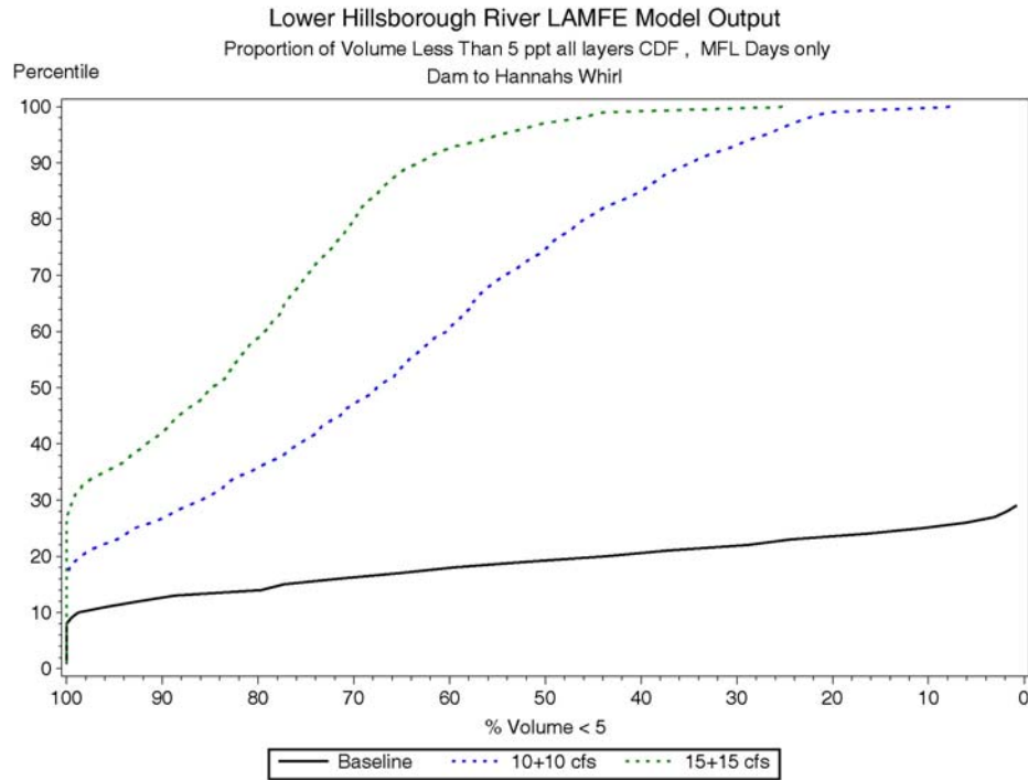
Figure 7-51 CDF plot of percent volume less than 5 ppt from the dam to Hannah’s Whirl versus percentile of MFL days for combination scenarios as well baseline.
