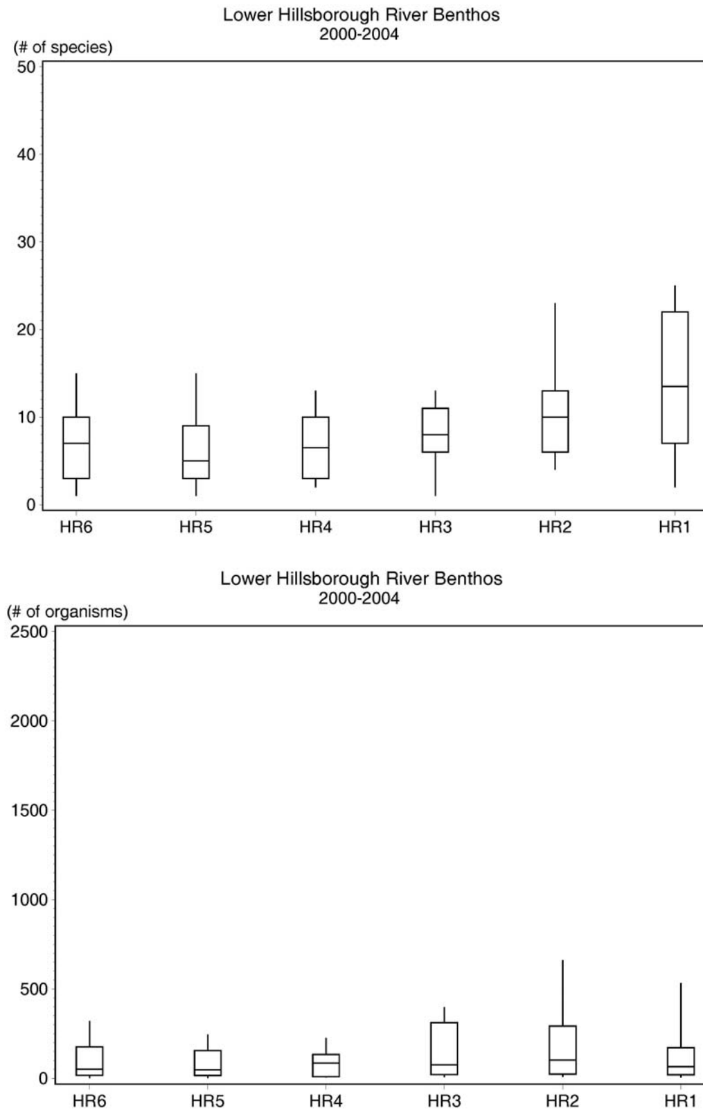
Figure 5-5. Lower Hillsborough River benthos species richness and total abundance by stratum, Tampa Bay Water HBMP data 2000-2004.
