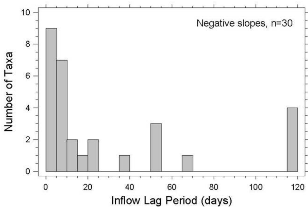
Figure 5-17 Distribution of the abundance response lags for fish taxa exhibiting positive and negative response slopes (Figure from MacDonald et al. , 2005).
