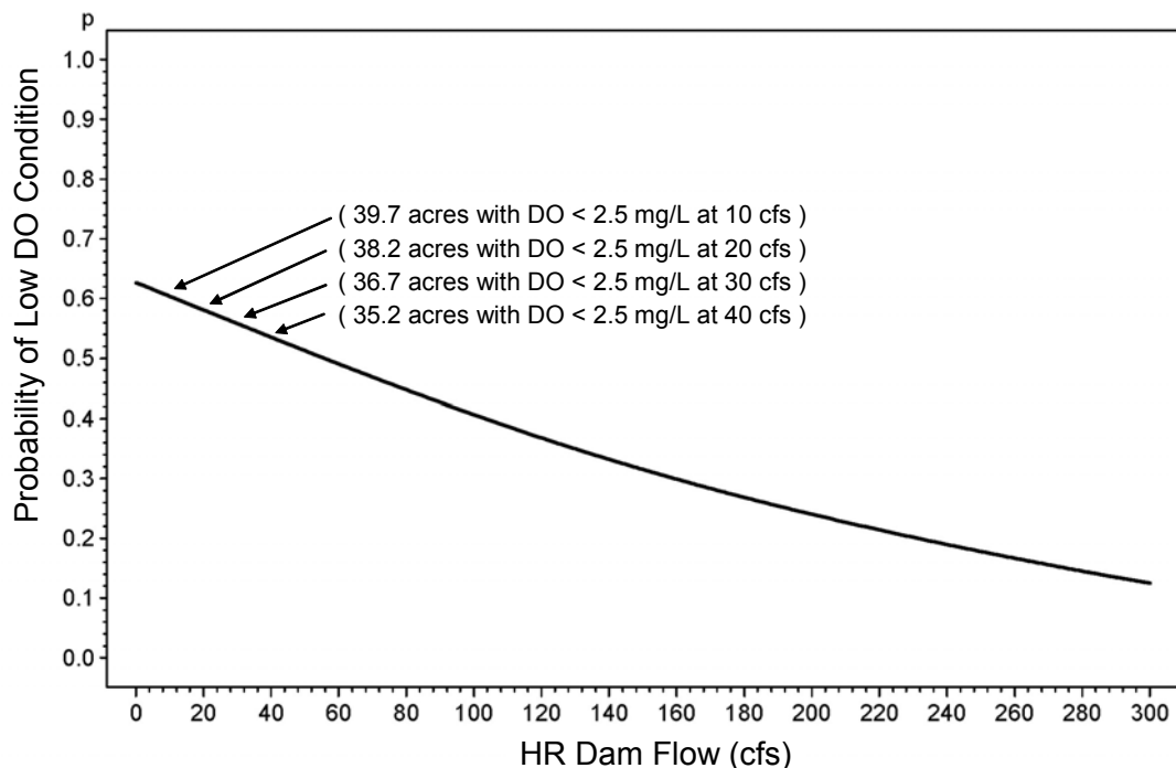
Figure 6-27 Probability of bottom DO<2.5 mg/L between Km 10 and 14 as a function of dam flow (calculated as the mean of estimates by 0 th , 25 th , 50 th , 75 th , and 100 th depth percentile). For reference, the probabilities are expressed as acres of river bottom for several example flow values (more precisely, the probabilities represent joint probabilities over time and space).
