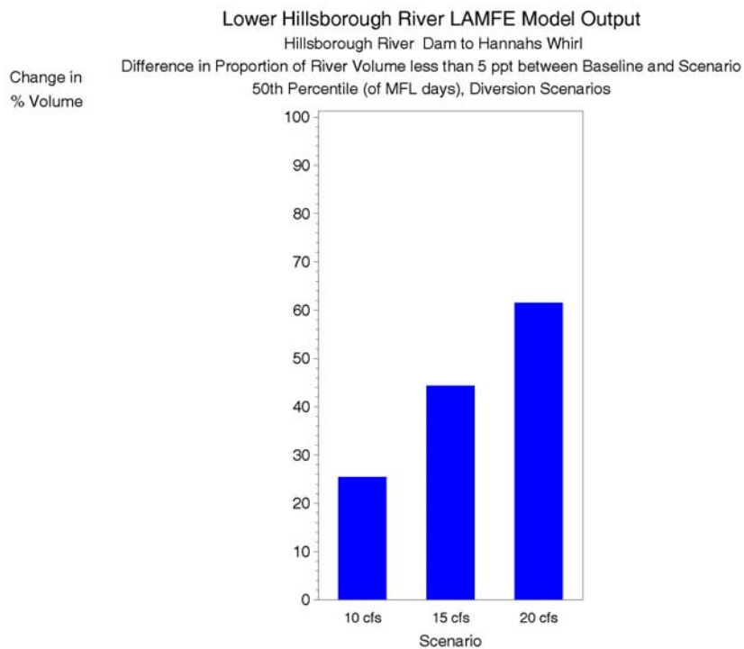
Figure 7-33 Difference in the proportion of volume less than 5 ppt between the baseline and Hannah's Whirl diversion scenarios (scenario - baseline), 50 th percentile of MFL days.
