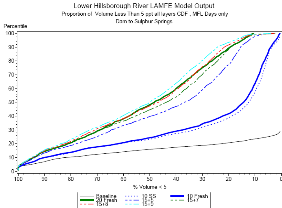
Figure 8.2. Comparison of the effect of 20 cfs freshwater against various blends of Sulphur Springs and freshwater.
