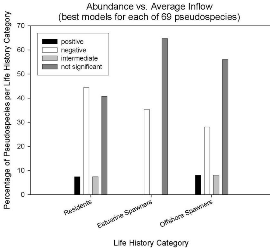
Figure 5-19 Summary of regression results assessing fish abundance in relation to inflow. Positive and negative indicate increases and decreases in abundance with increasing flow, while intermediate indicates maximum or minimum abundances at intermediate flows. (Figure from MacDonald et al. , 2005).
