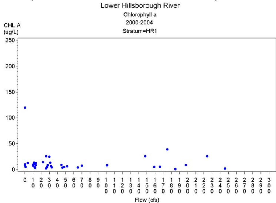
Figure 6-36. Observed response of chlorophyll a at EPC Station 2 as a function of flow at the Hillsborough River Dam (Dam flow + Sulphur Springs diversions to the base of the dam). Data subset to flows less than 300 cfs for this figure.
