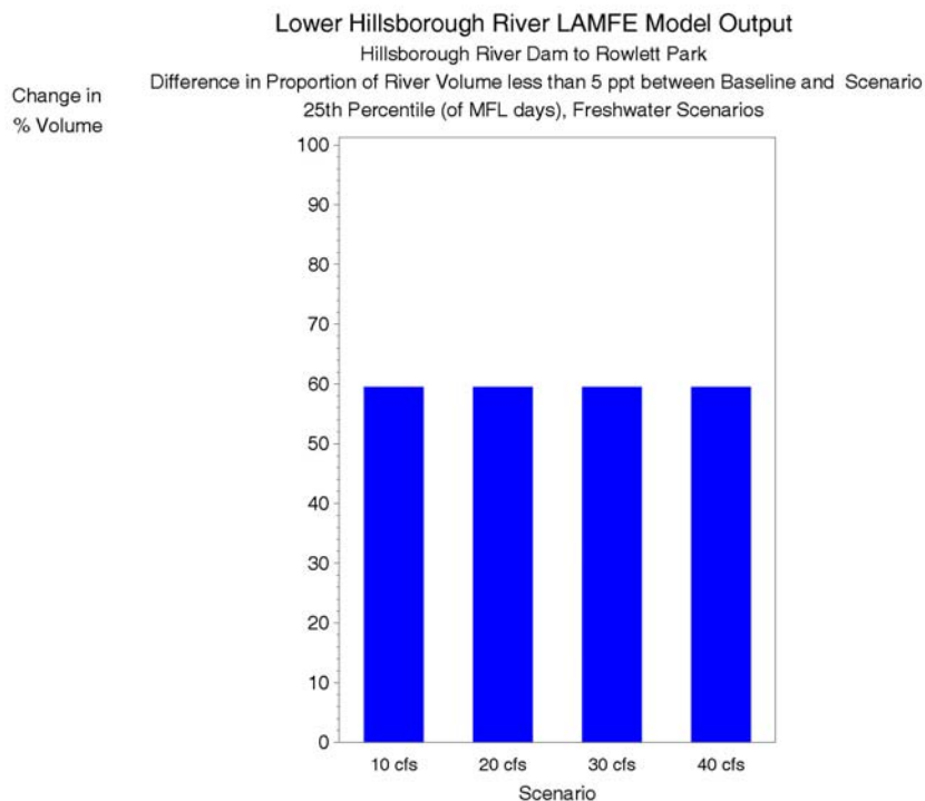
Figure 7-8 Difference in the proportion of volume less than 5 ppt between the baseline and freshwater Scenarios (Scenario - Baseline), 25 th percentile of MFL days, Dam to Rowlett Park.
