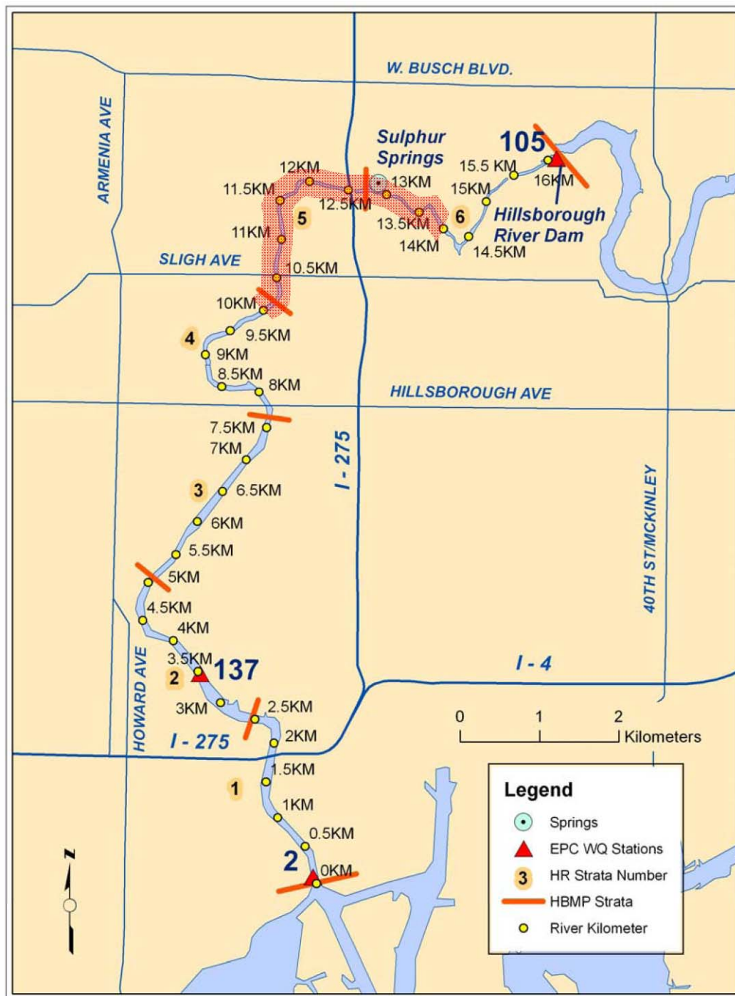
Figure 6-19 The most prevalent region (River Kilometer 10 to 14) of low bottom DO conditions in the LHR for flow conditions between 20 and 60 cfs.
