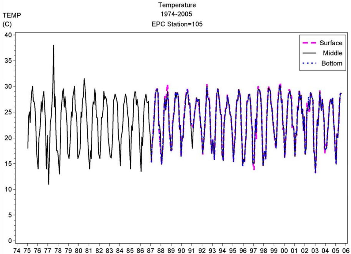
Figure 4-3 Monthly time series of surface and bottom temperature at EPCHC Station 105 (near Rowlett Park).
