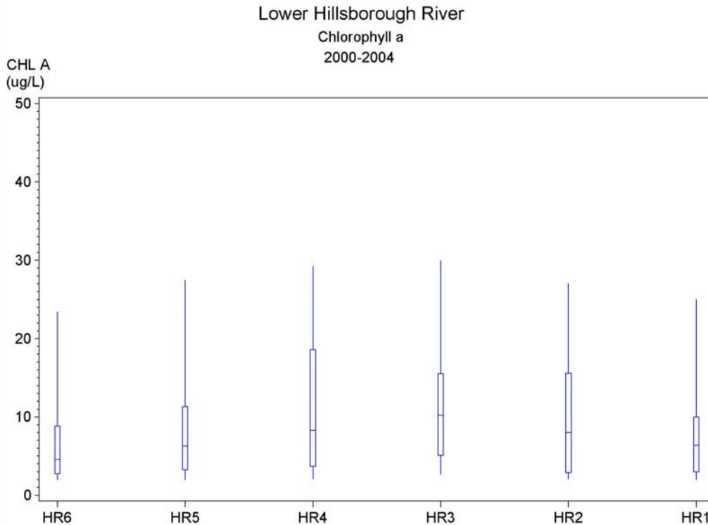
Figure 4-22 Observed longitudinal distributions of chlorophyll a for the Tampa Bay Water HBMP program period of record.
