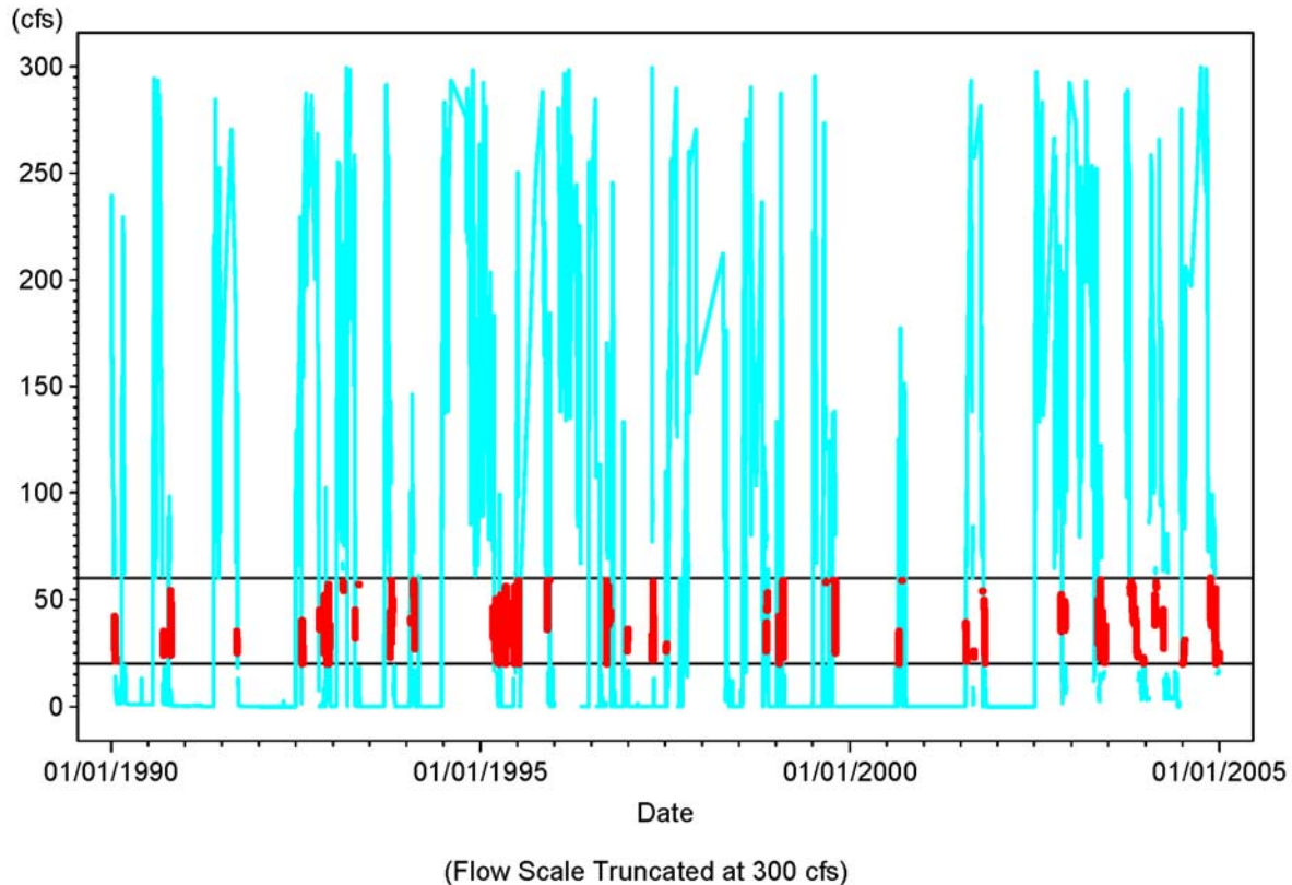
Figure 6-20 Daily flow values for the Hillsborough River Dam with flows between 20 and 60 cfs highlighted in red. High flow values truncated at 300 cfs for graphical purposes.
