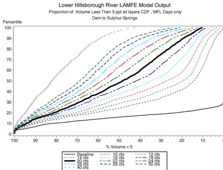
Figure 7-23 CDF plot of percent volume less than 5 ppt from the dam to Sulphur Springs versus percentile of MFL days for the additional freshwater Scenarios.
