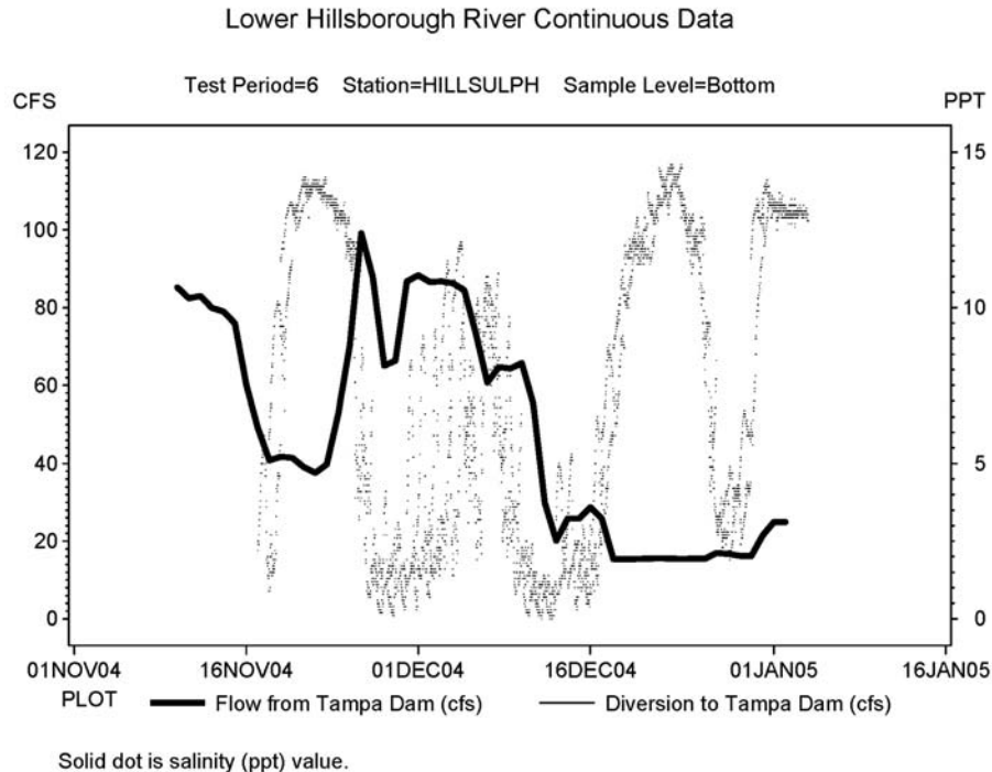
Figure 6-14 Dam flow and spring diversion flow during Test Period 6 (left axis), and observed Hillsborough River at Sulphur Springs continuous recorder bottom salinity (right axis – solid circles). There were no spring diversions during this test period.
