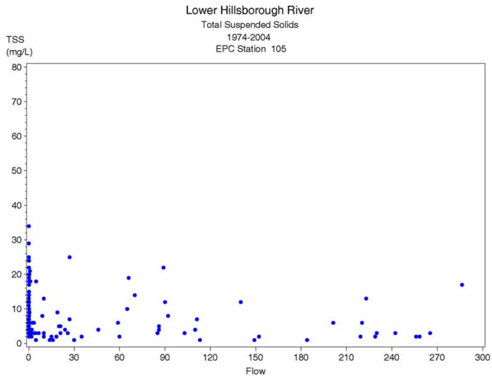
Figure 6-45 Observed response of total suspended solids concentration at EPC Station 105 as a function of flow at the Hillsborough River Dam (Dam flow + Sulphur Springs diversions to the base of the dam). Data were subset to flows less than 300 cfs.
