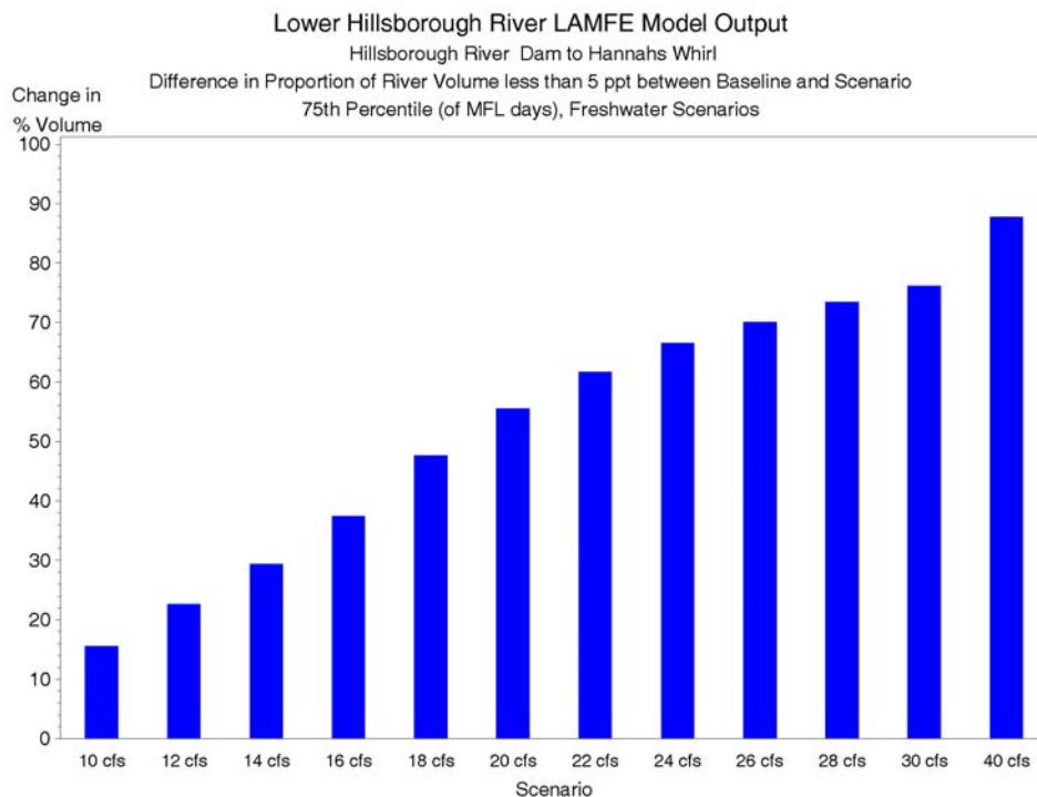
Figure 7-19 Difference in the proportion of volume less than 5 ppt between the baseline and freshwater Scenarios (Scenario - Baseline), 75 th percentile of MFL days, Dam to Hannah's Whirl.
