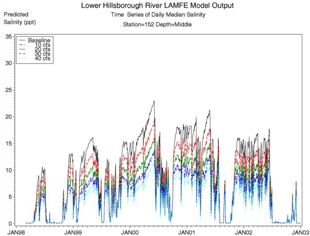
Figure 6-52 Predicted daily median salinity for the baseline and freshwater scenarios at EPCHC station 152, middle layer.
