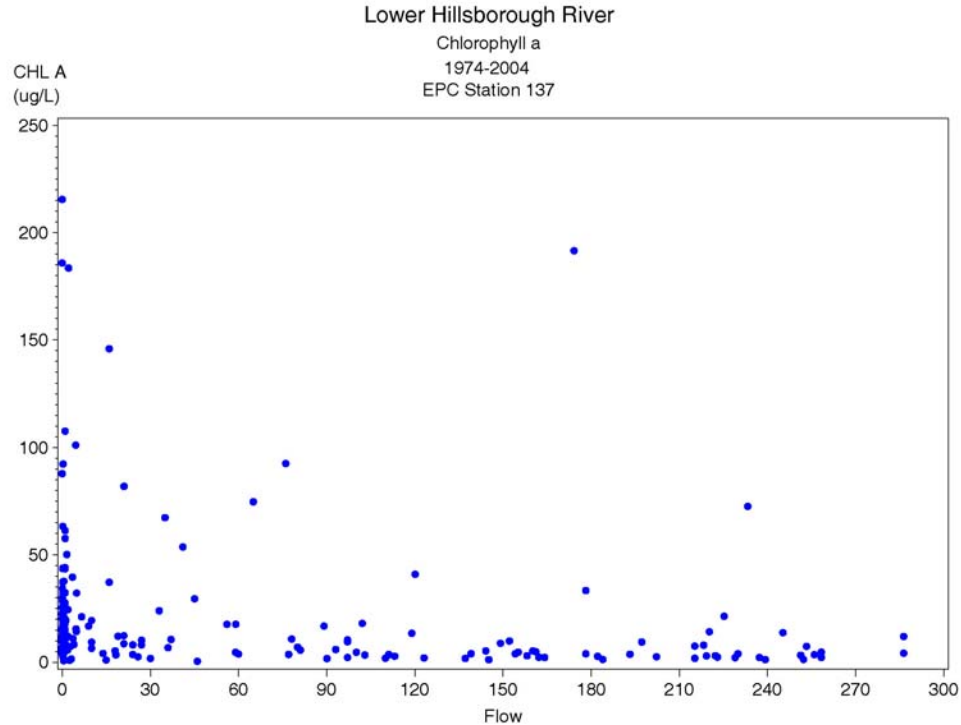
Figure 6-35. Observed response of chlorophyll a at EPC Station 137 as a function of flow at the Hillsborough River Dam (Dam flow + Sulphur Springs diversions to the base of the dam). Data subset to flows less than 300 cfs for this figure.
