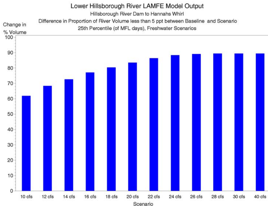
Figure 7-17 Difference in the proportion of volume less than 5 ppt between the baseline and freshwater Scenarios (Scenario - Baseline), 25 th percentile of MFL days, Dam to Hannah's Whirl.
