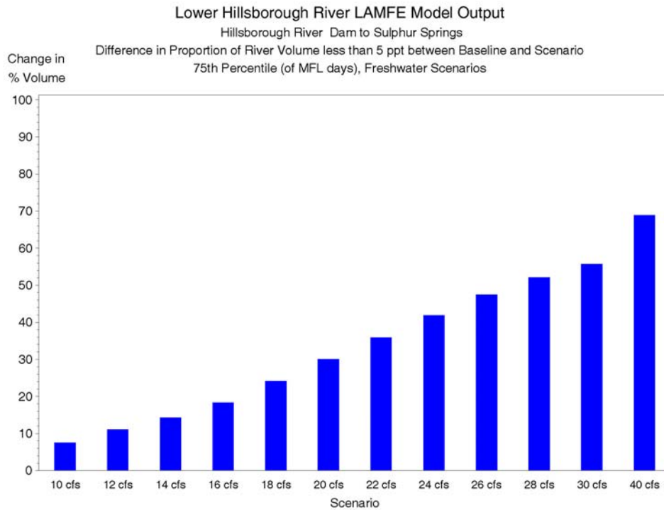
Figure 7-16 Difference in the proportion of volume less than 5 ppt between the baseline and freshwater Scenarios (Scenario - Baseline), 75 th percentile of MFL days, Dam to Sulphur Springs.
