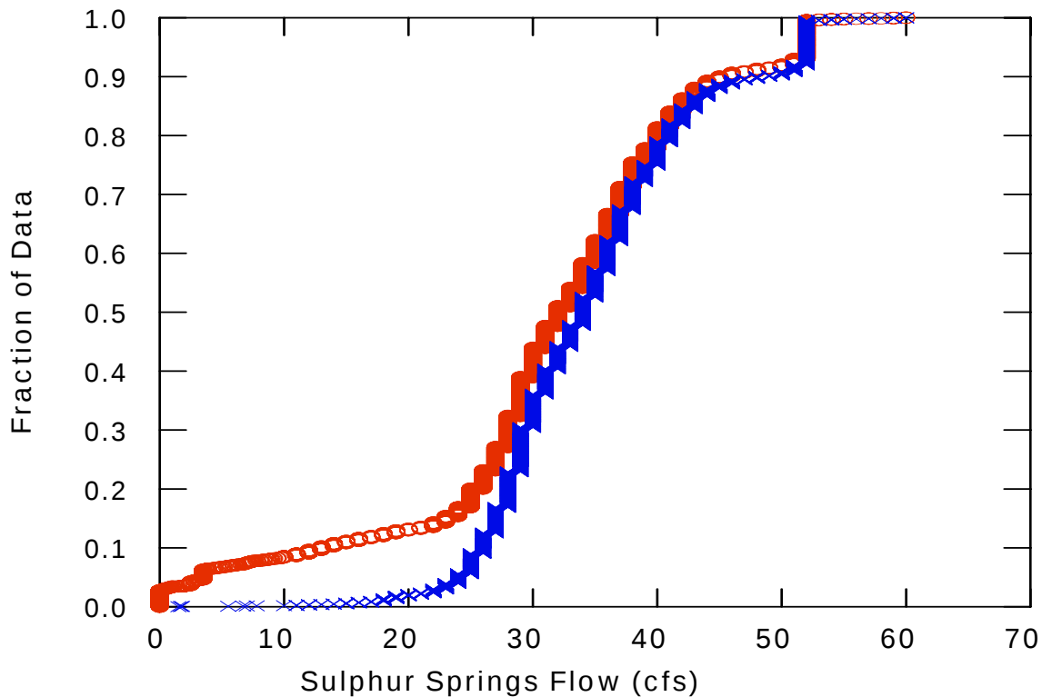
Figure 2-13 Flow duration curves for daily flows from Sulphur Springs, 1991–2002. Blue represents days with no withdrawals, red includes all daily records. (From: SWFWMD, 2004b)
