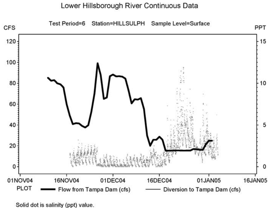
Figure 6-13 Dam flow and spring diversion flow during Test Period 6 (left axis), and observed Hillsborough River at Sulphur Springs continuous recorder surface salinity (right axis – solid circles). There were no spring diversions during this test period.
