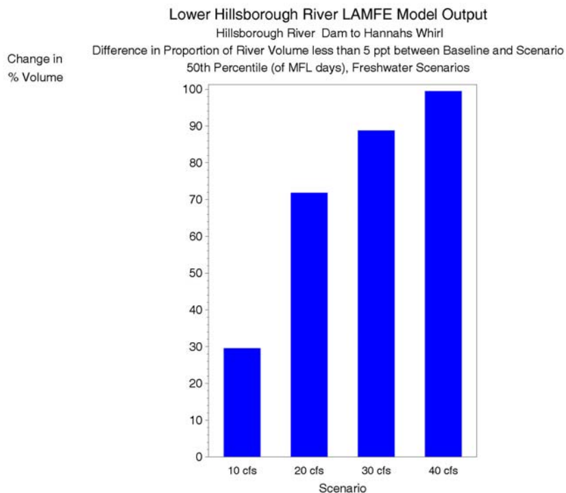
Figure 7-6 Difference in the proportion of volume less than 5 ppt between the baseline and freshwater Scenarios (Scenario - Baseline), 50 th percentile of MFL days, Dam to Hannah's Whirl.
