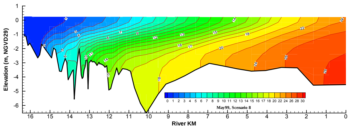
Figure 6-64 Predicted monthly median salinity for the 40 cfs freshwater Scenario, May 1999.
