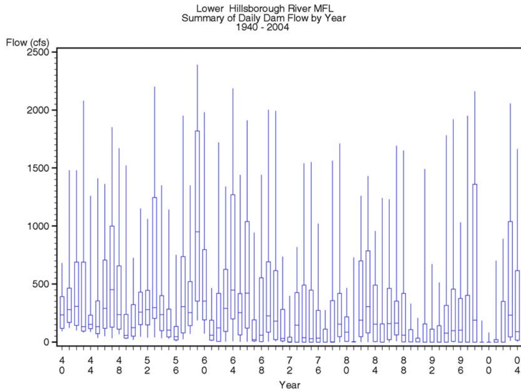
Figure 2-7 Box and whisker plot of daily Hillsborough River Dam flows by year, 1940-2004. Whiskers represent the 5 th and 95 th percentiles.
