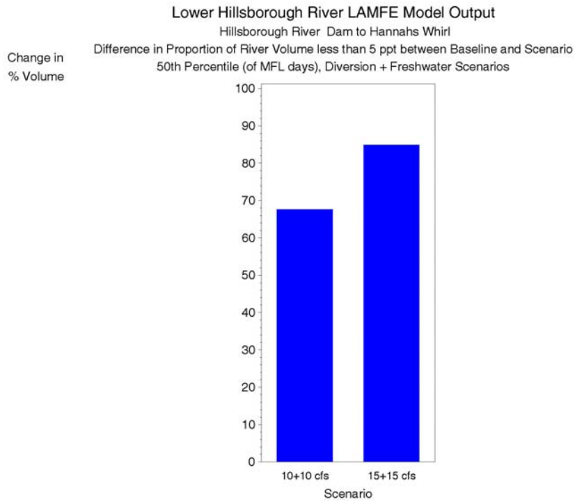
Figure 7-45 Difference in the proportion of volume less than 5 ppt between the baseline and Hannah's Whirl for the diversion scenarios (scenario - baseline), 50 th percentile of MFL days.
