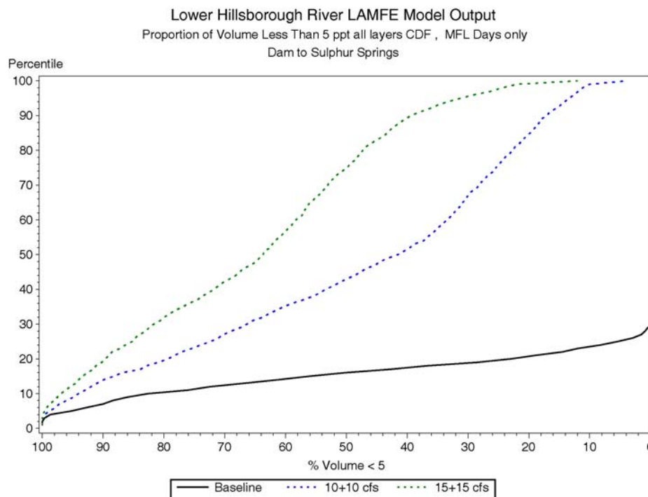
Figure 7-50 CDF plot of percent volume less than 5 ppt from the dam to Sulphur Springs versus percentile of MFL days for combination scenarios as well baseline.
