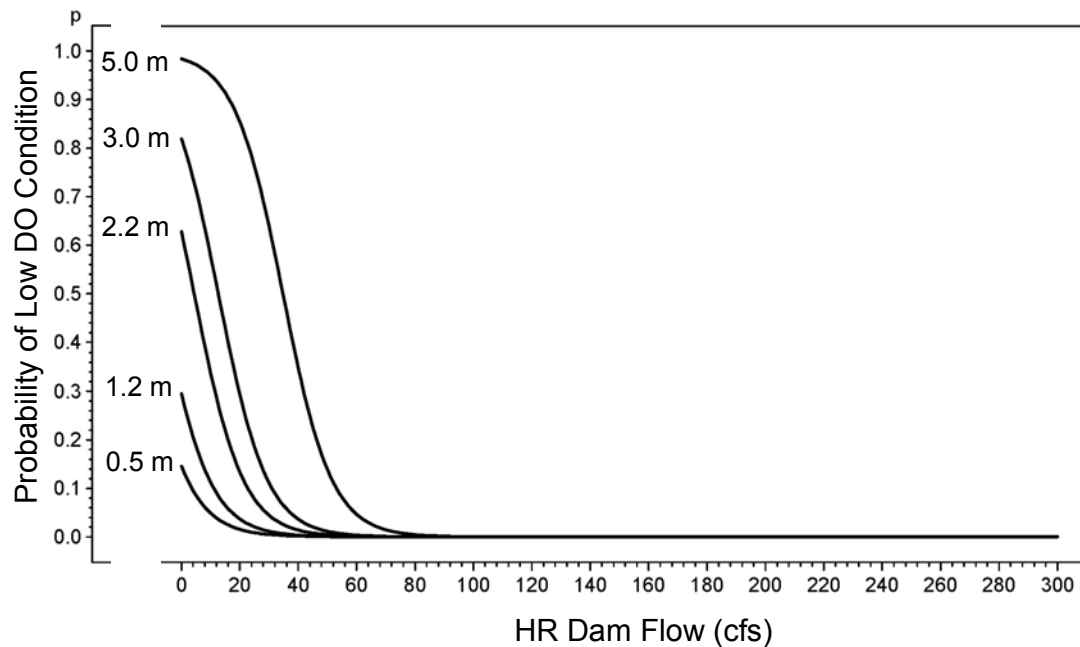
Figure 6-22 Probability of bottom DO < 2.5 mg/L between Km 14 and the dam as a function of dam flow and depth for dam flows between 0 and 300 cfs. Estimates are shown for depth percentiles (0 th , 25 th , 50 th , 75 th ) and the deepest depth (5.0 m) for which DO data were reported based on bottom area.
