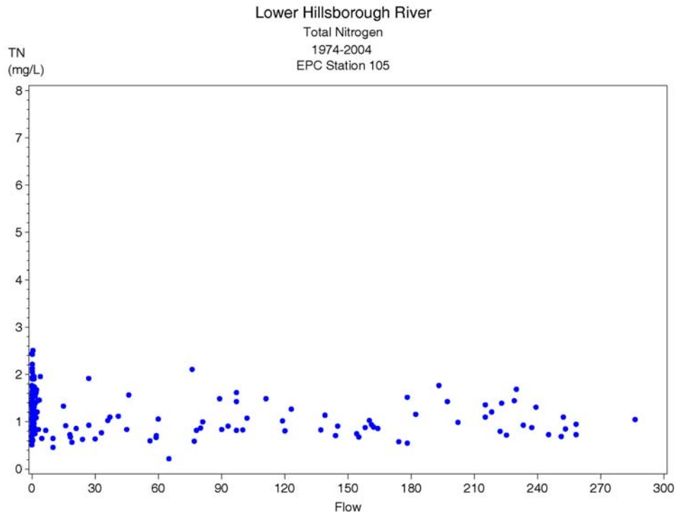
Figure 6-39 Observed response of total nitrogen concentration at EPC 105 as a function of flow at the Hillsborough River Dam (Dam flow + Sulphur Springs diversions to the base of the dam). Data were subset to flows less than 300 cfs for this figure.
