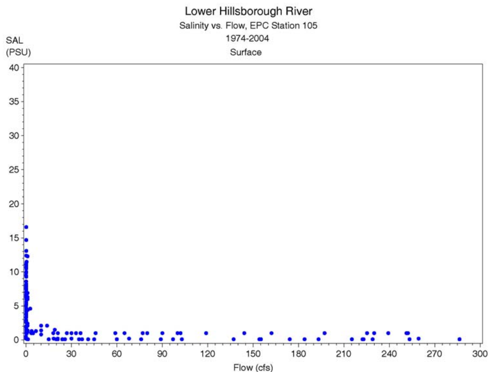
Figure 6-2 Long term EPCHC surface salinity observations at EPC Station 105 as a function of flow at the Hillsborough River Dam (Dam flow + Sulphur Springs diversions to the base of the dam). Data subset to flows less than 300 cfs for this figure.
