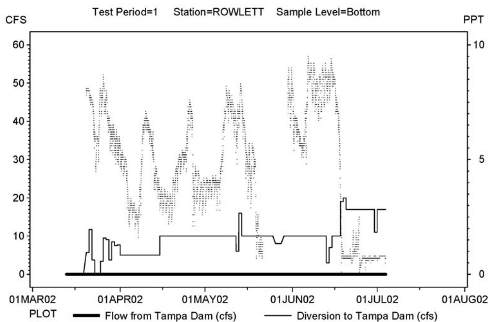
Figure 6-8 Dam flow and spring diversion flow during Test Period 1 (left axis), and observed Rowlett Park continuous recorder bottom salinity (right axis- solid circles).
