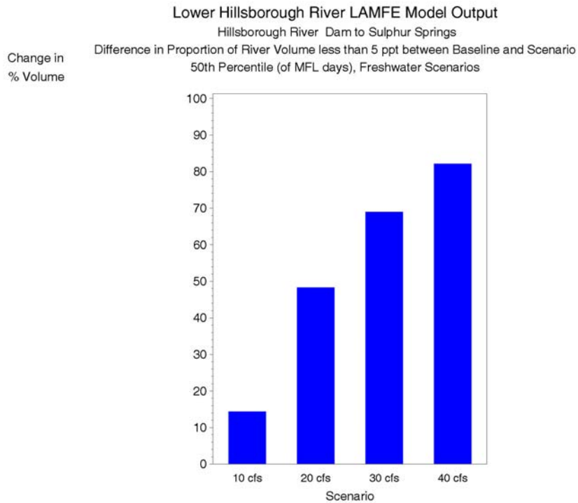
Figure 7-3 Difference in the proportion of volume less than 5 ppt between the baseline and freshwater Scenarios (Scenario - Baseline), 50 th percentile of MFL days, Dam to Sulphur Springs.
