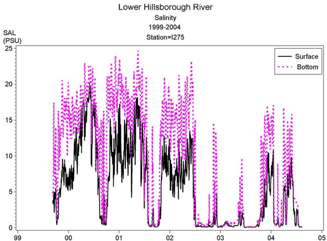
Figure 4-15 Observed USGS/District continuous recorder time series of mean daily surface and bottom salinity near I-275.
