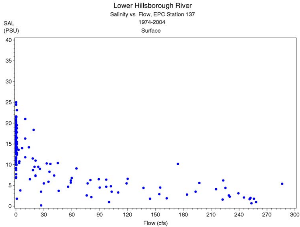
Figure 6-3 Long term EPCHC surface salinity observations at EPC Station 137 as a function of flow at the Hillsborough River Dam (Dam flow + Sulphur Springs diversions to the base of the dam). Data subset to flows less than 300 cfs for this figure.
