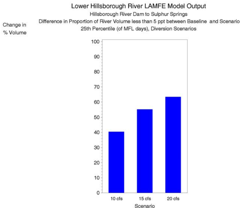
Figure 7-29 Difference in the proportion of volume less than 5 ppt between the baseline and Sulphur Springs diversion scenarios (scenario - baseline), 25 th percentile of MFL days.
