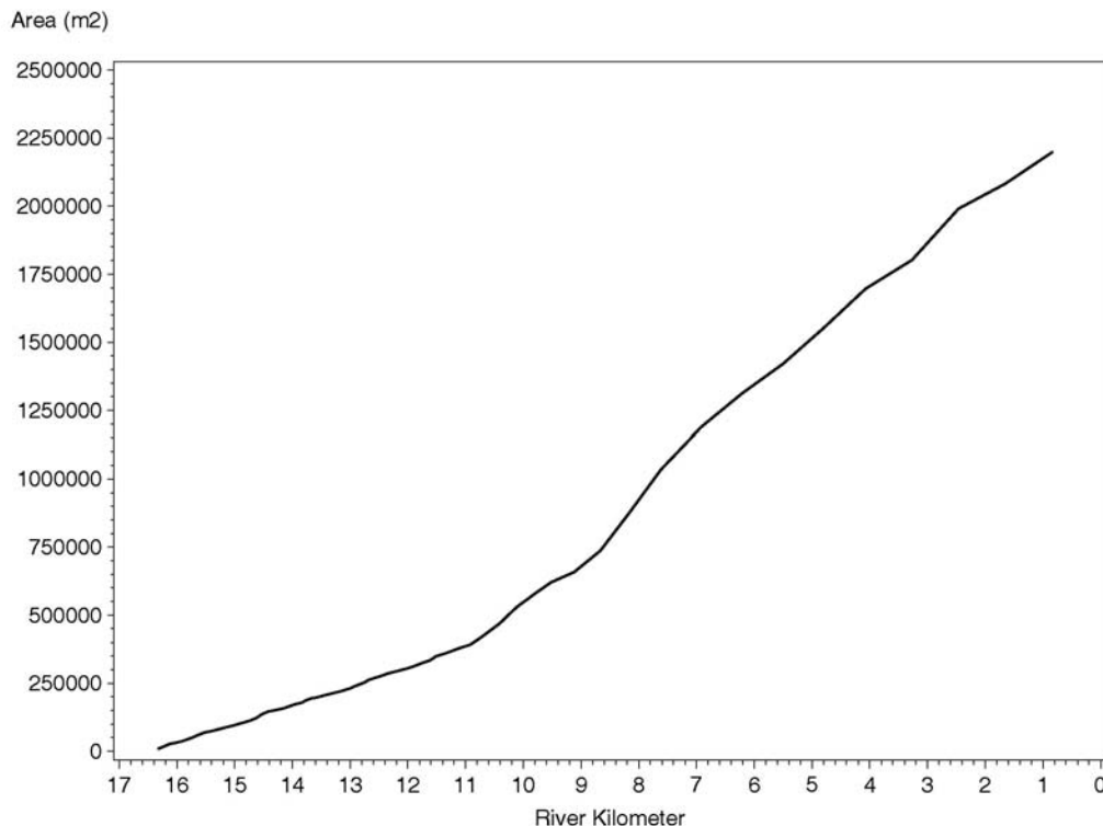
Figure 3-3 Cumulative surface area by river kilometer in the LHR.
