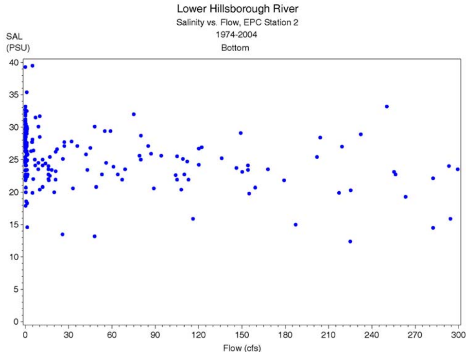
Figure 6-7 Long term EPCHC bottom salinity observations at EPC Station 2 as a function of flow at the Hillsborough River Dam (Dam flow + Sulphur Springs diversions to the base of the dam). Data subset to flows less than 300 cfs for this figure.
