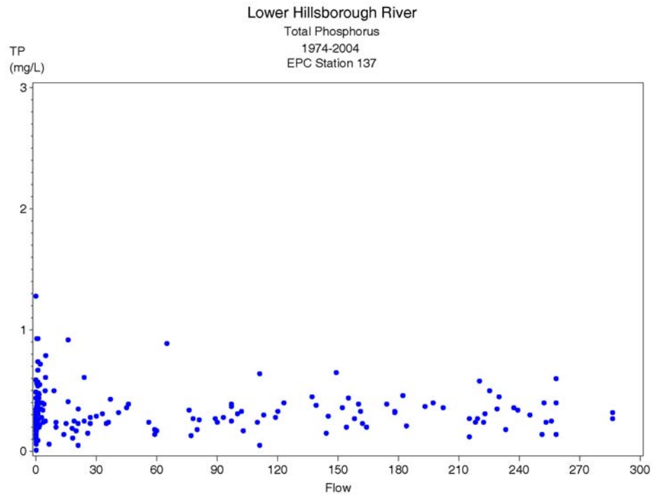
Figure 6-43. Observed response of total phosphorous concentration at EPC Station 137 as a function of flow at the Hillsborough River Dam (Dam flow + Sulphur Springs diversions to the base of the dam). Data were subset to flows less than 300 cfs and TP values less than 4 for this figure.
