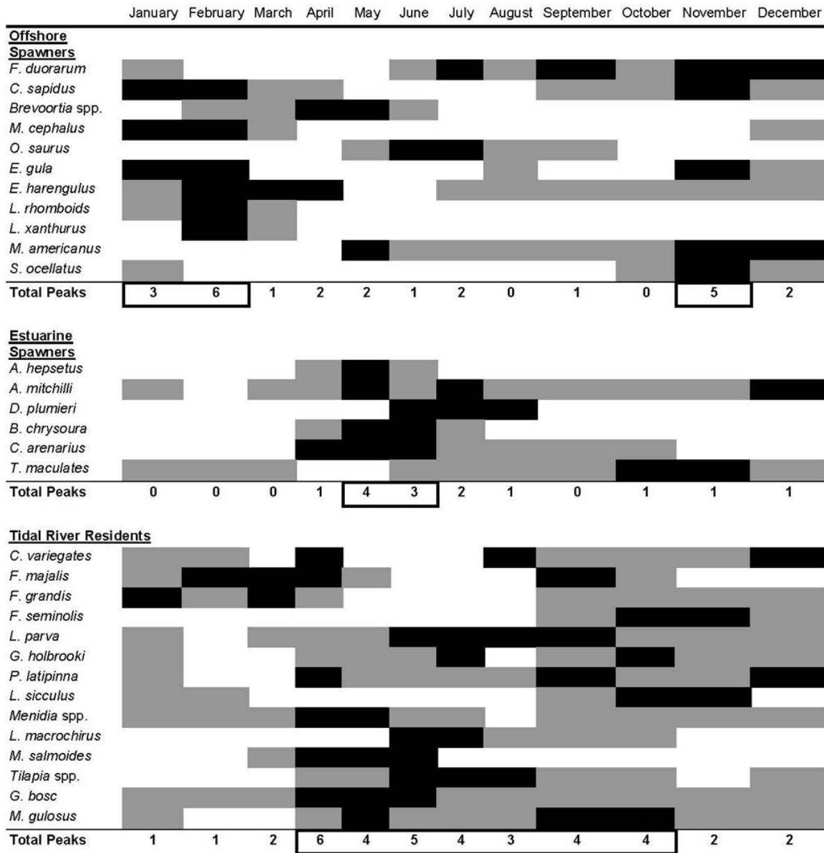
Figure 5-14 Months of occurrence (gray) and peak abundance (black) for new recruits collected by seine and trawl nets (Figure from MacDonald et al. , 2005).
