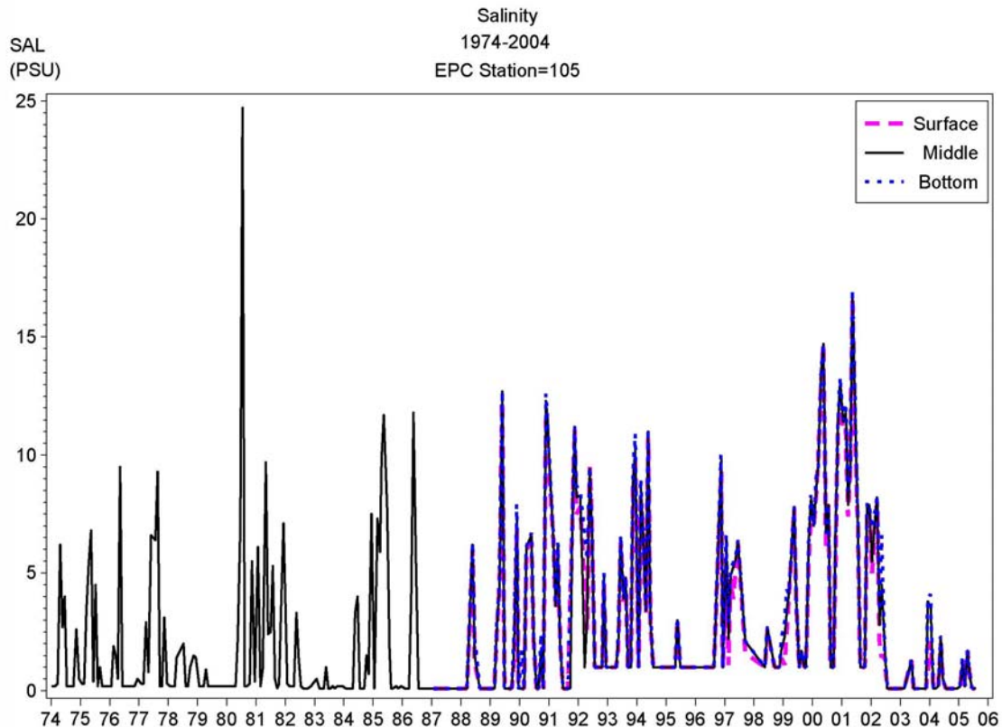
Figure 4-2 Monthly time series of surface, middle, and bottom salinity at EPCHC Station 105 (near Rowlett Park).
