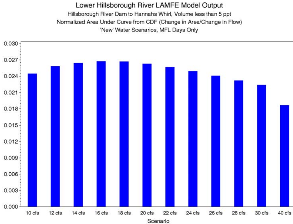
Figure 7-27 Normalized area under the curve based on CDF plot of percent volume less than 5 ppt from the dam to Hannah's Whirl versus percentile of MFL days for the additional freshwater Scenarios.
