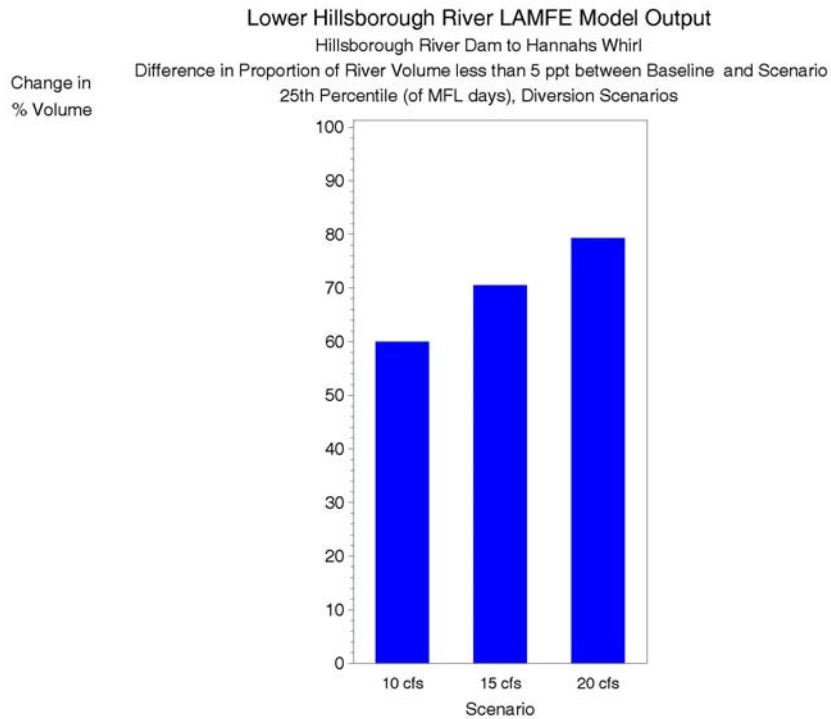
Figure 7-32 Difference in the proportion of volume less than 5 ppt between the baseline and Hannah's Whirl diversion scenarios (scenario - baseline), 25 th percentile of MFL days.
