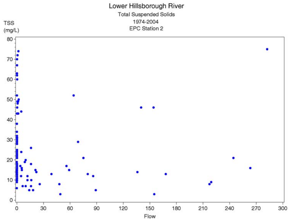
Figure 6-47. Observed response of total suspended solids concentration at EPC Station 2 as a function of flow at the Hillsborough River Dam (Dam flow + Sulphur Springs diversions to the base of the dam). Data were subset to flows less than 300 cfs.
