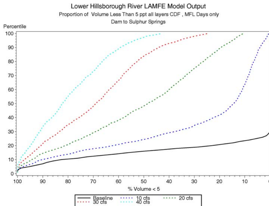
Figure 7-11 CDF plot of percent volume from the dam to Sulphur Springs less than 5 ppt for MFL days for freshwater scenarios.
