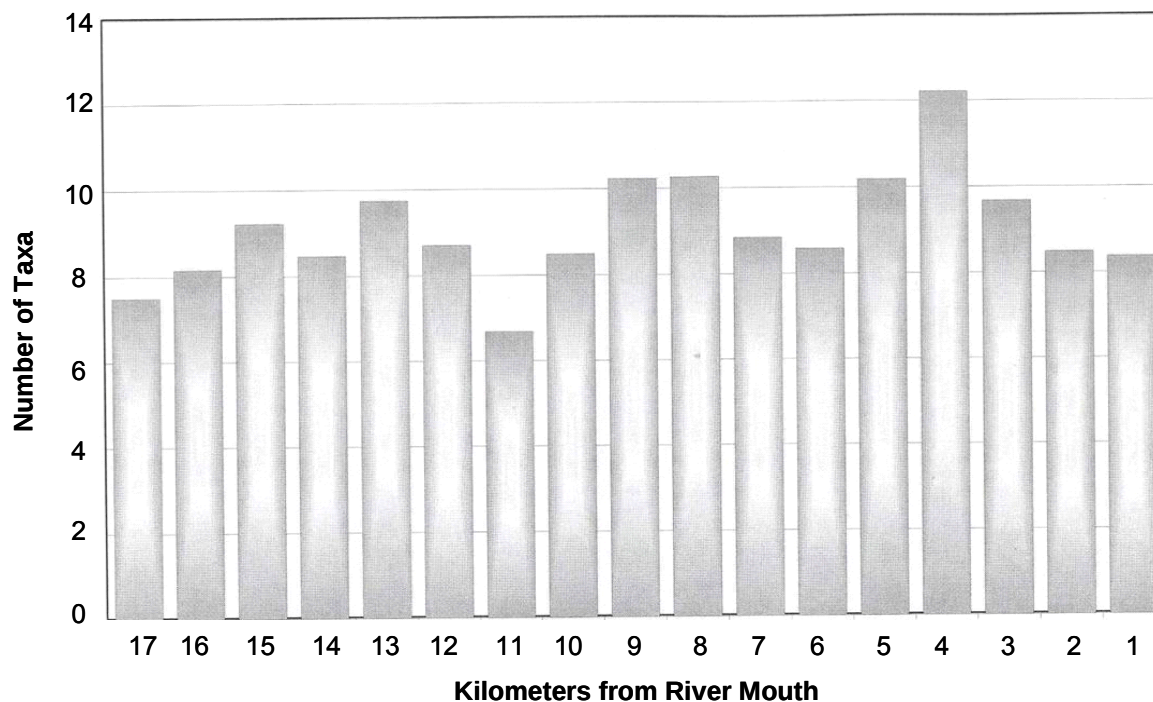
Figure 5-10 Average number of fish taxa per sample in the HR by river kilometer, May 2000 through December 2002 (From: PBS&J, 2003).
