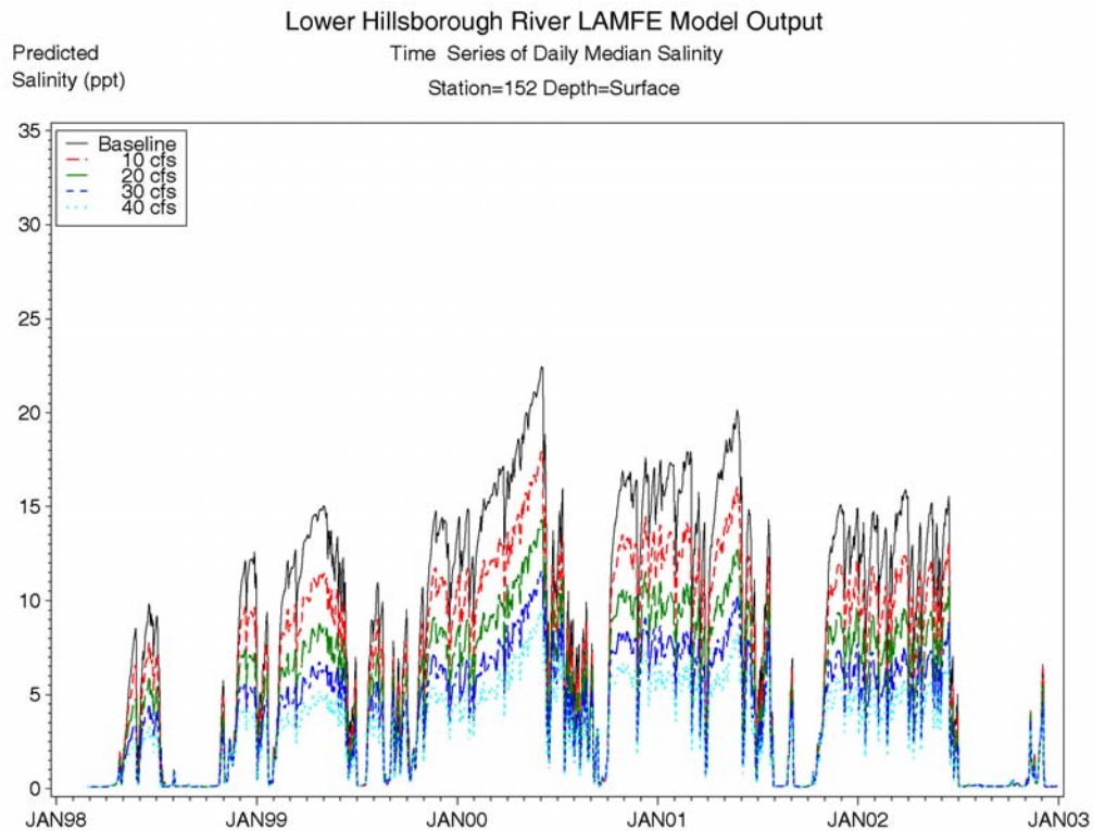
Figure 6-51 Predicted daily median salinity for the baseline and freshwater scenarios at EPCHC station 152, surface layer.
