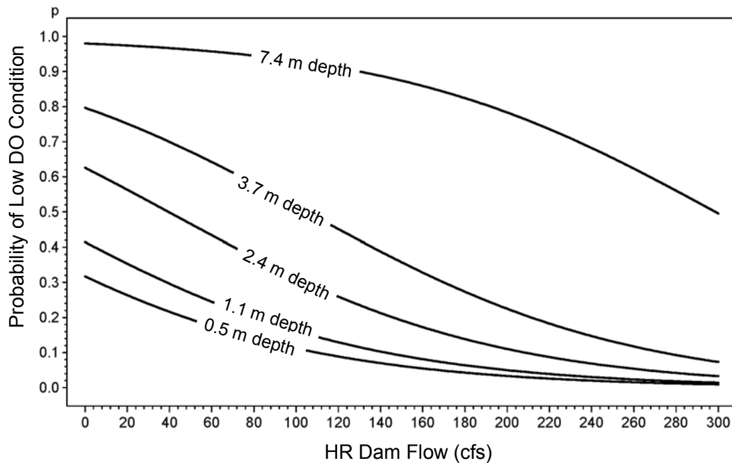
Figure 6-26. Probability of bottom DO<2.5 mg/L between Km 10 and 14 as a function of river kilometer and depth for dam flows between 0 and 300 cfs. Estimates are shown for depth percentiles (0 th , 25 th , 50 th , 75 th ) and the deepest depth (7.4 m) for which DO data were reported based on bottom area.
