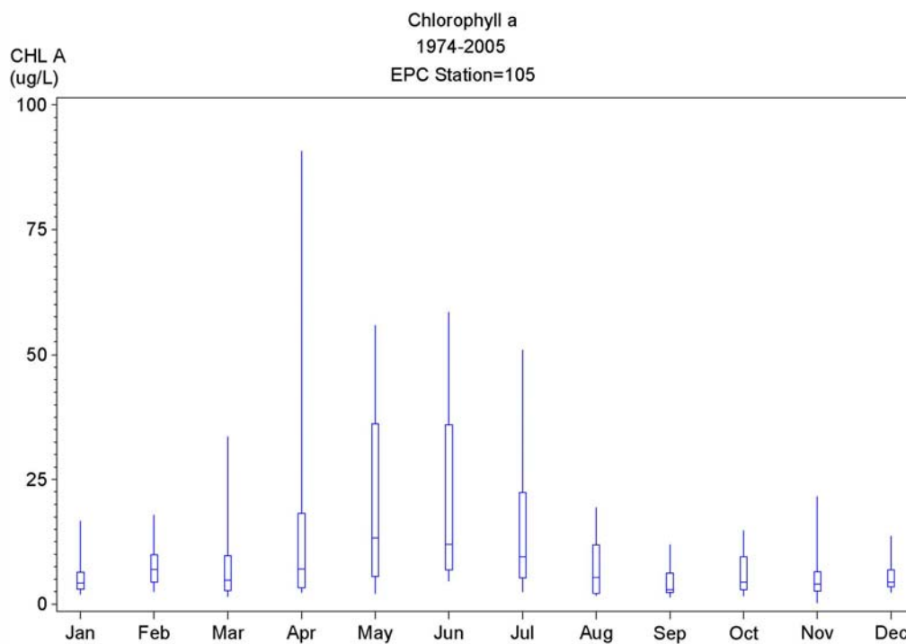
Figure 4-12 Monthly distributions of chlorophyll a at EPCHC Station 105 (near Rowlett Park) across multiple years. EPCHC chlorophyll samples are taken at mid-depth. Boxes represent the 25 th , 50 th and 75 th percentiles, while whiskers represent the 10 th and 90 th percentiles.
