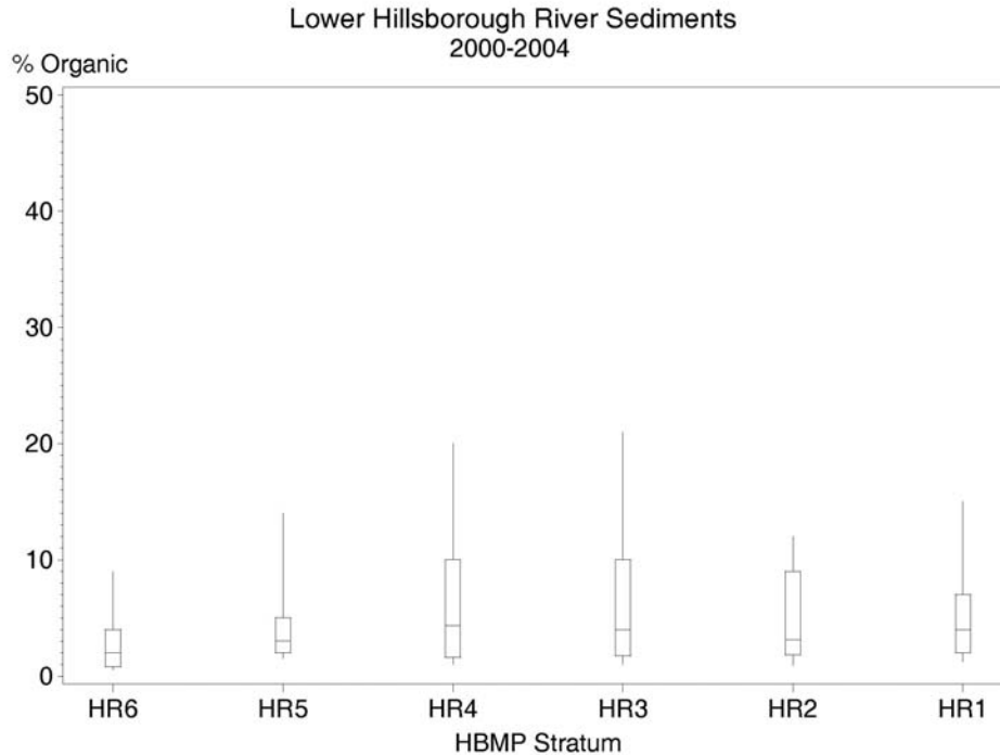
Figure 3-6 Longitudinal distribution of percent organics (=loss on ignition) in LHR sediments (From: PBS&J 2004; 2005). Stratum 1 is downstream, Stratum 6 is upstream.
