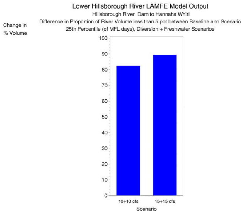
Figure 7-44 Difference in the proportion of volume less than 5 ppt between the baseline and Hannah's Whirl for the diversion scenarios (scenario - baseline), 25 th percentile of MFL days.
