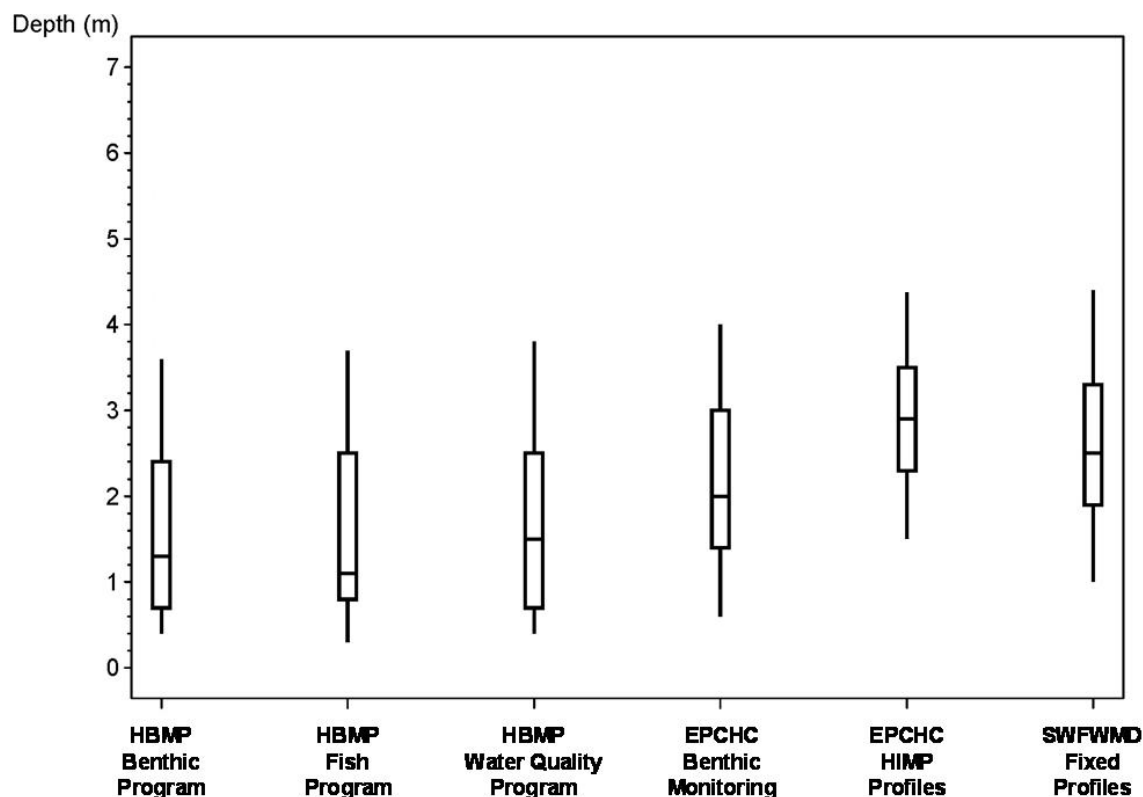
Figure 6-15 Depths reported for each monitoring program for bottom DO samples in the LHR. The boxes extend from the 25 th to 75 th percentiles, and the whiskers extend from the 5 th to 95 th percentiles.
