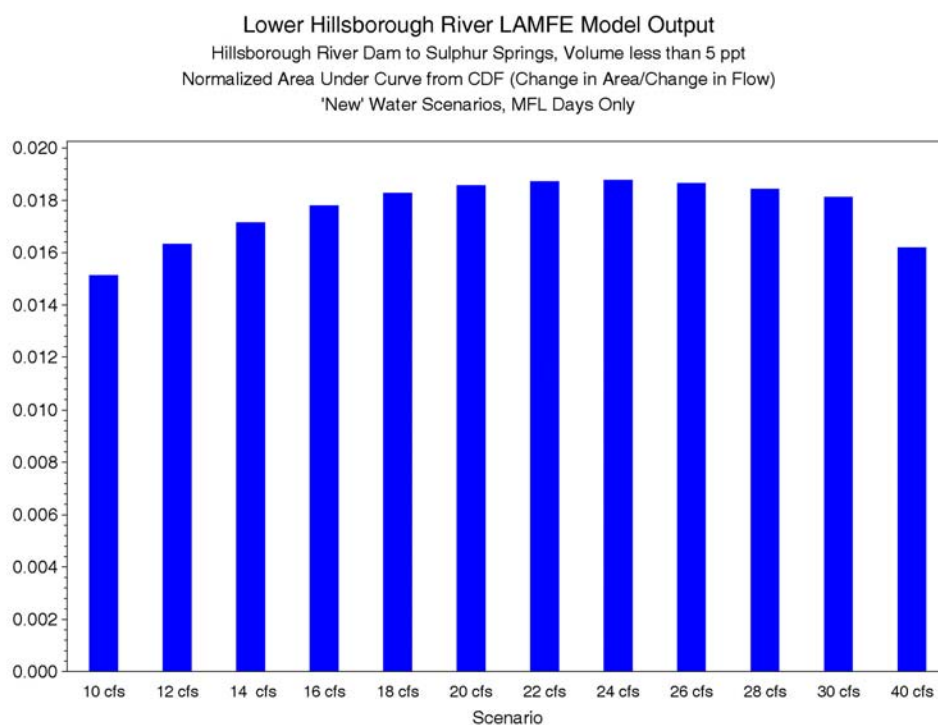
Figure 7-26 Normalized area under the curve based on CDF plot of percent volume less than 5 ppt from the dam to Sulphur Springs versus percentile of MFL days for the additional freshwater Scenarios.
