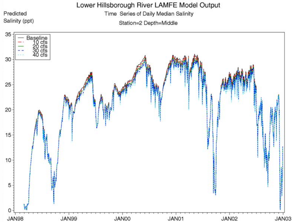
Figure 6-58 Predicted daily median salinity for the baseline and freshwater scenarios at EPCHC station 2, middle layer.
