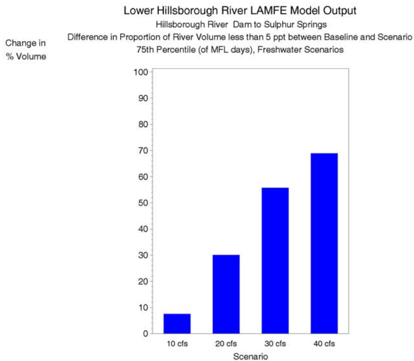
Figure 7-4 Difference in the proportion of volume less than 5 ppt between the baseline and freshwater Scenarios (Scenario - Baseline), 75 th percentile of MFL days, Dam to Sulphur Springs.
