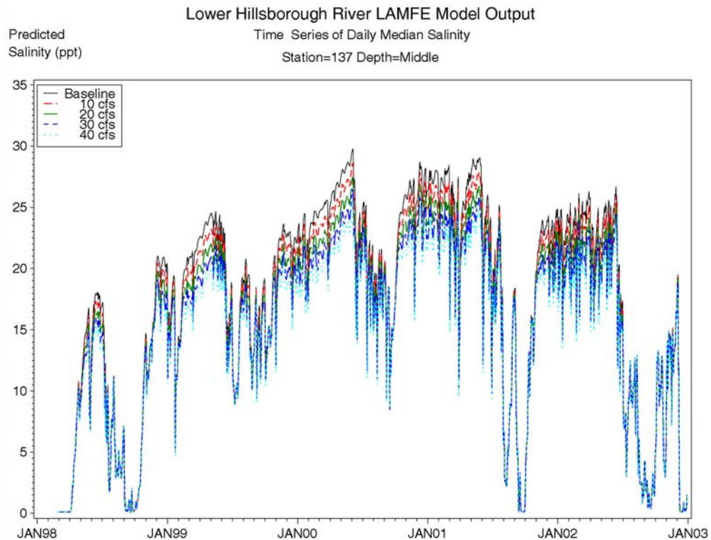
Figure 6-55 Predicted daily median salinity for the baseline and freshwater scenarios at EPCHC station 137, middle layer.
