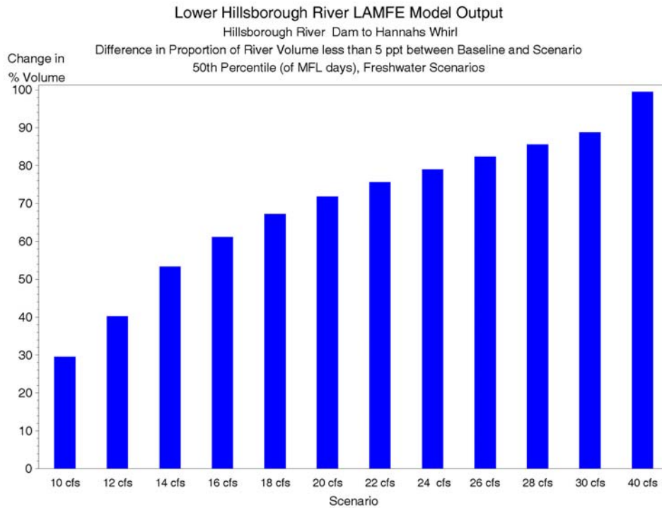
Figure 7-18 Difference in the proportion of volume less than 5 ppt between the baseline and freshwater Scenarios (Scenario - Baseline), 50 th percentile of MFL days, Dam to Hannah's Whirl.
