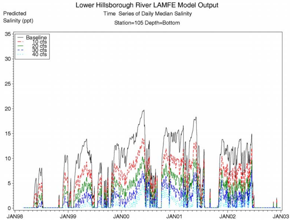
Figure 6-50 Predicted daily median salinity for the baseline and freshwater scenarios at EPCHC station 105, bottom layer.
