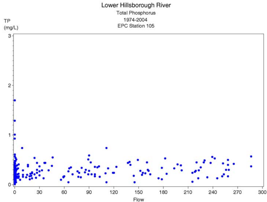
Figure 6-42 Observed response of total phosphorous concentration at EPC Station 105 as a function of flow at the Hillsborough River Dam (Dam flow + Sulphur Springs diversions to the base of the dam). Data were subset to flows less than 300 cfs and TP values less than 4 for this figure.
