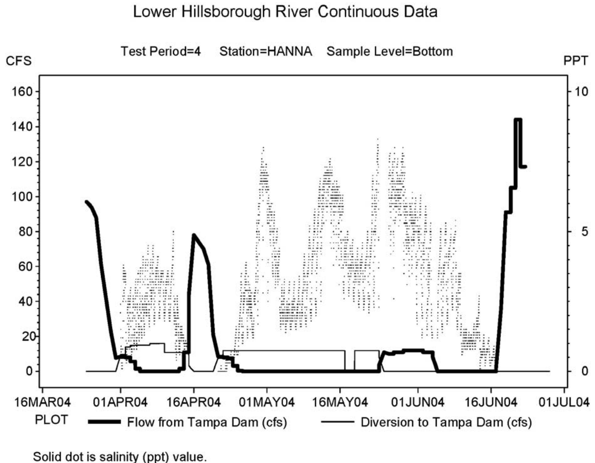
Figure 6-11 Dam flow and spring diversion flow during Test Period 4 (left axis), and observed Hannah's Whirl continuous recorder bottom salinity (right axis – solid circles).
