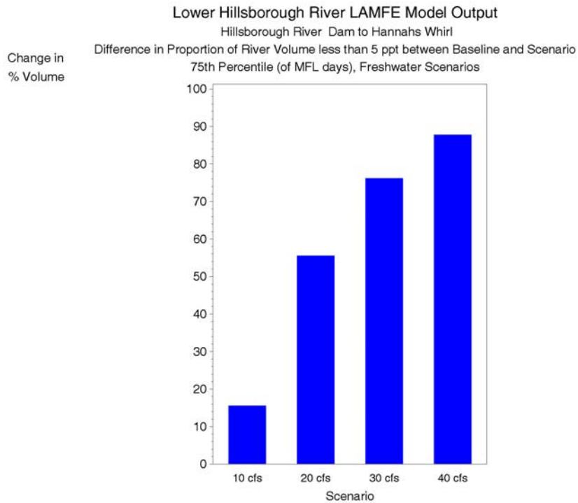
Figure 7-7 Difference in the proportion of volume less than 5 ppt between the baseline and freshwater Scenarios (Scenario - Baseline), 75 th percentile of MFL days, Dam to Hannah's Whirl.
