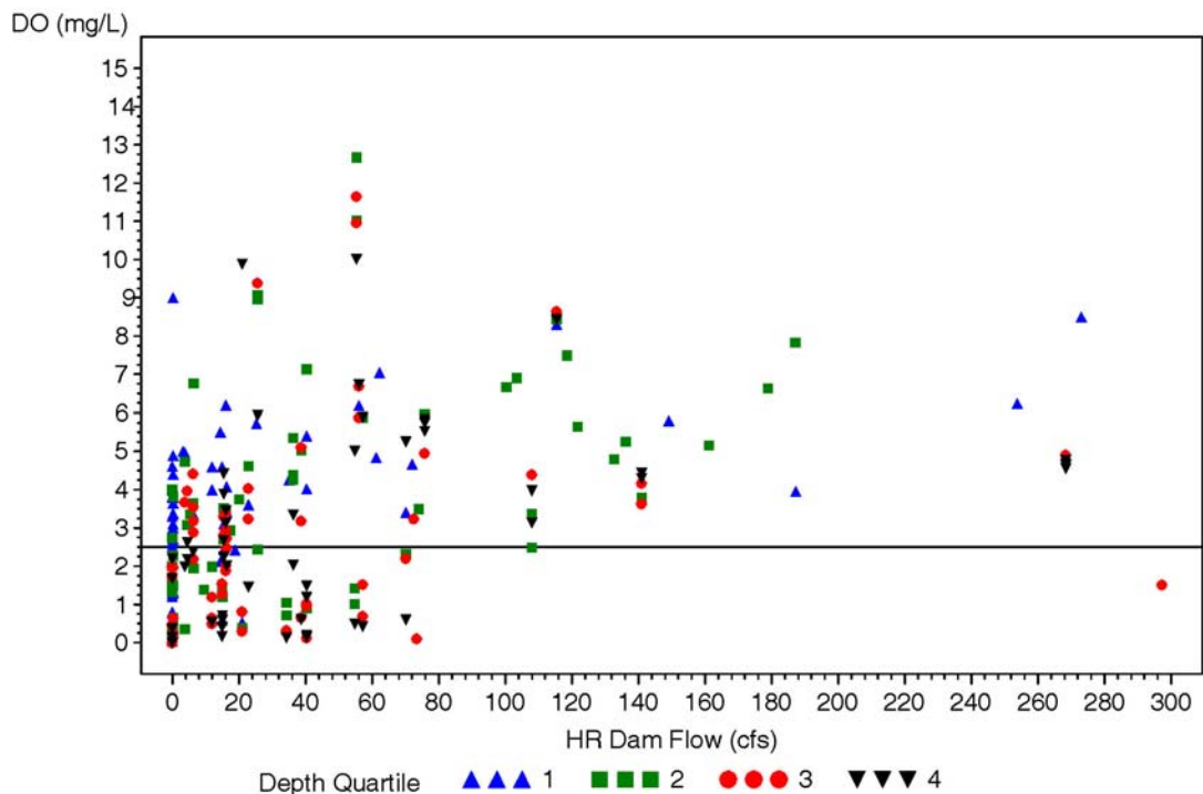
Figure 6-25d. Bottom DO for river km 13 as a function depth for dam flows between 0 and 300 cfs. Symbols are categorized by depth quartiles based on bottom area bathymetry for this region of the river.
