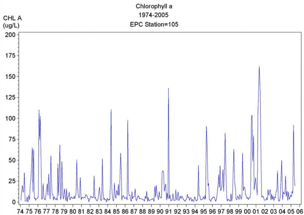
Figure 4-5 Monthly time series of chlorophyll a at EPCHC Station 105 (near Rowlett Park).
