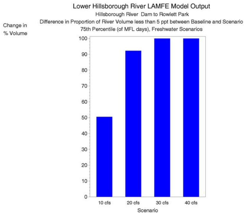
Figure 7-10 Difference in the proportion of volume less than 5 ppt between the baseline and freshwater Scenarios (Scenario - Baseline), 75 th percentile of MFL days, Dam to Rowlett Park.
