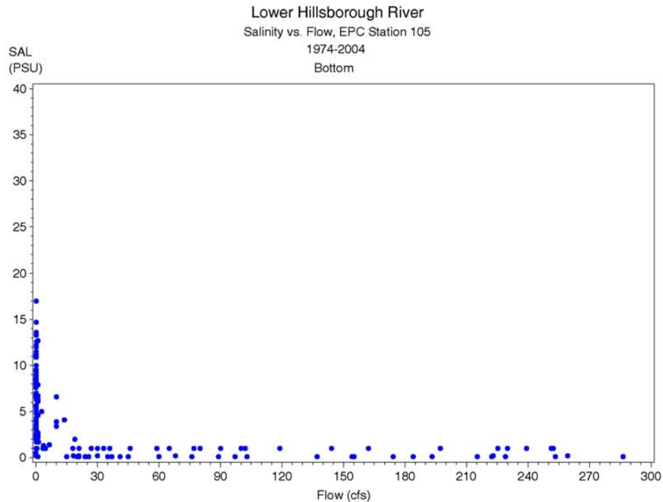
Figure 6-5 Long term EPCHC bottom salinity observations at EPC Station 105 as a function of flow at the Hillsborough River Dam (Dam flow + Sulphur Springs diversions to the base of the dam). Data subset to flows less than 300 cfs for this figure.
