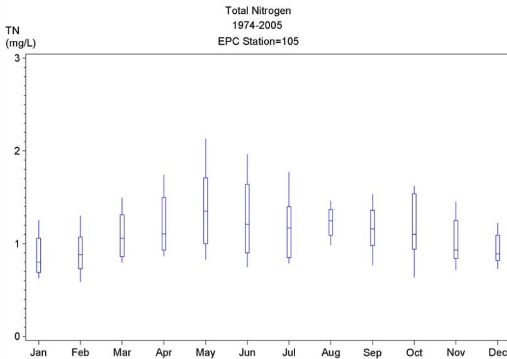
Figure 4-13 Monthly distributions of total nitrogen at EPCHC Station 105 (near Rowlett Park) across multiple years.
