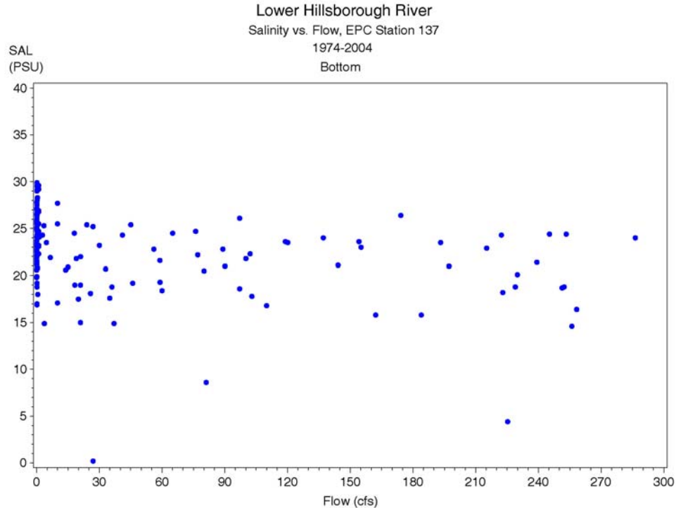
Figure 6-6 Long term EPCHC bottom salinity observations at EPC Station 137 as a function of flow at the Hillsborough River Dam (Dam flow + Sulphur Springs diversions to the base of the dam). Data subset to flows less than 300 cfs for this figure.
