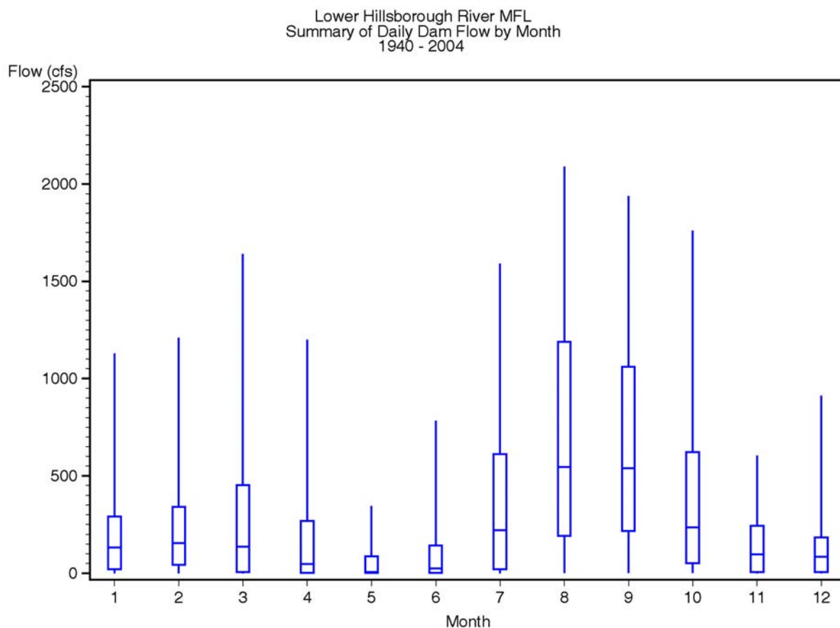
Figure 2-9 Box and whisker plot of daily Hillsborough River Dam flows by calendar month, 1940-2004. Whiskers represent the 5 th and 95 th percentiles.
