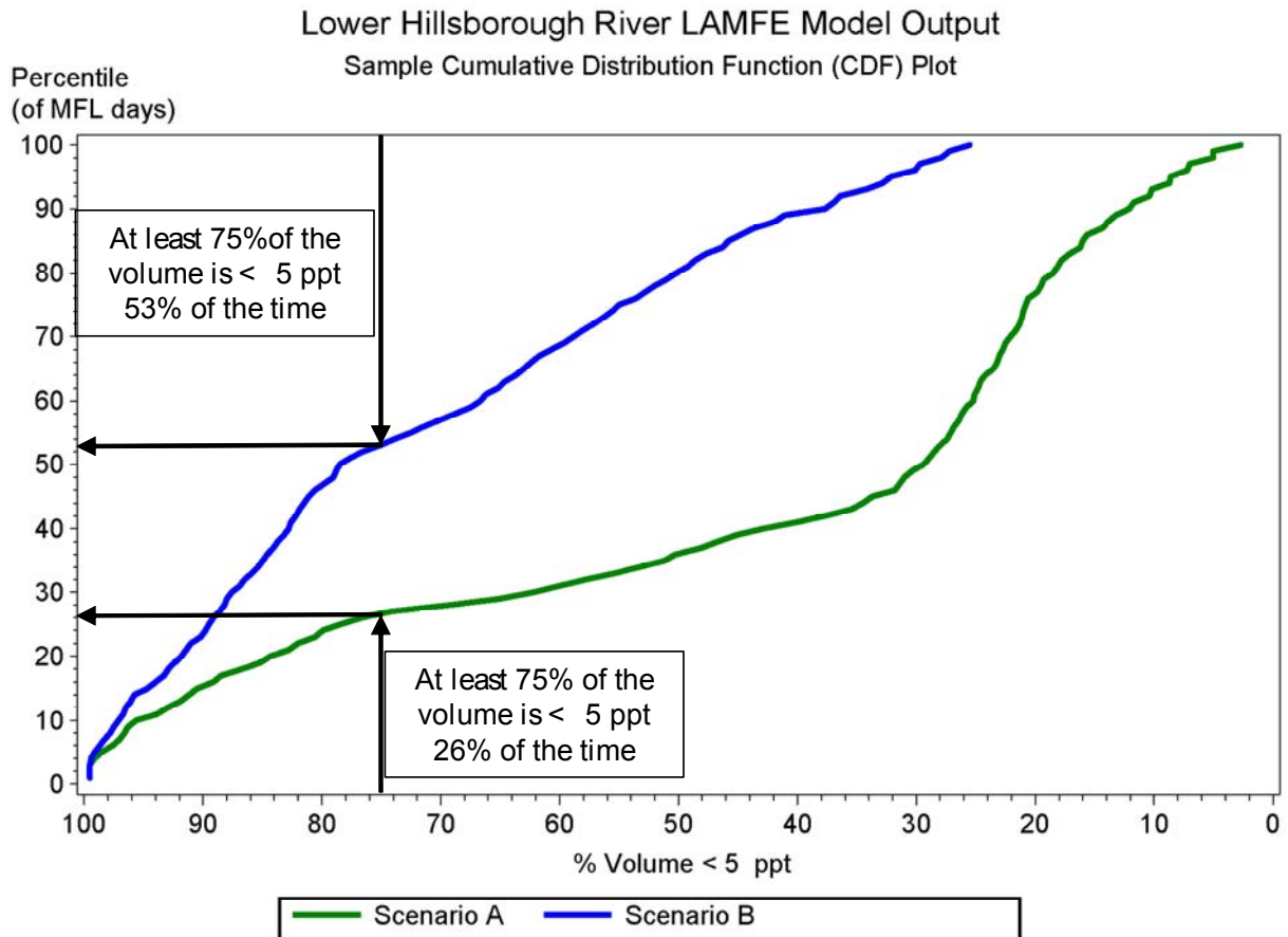
Figure 7-1a Example CDF plot. See discussion above.
