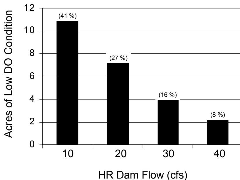
Figure 6-24 Acres of bottom DO < 2.5 mg/L between Km 14 and the dam as a function of dam flow. Corresponding percent of bottom habitat in this region of the river indicated in parentheses.
