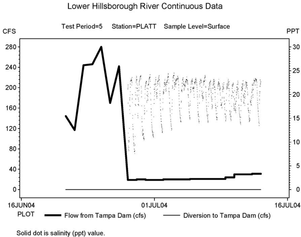
Figure 6-12 Dam flow and spring diversion flow during Test Period 5 (left axis), and observed Plat Street continuous recorder surface salinity (right axis – solid circles).
