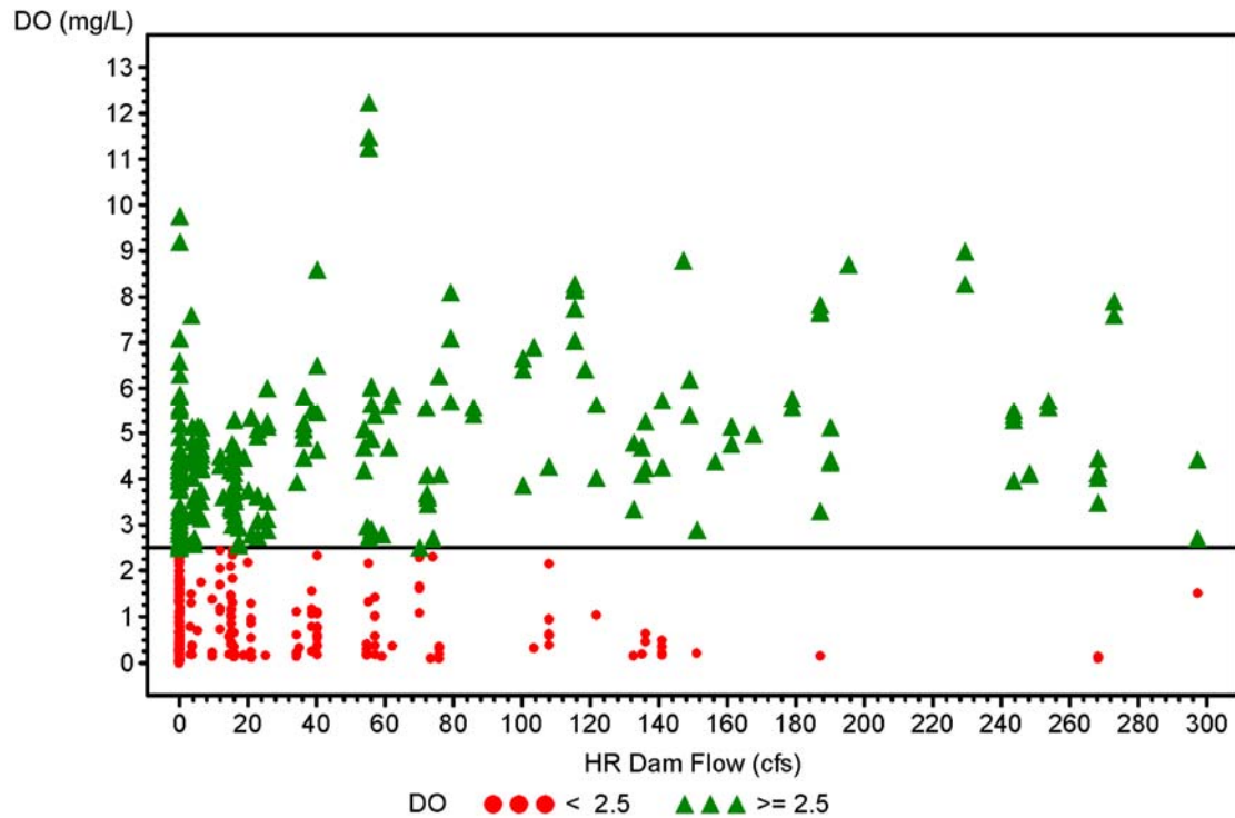
Figure 6-16 Bottom DO in LHR Stratum 5 (approximately from Sligh Avenue to Sulphur Springs) as a function of dam flow.
