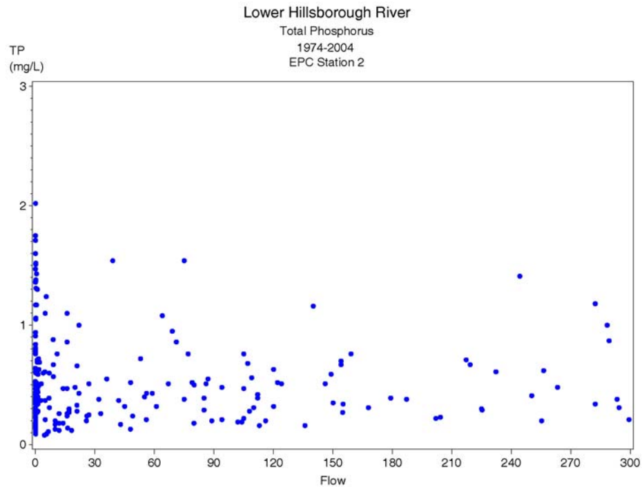
Figure 6-44. Observed response of total phosphorous concentration at EPC Station 2 as a function of flow at the Hillsborough River Dam (Dam flow + Sulphur Springs diversions to the base of the dam). Data were subset to flows less than 300 cfs and TP values less than 4 for this figure.
