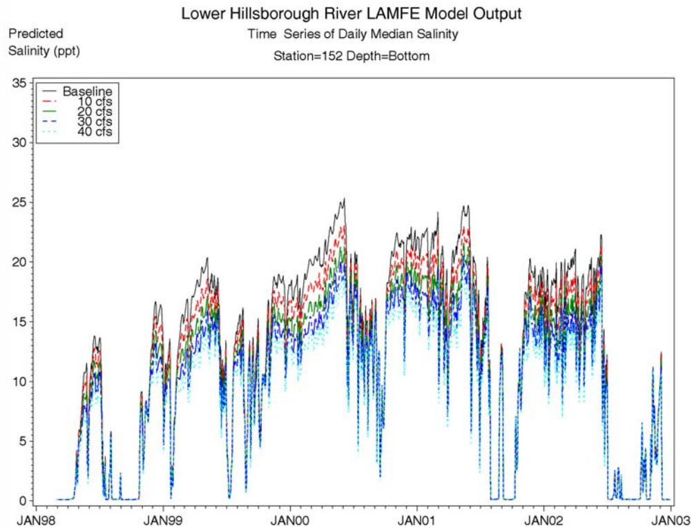
Figure 6-53 Predicted daily median salinity for the baseline and freshwater scenarios at EPCHC station 152, bottom layer.
