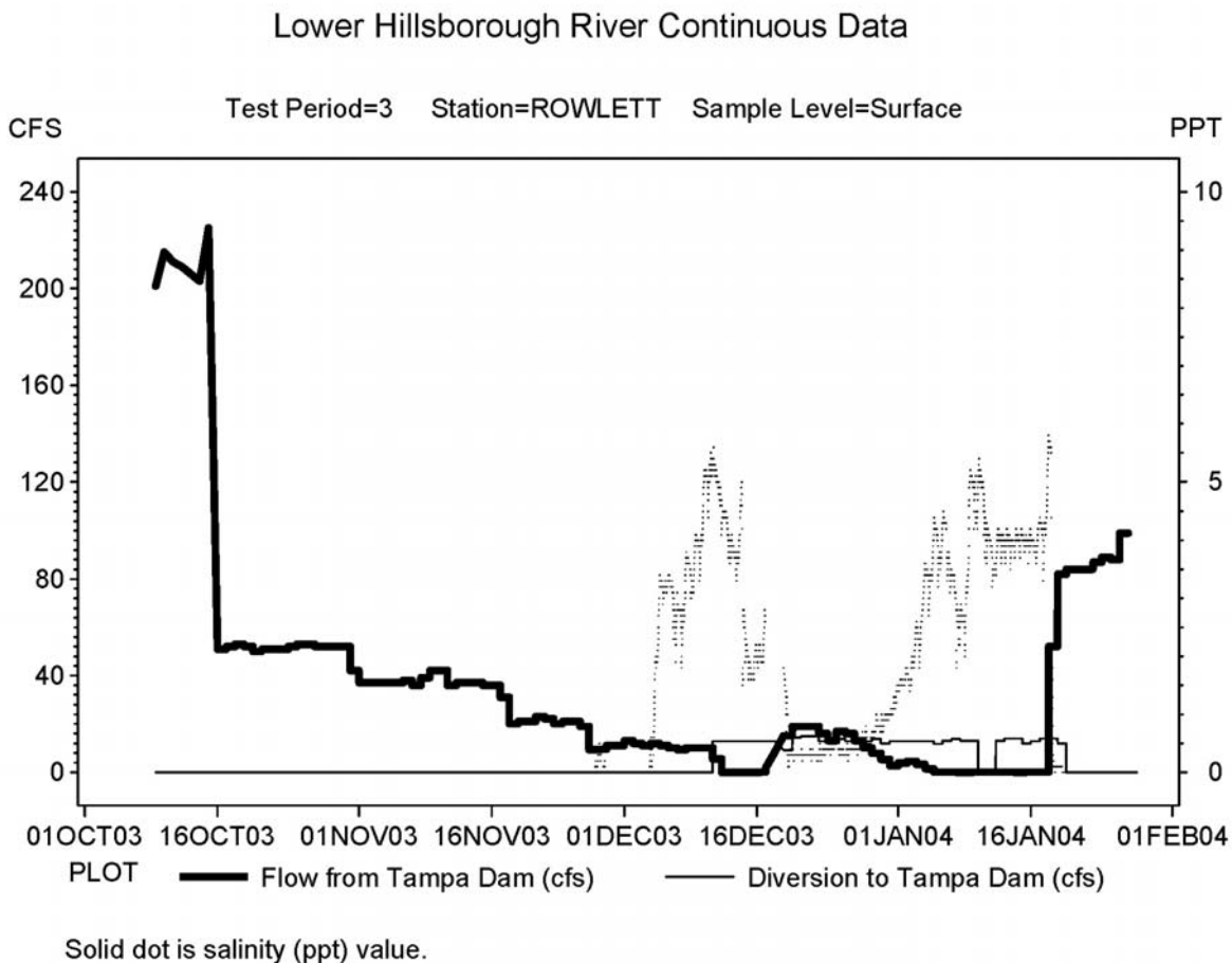
Figure 6-10 Dam flow and spring diversion flow during Test Period 3 (left axis), and observed Rowlett Park continuous recorder surface salinity (right axis – solid circles).
