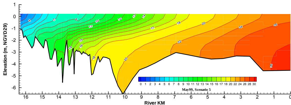
Figure 6-61 Predicted monthly median salinity for the 10 cfs freshwater Scenario, May 1999.
