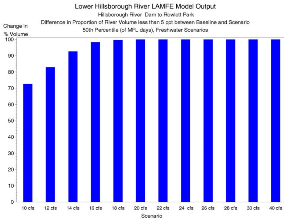
Figure 7-21 Difference in the proportion of volume less than 5 ppt between the baseline and freshwater Scenarios (Scenario - Baseline), 50 th percentile of MFL days, Dam to Rowlett Park.
