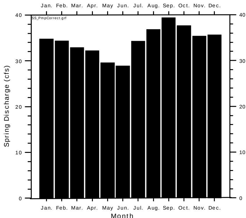
Figure 2-12 Average monthly flows from Sulphur Springs corrected for withdrawals for 1991 – 2002. (Source: SWFWMD, 2004b)
