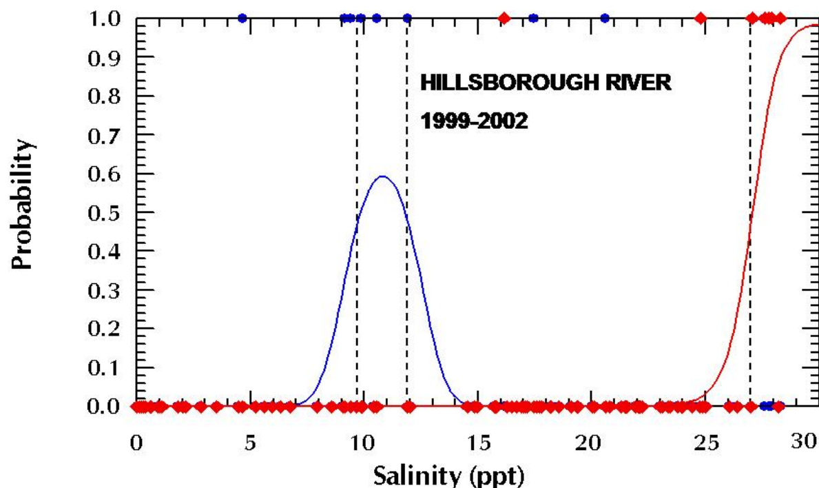
Figure 5-4. Probability of occurrence vs. wet season salinity (binary logistic regression) of species assemblages identified in numerical classification analysis (From: Grabe et al. 2004).
