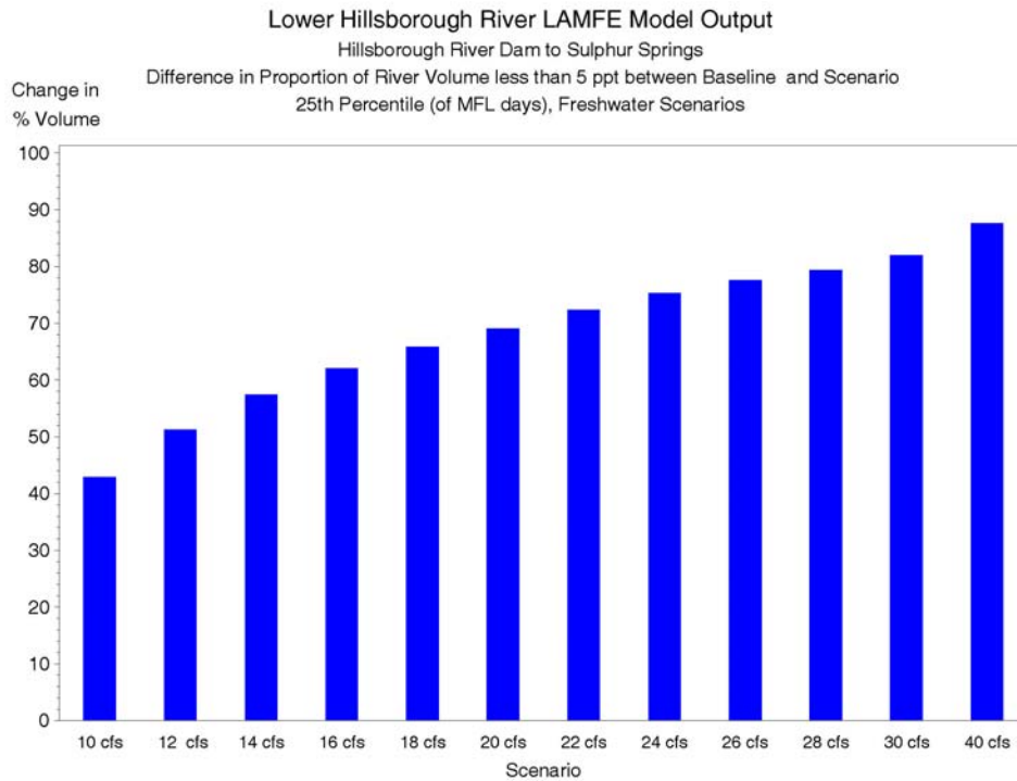
Figure 7-14 Difference in the proportion of volume less than 5 ppt between the baseline and freshwater Scenarios (Scenario - Baseline), 25 th percentile of MFL days, Dam to Sulphur Springs.
