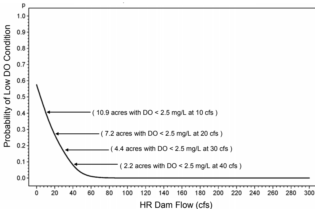
Figure 6-23 Probability of bottom DO < 2.5 mg/L between Km 14 and the dam as a function of dam flow (calculated as the mean of estimates by 0 th , 25 th , 50 th , 75 th , and 100 th depth percentile). For reference, the probabilities are expressed as acres of river bottom for several example flow values (more precisely, the probabilities represent joint probabilities over time and space).
