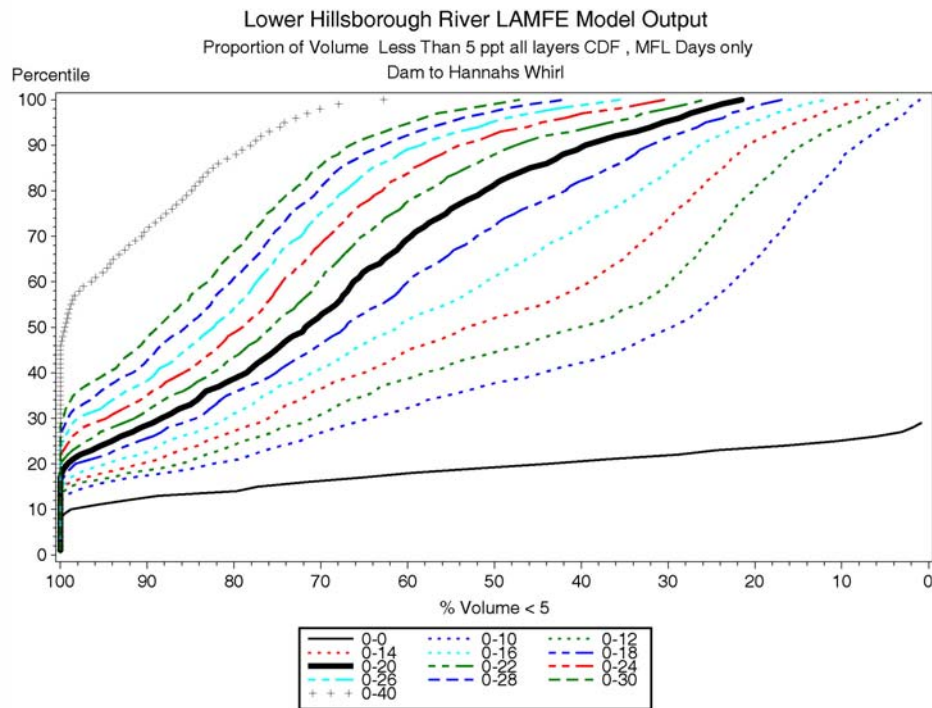
Figure 7-24 CDF plot of percent volume less than 5 ppt from the dam to Hannah's Whirl versus percentile of MFL days for the additional freshwater Scenarios.
