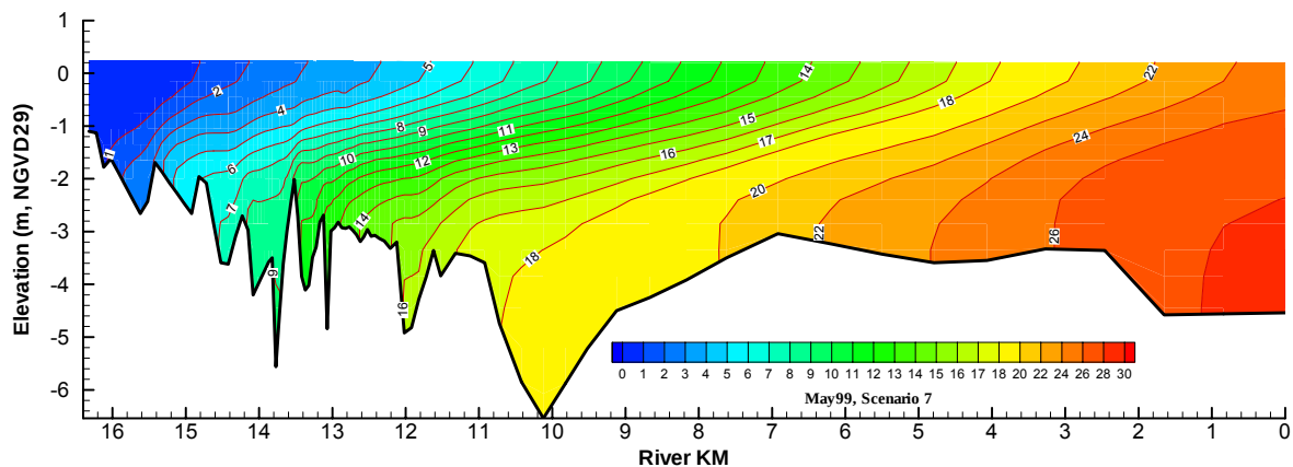
Figure 6-63 Predicted monthly median salinity for the 30 cfs freshwater Scenario, May 1999.
