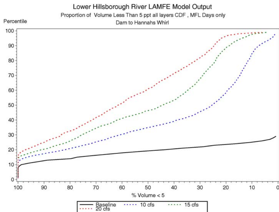
Figure 7-39 CDF plot of percent volume less than 5 ppt between dam and Hannah's Whirl versus percentile of MFL days for Sulphur Springs diversion scenarios.
