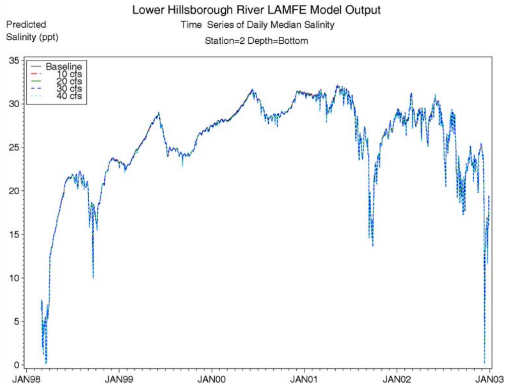
Figure 6-59 Predicted daily median salinity for the baseline and freshwater scenarios at EPCHC station 2, bottom layer.
