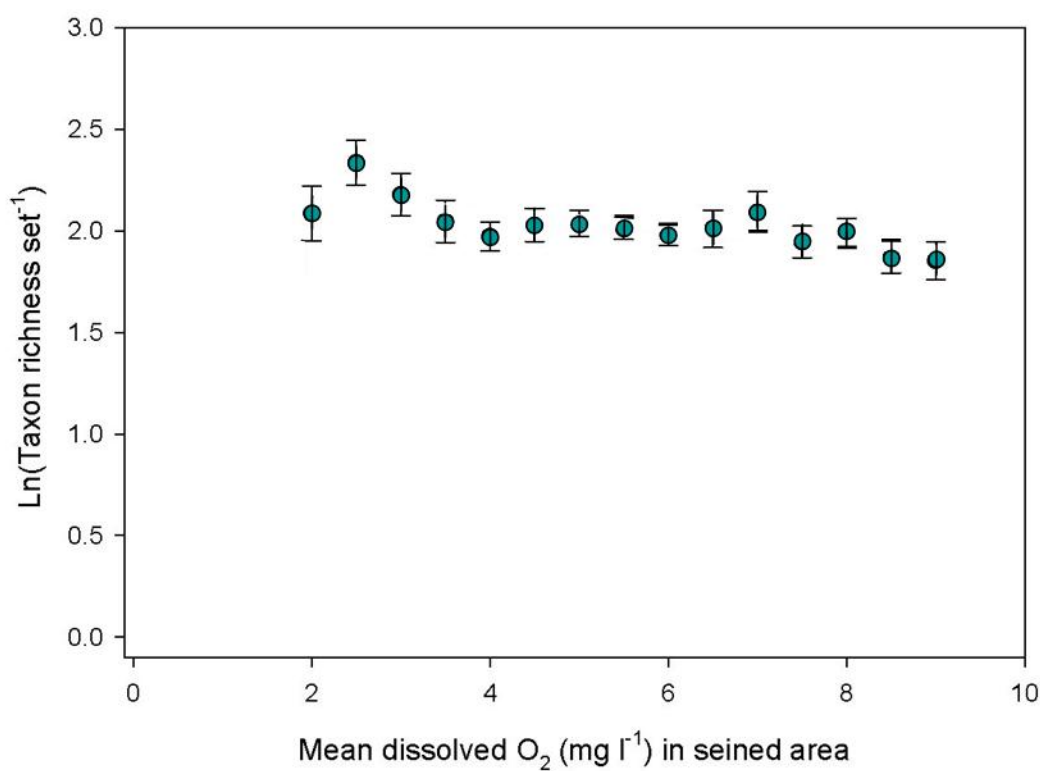
Figure 5-23 Linear relationship between mean taxon richness in seines and dissolved oxygen in the HR (Figure adapted from MacDonald et al. , 2005).
