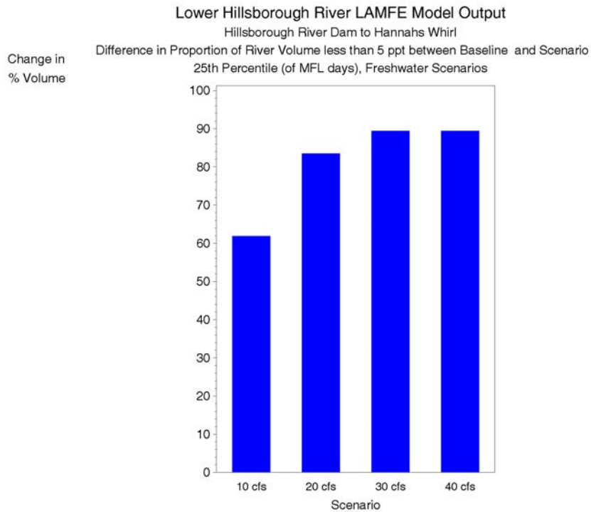
Figure 7-5 Difference in the proportion of volume less than 5 ppt between the baseline and freshwater Scenarios (Scenario - Baseline), 25 th percentile of MFL days, Dam to Hannah's Whirl.
