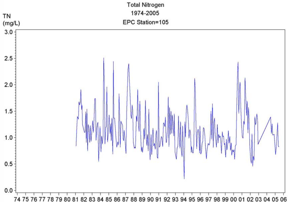
Figure 4-6 Monthly time series of total nitrogen at EPCHC Station 105 (near Rowlett Park).
