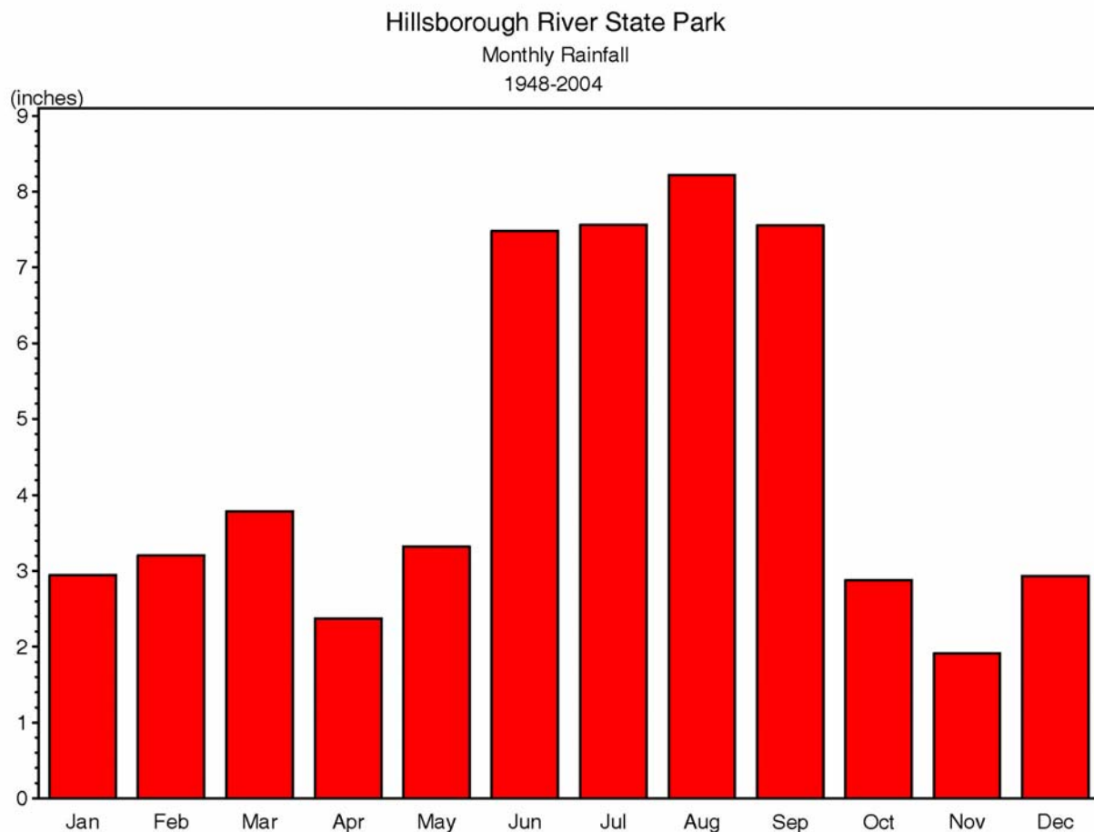
Figure 2-4 Mean monthly rainfall (total inches) at the Hillsborough River State park, 1948-2004.
