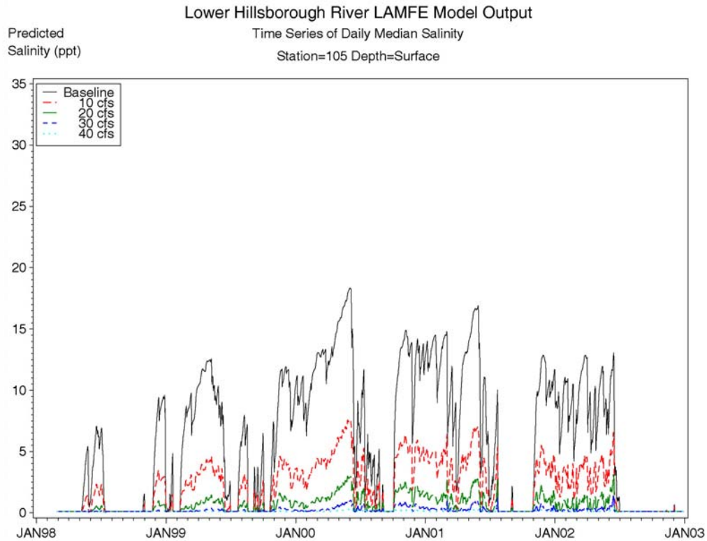
Figure 6-48 Predicted daily median salinity for the baseline and freshwater scenarios at EPCHC station 105, surface layer.
