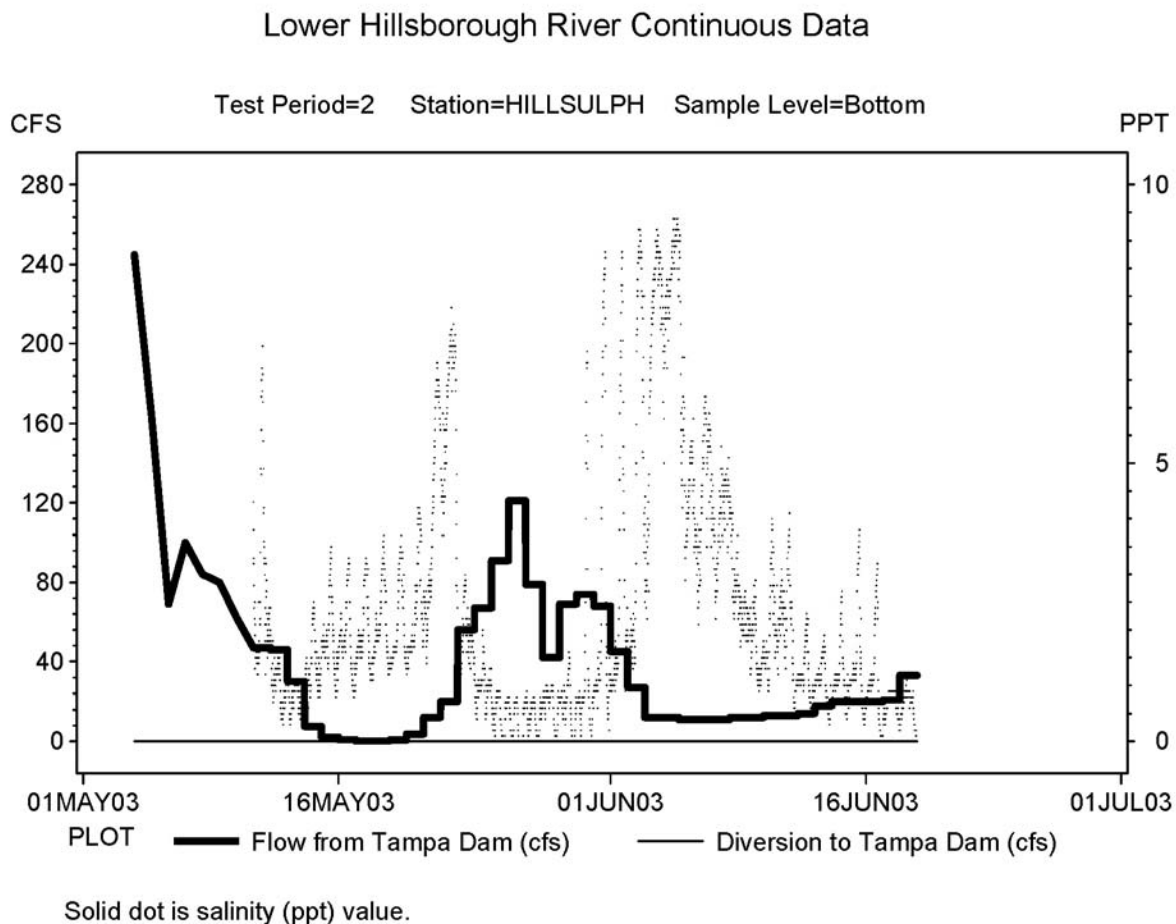
Figure 6-9 Dam flow and spring diversion flow during Test Period 2 (left axis), and observed Hillsborough River at Sulphur Springs continuous recorder bottom salinity (right axis – solid circles).
