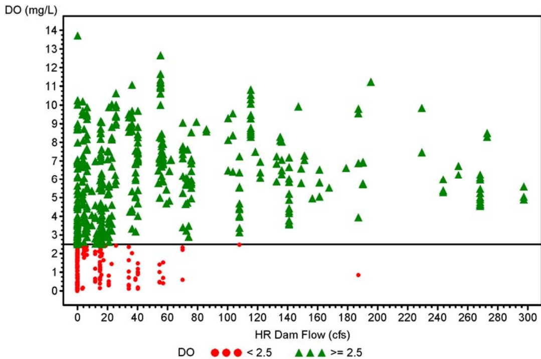
Figure 6-17 Bottom DO in LHR Stratum 6 (approximately from Sulphur Springs to the dam) as a function of dam flow.
