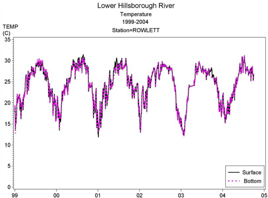
Figure 4-18 Observed USGS/District continuous recorder time series of surface and bottom temperature at Rowlett Park.
