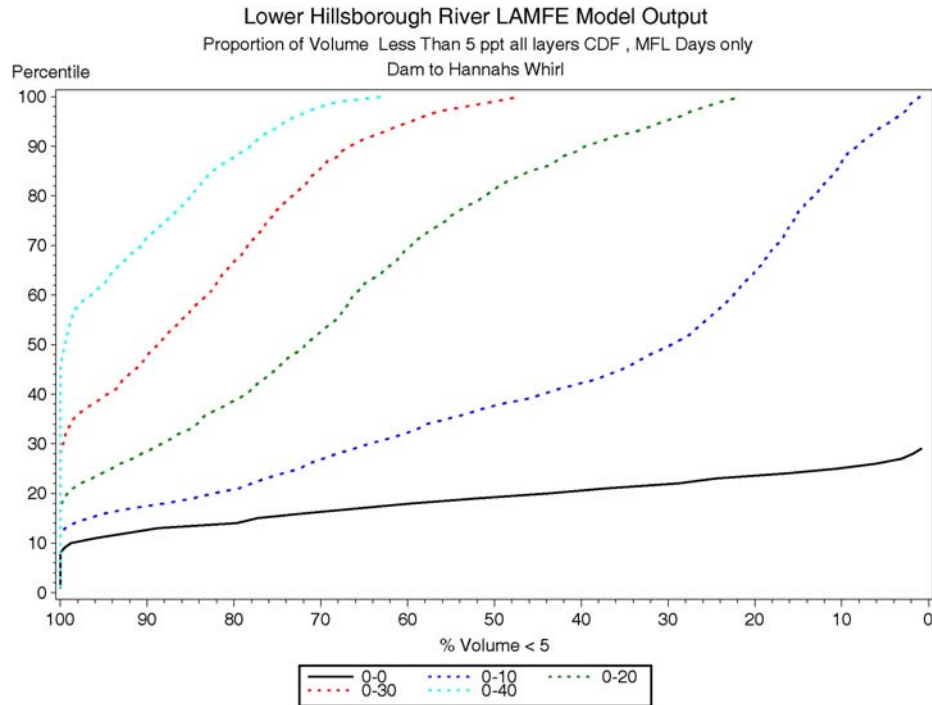
Figure 7-12 CDF plot of percent volume from the dam to Hannah's Whirl less than 5 ppt for MFL days for freshwater scenarios.
