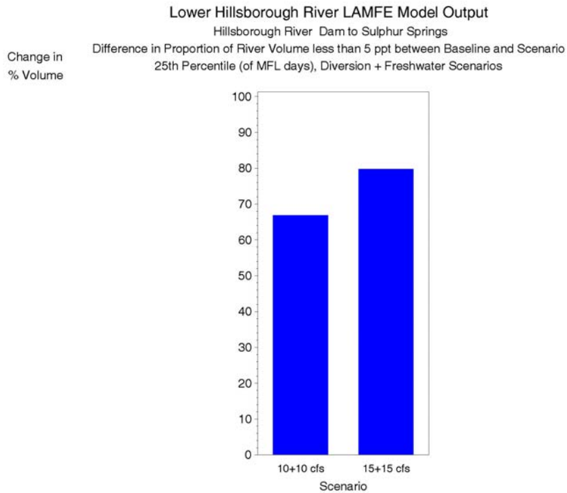
Figure 7-41 Difference in the proportion of volume less than 5 ppt between the baseline and Sulphur Springs for the diversion scenarios (scenario - baseline), 25 th percentile of MFL days.
