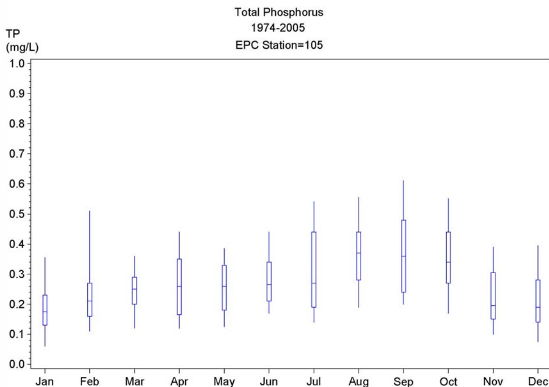
Figure 4-14 Monthly distributions of total phosphorous at EPCHC Station 105 (near Rowlett Park) across multiple years.
