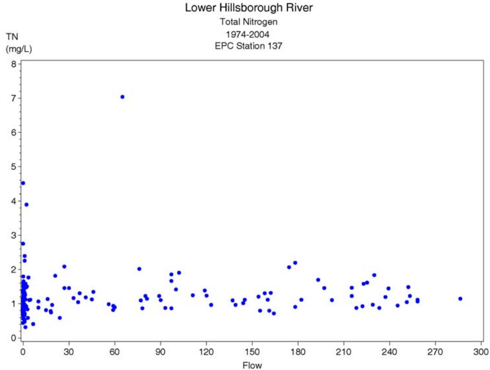
Figure 6-40. Observed response of total nitrogen concentration at EPC 137 as a function of flow at the Hillsborough River Dam (Dam flow + Sulphur Springs diversions to the base of the dam). Data were subset to flows less than 300 cfs for this figure.
