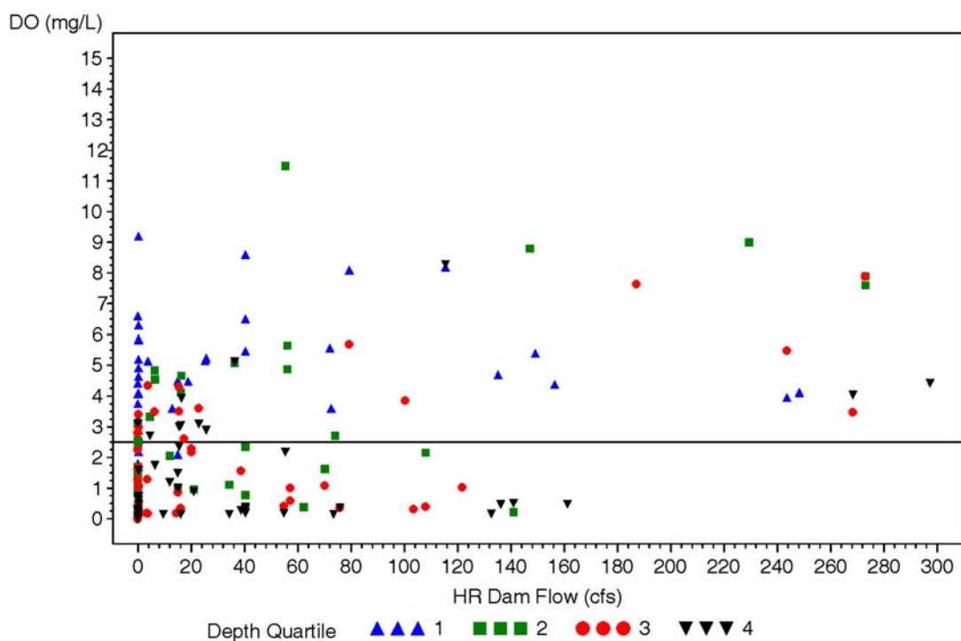
Figure 6-25b. Bottom DO for river km 11 as a function depth for dam flows between 0 and 300 cfs. Symbols are categorized by depth quartiles based on bottom area bathymetry for this region of the river.
