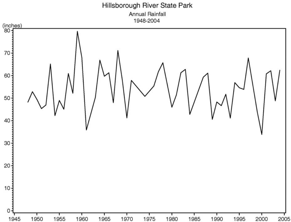
Figure 2-5 Annual rainfall (inches) at Hillsborough River State Park, 1948-2004.
