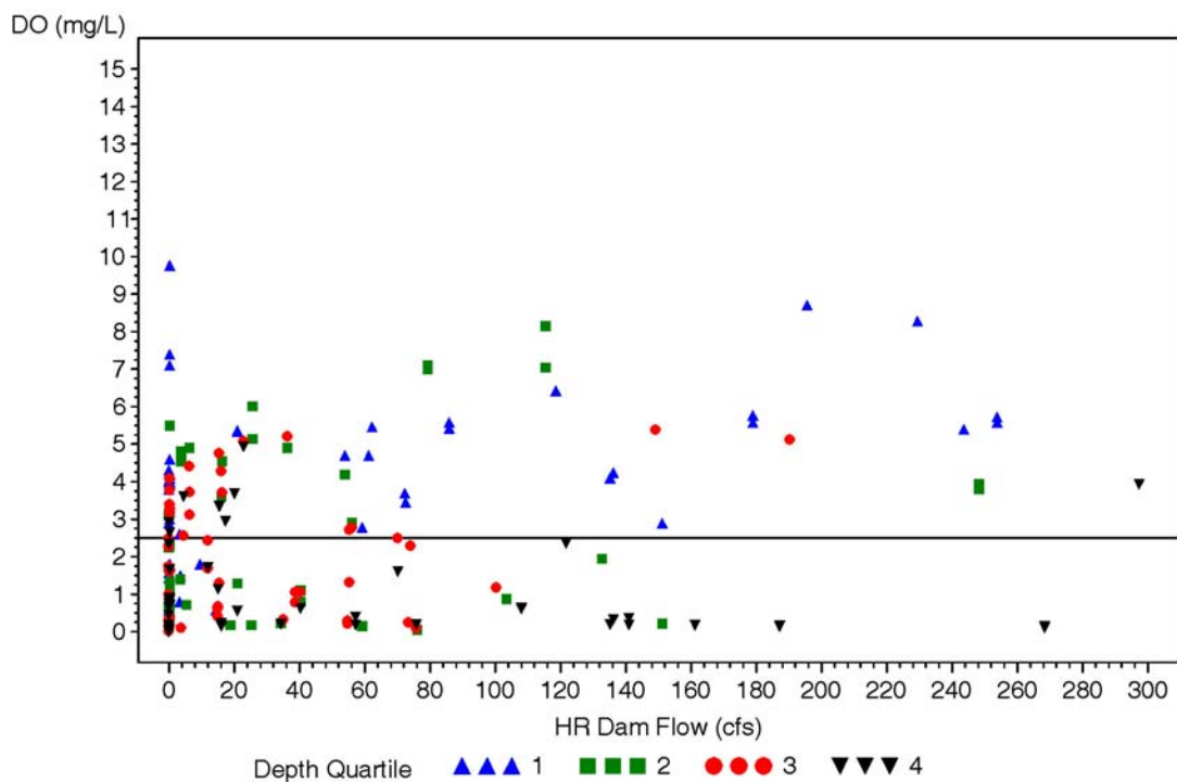
Figure 6-25a. Bottom DO for river km 10 as a function depth for dam flows between 0 and 300 cfs. Symbols are categorized by depth quartiles based on bottom area bathymetry for this region of the river.
