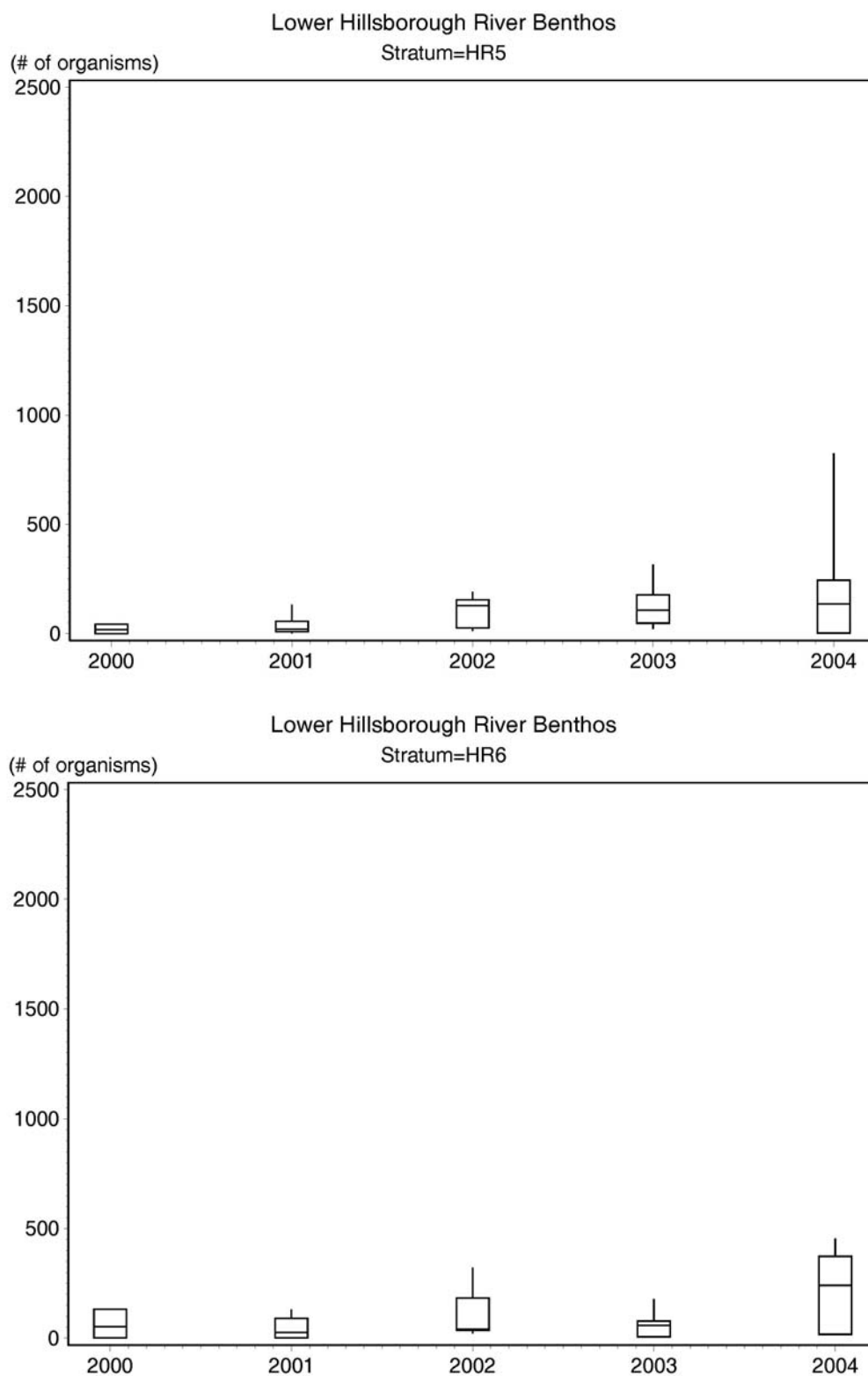
Figure 5-7. Total numbers of benthic macroinvertebrates m^{-2} in Lower Hillsborough River HBMP strata 5 and 6, by year, 2000-2004.
