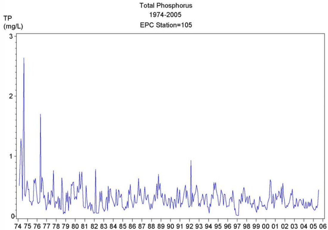
Figure 4-7 Monthly time series of total phosphorous at EPCHC Station 105 (near Rowlett Park).
