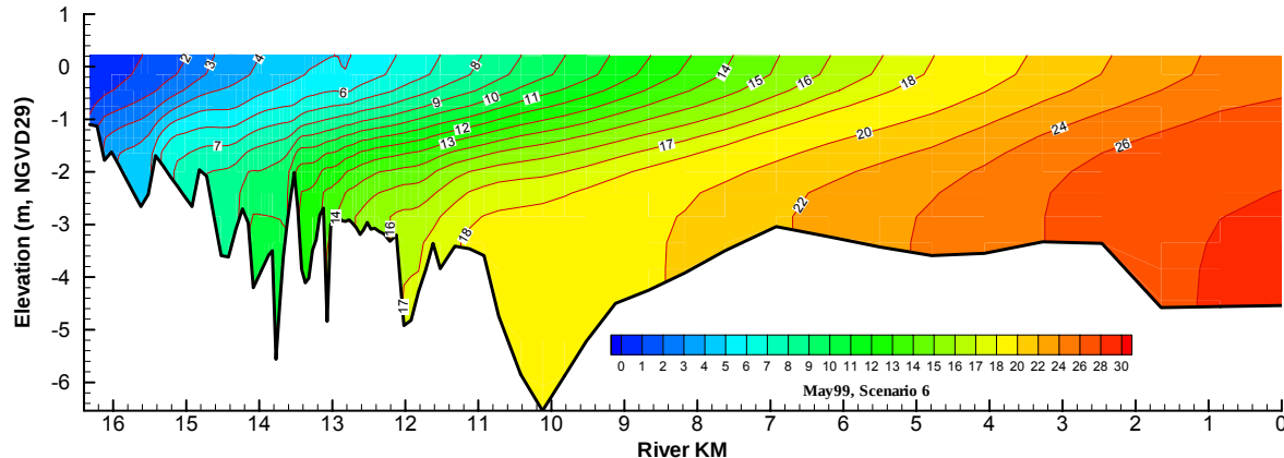
Figure 6-62 Predicted monthly median salinity for the 20 cfs freshwater Scenario, May 1999.
