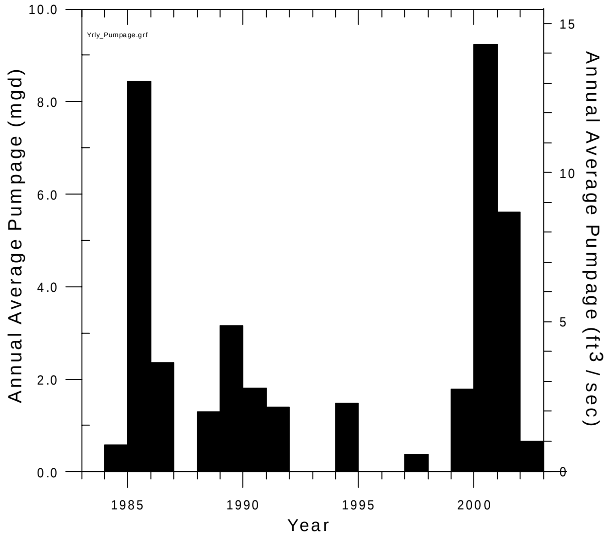
Figure 2-14 Average annual pumpage rates from Sulphur Spring by the City of Tampa for 1984-2002. (From: SWFWMD, 2004b)
