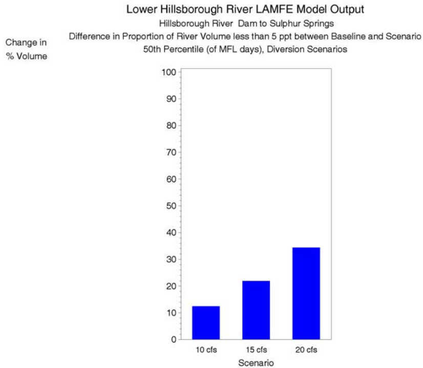
Figure 7-30 Difference in the proportion of volume less than 5 ppt between the baseline and Sulphur Springs diversion scenarios (scenario - baseline), 50 th percentile of MFL days.
