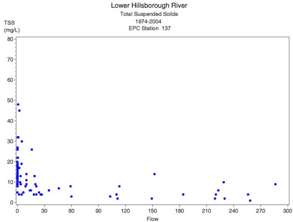
Figure 6-46. Observed response of total suspended solids concentration at EPC Station 137 as a function of flow at the Hillsborough River Dam (Dam flow + Sulphur Springs diversions to the base of the dam). Data were subset to flows less than 300 cfs.
