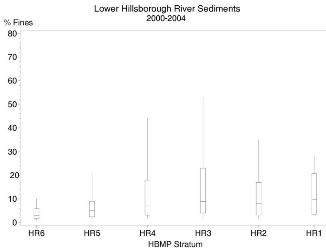
Figure 3-5 Longitudinal distribution of percent fines (=silt+clay) in LHR sediments, 2000-2004. (From: PBS&J 2004; 2005). Stratum 1 is downstream, Stratum 6 is upstream.
