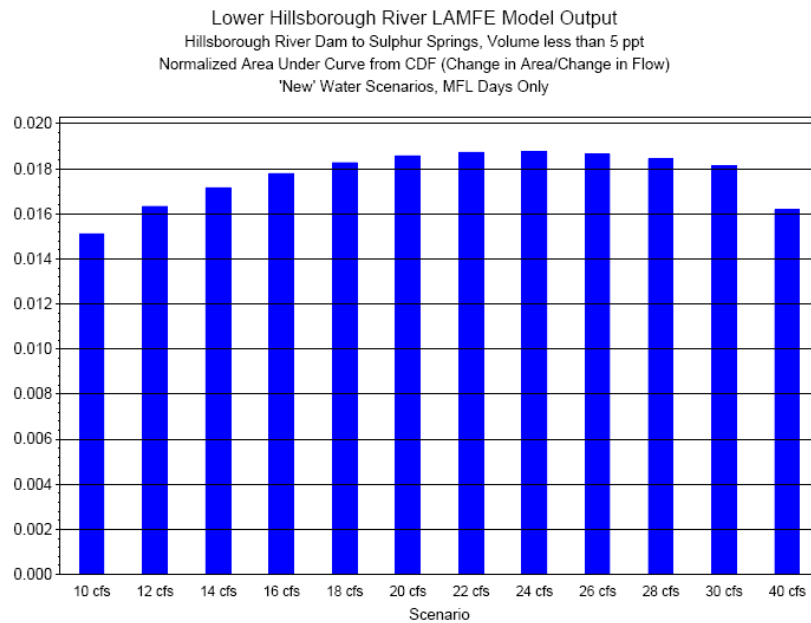
Figure 8.1. Difference in rate of change in unit area per unit flow from Hillsborough River Dam to Sulphur Springs as flow is increased in 2 cfs increments.
