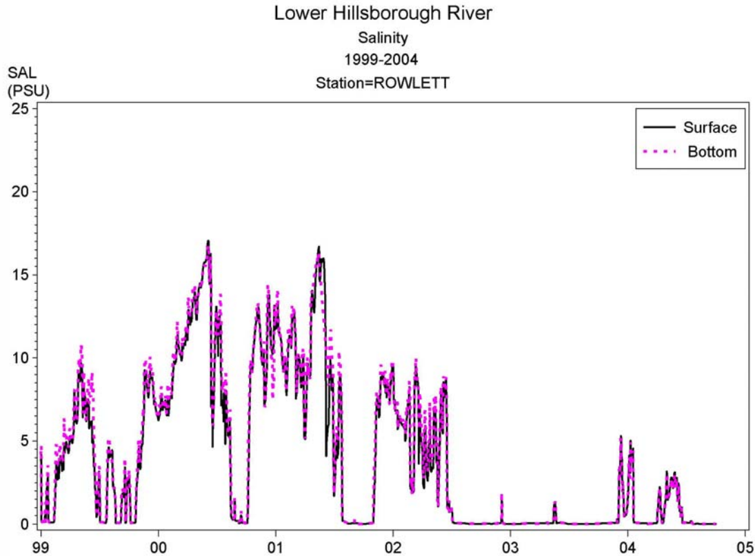
Figure 4-16 Observed USGS/District continuous recorder time series of surface and bottom salinity at Rowlett Park.
