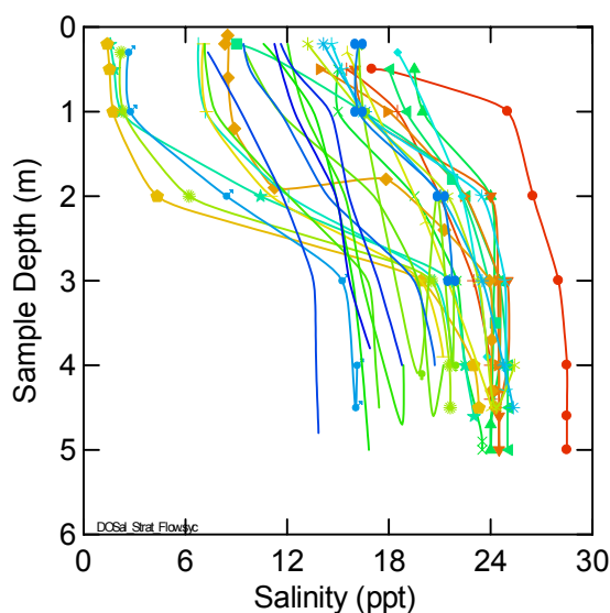
Figure 3-12 Salinity Profiles : Flows \geq 180 cfs and Depth > 3 m (Segment 3)
