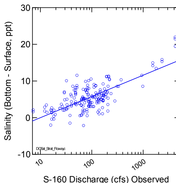
Figure 3-11 Salinity Stratification vs S-160 Flow (Segment 3)
