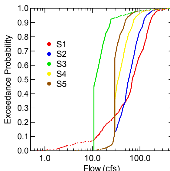
Figure 3-20 Flow Scenario CDFs (2001-2004) [View is trimmed 0.5 - 500 cfs]
