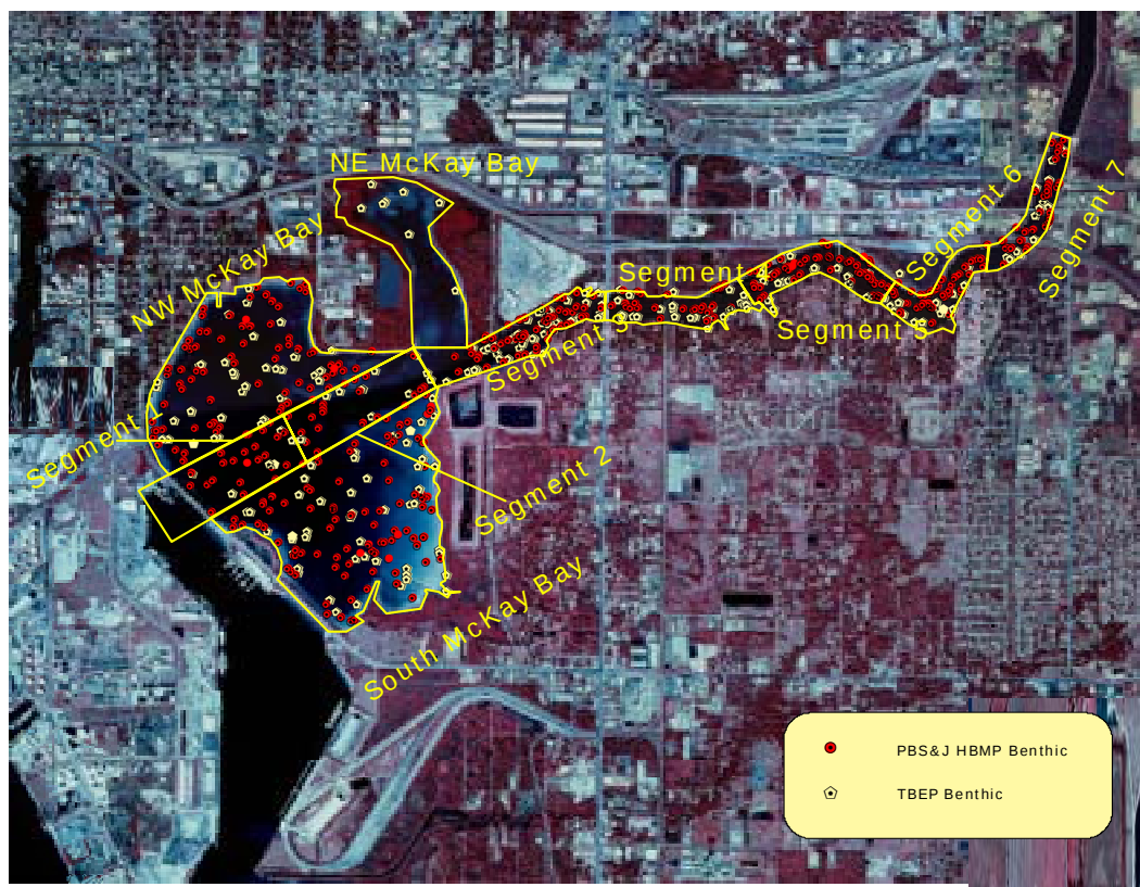
Figure 2-15 TBEP/EPCHC HIMP and PBS&J Benthic Stations
