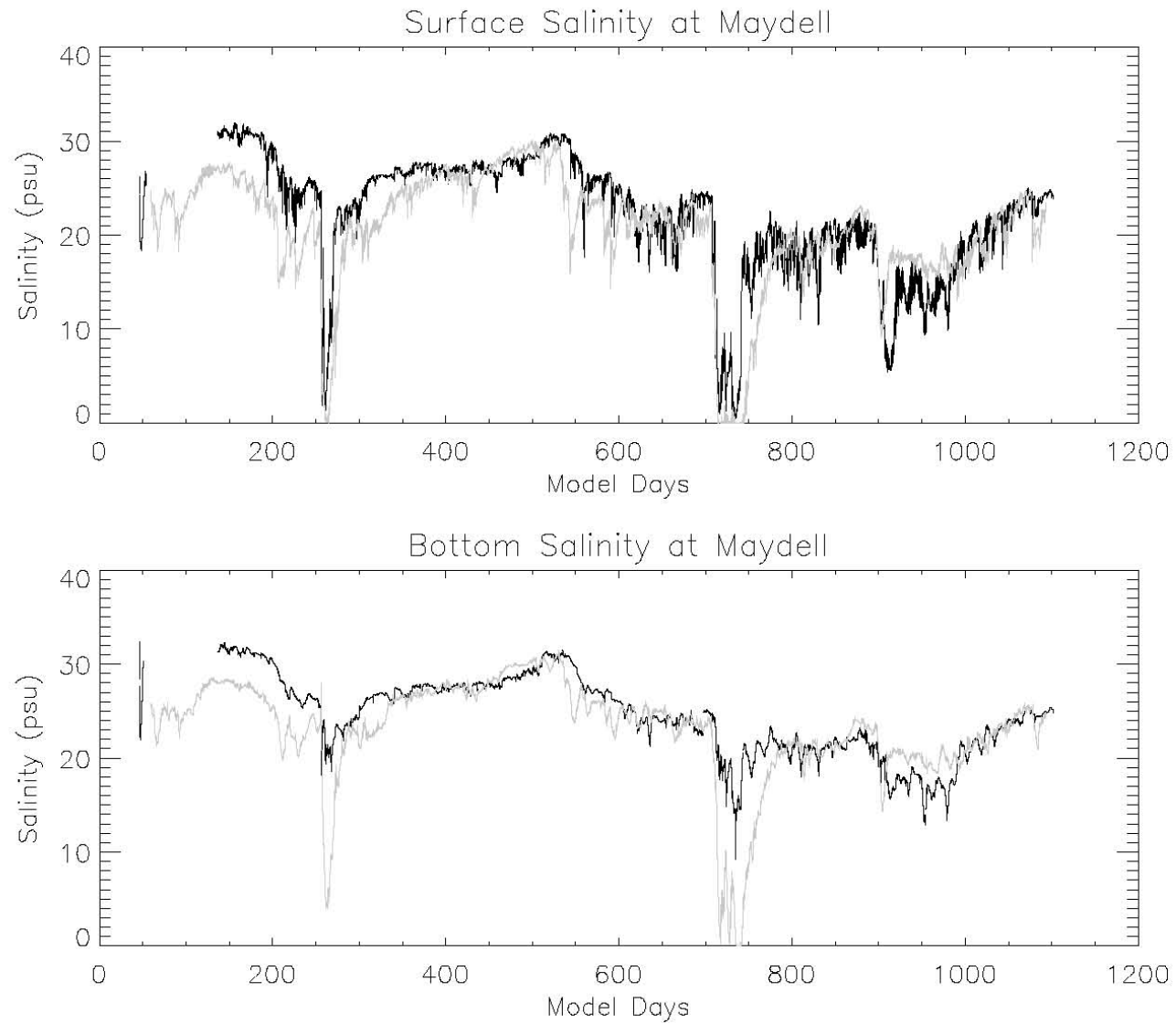
Figure 3-24 Modeled (grey) and Observed (black) Salinity at Maydell Drive (2001-2003)
