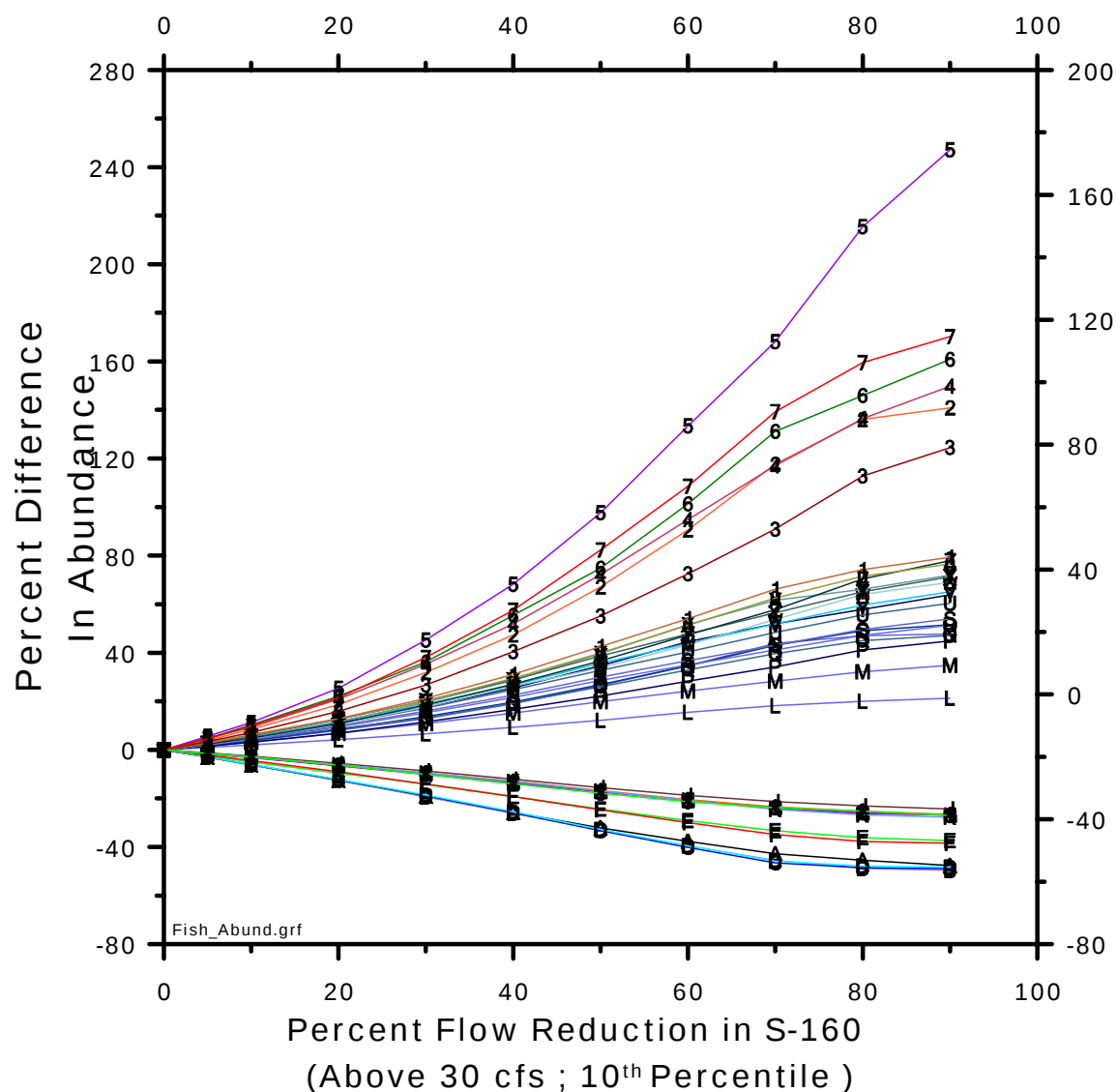
Figure 3-7 Change in Abundance as a Function of Reduced Flows - All Taxa
