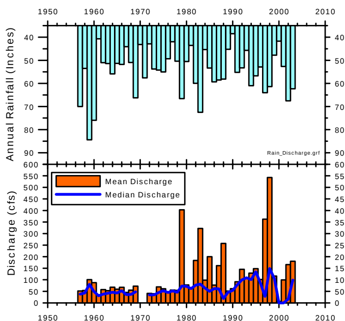
Figure 2-7 Historical Rainfall and Discharge for S-160
