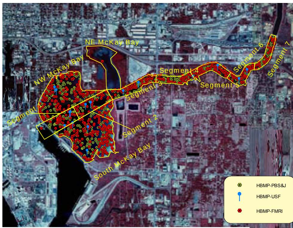
Figure 2-14 Location of All HBMP Stations
