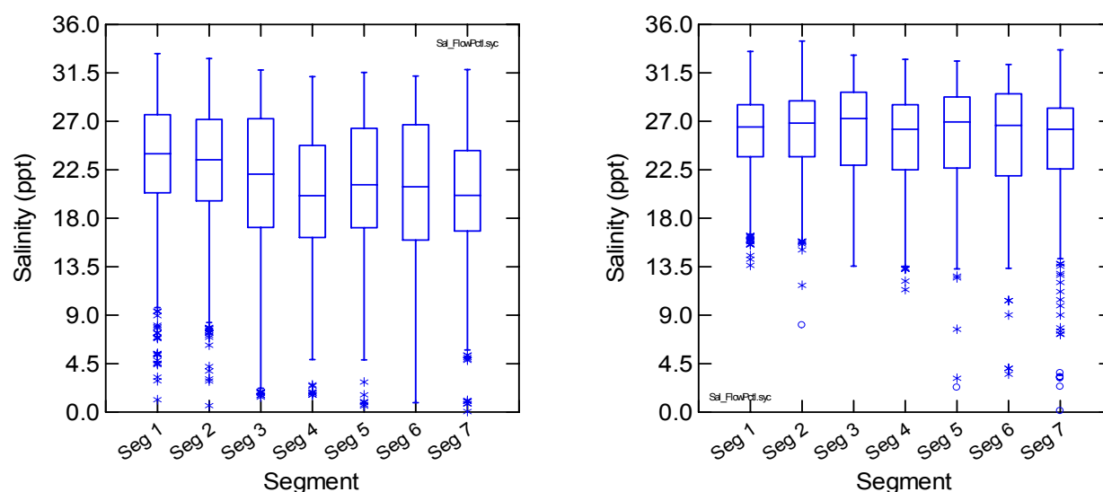
Figure 3-10 TBC Salinity 1974 -2003 at < 1 m (left) and \geq 3 m (right)
