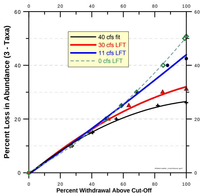
Figure 3-9 Effect of LFT on Abundance at Various Withdrawal Rates
