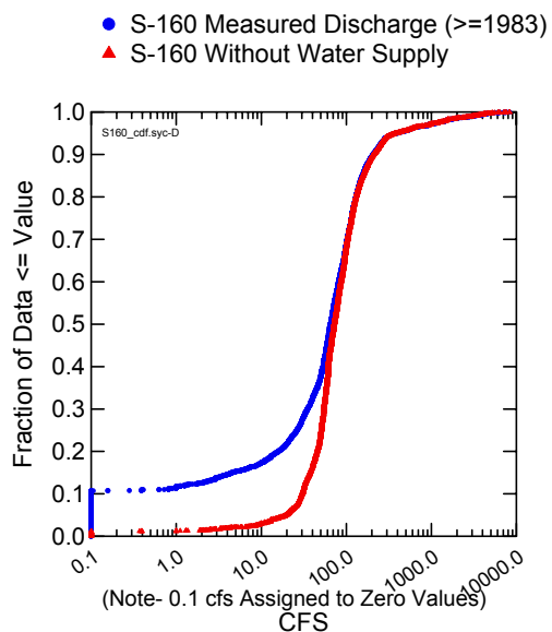
Figure 2-12 S-160 Flows - Measured (S1) and Baseline (S2)
