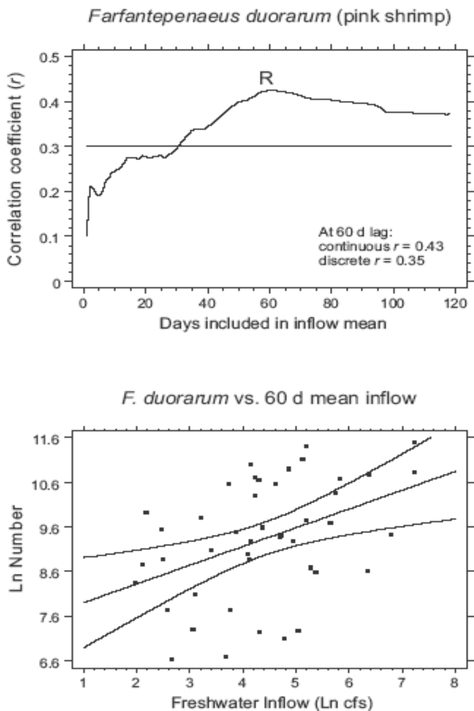
Figure 3-5 Example Lag Flow / Abundance Regression - Pink Shrimp
