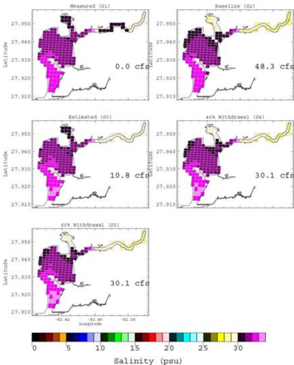
Figure 3-25 Modeled 25-Hour Average Bottom Salinity (Feb 15, 2001) for Five Flow Scenarios
