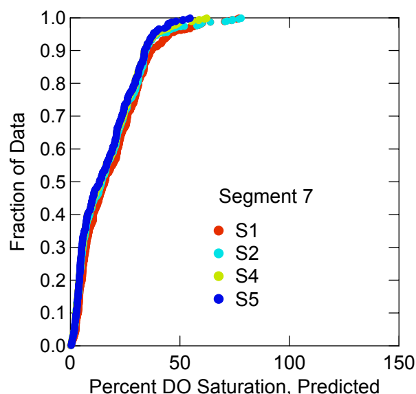
Figure 3-19 Predicted Percent DO Saturation for Observed (S1), Baseline (S2), 40% Withdrawal (S4) and 60% Withdrawal (S5) Scenarios
