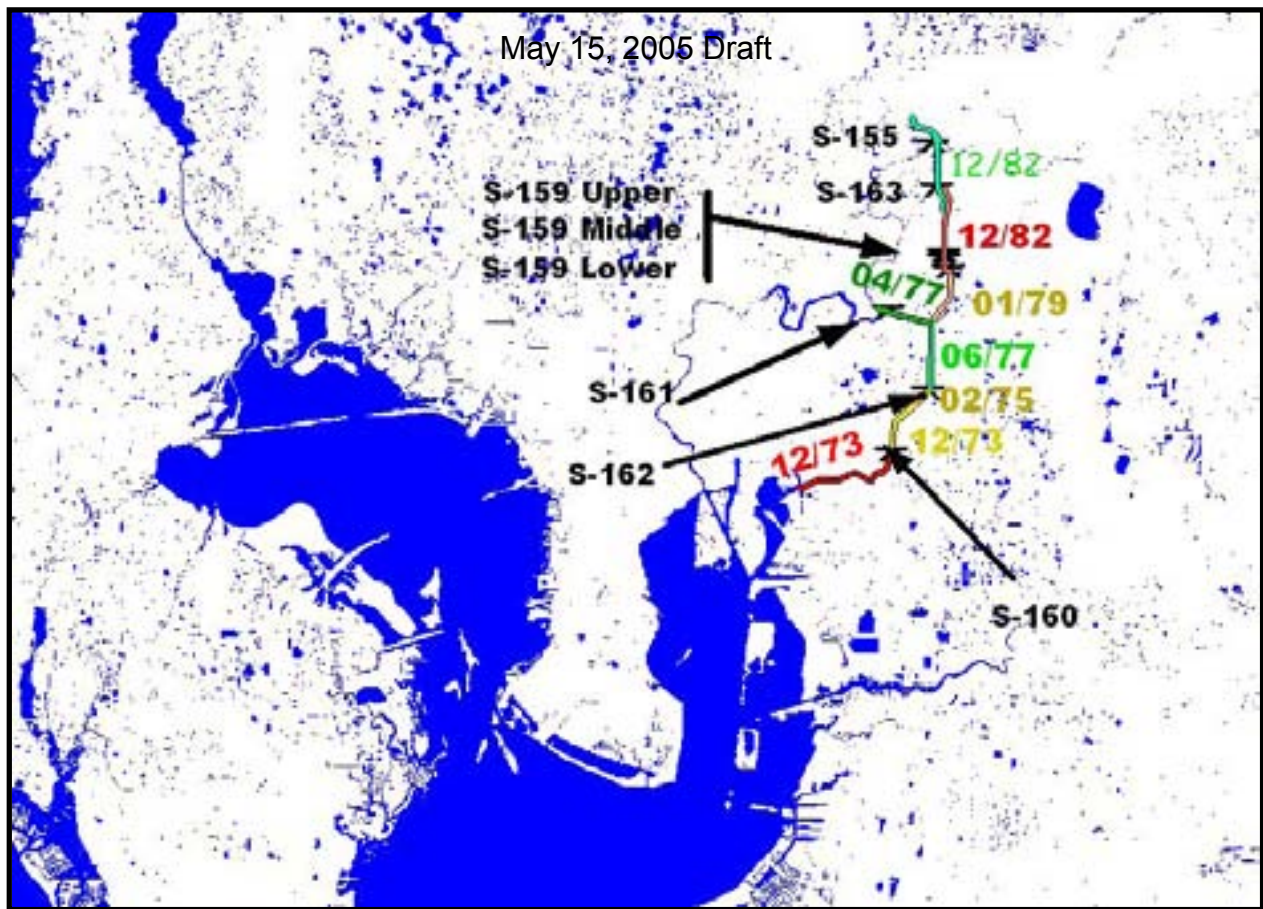
Figure 2-4 TBC Construction Completion Dates
