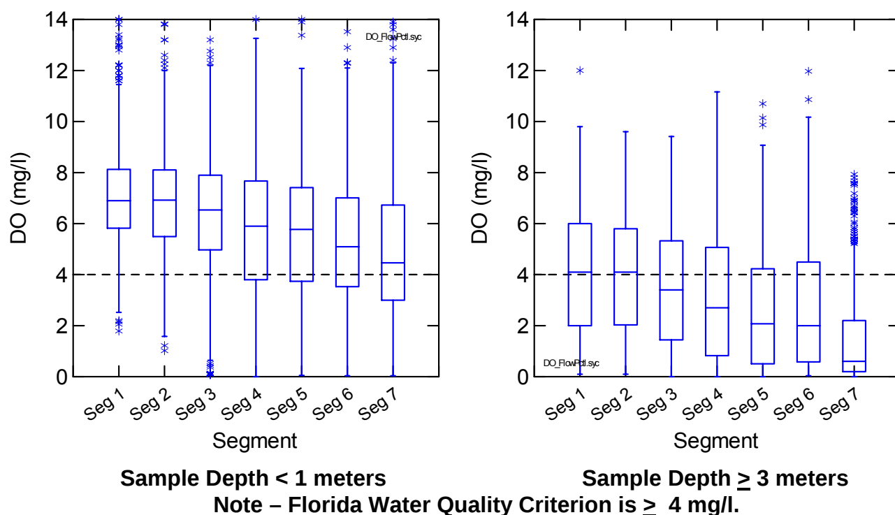
Figure 3-16 Dissolved Oxygen 1974-2003
