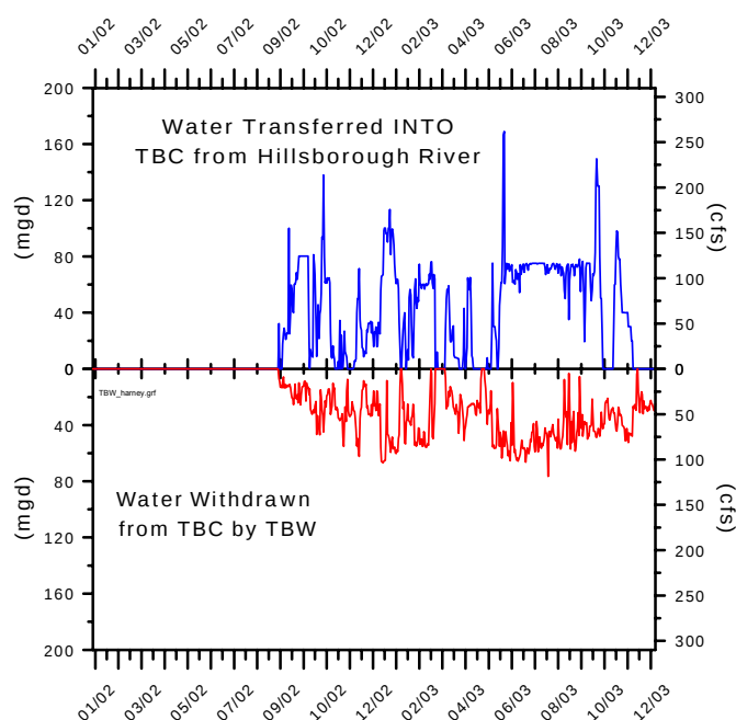
Figure 3-22 TBW Diversions and Withdrawals from TBC
