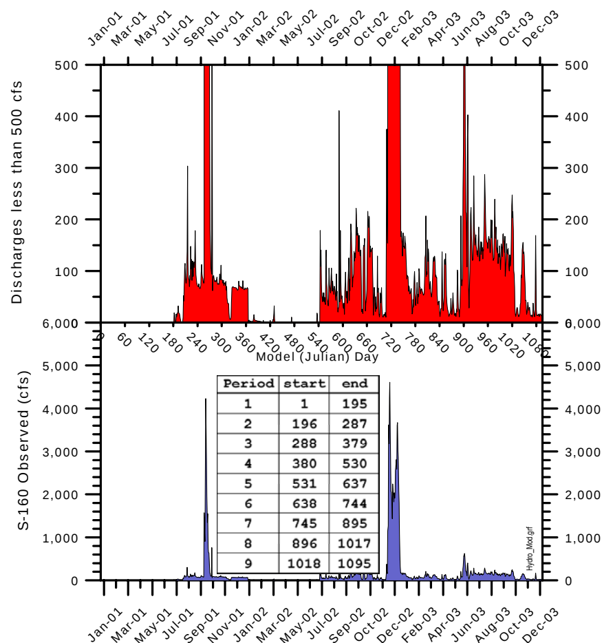
Figure 3-23 S-160 Discharge and Model Periods Evaluated.
