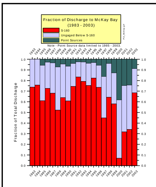
Figure 2-9 Relative Contribution of Freshwater to McKay Bay. Annual Average 1983-2003
