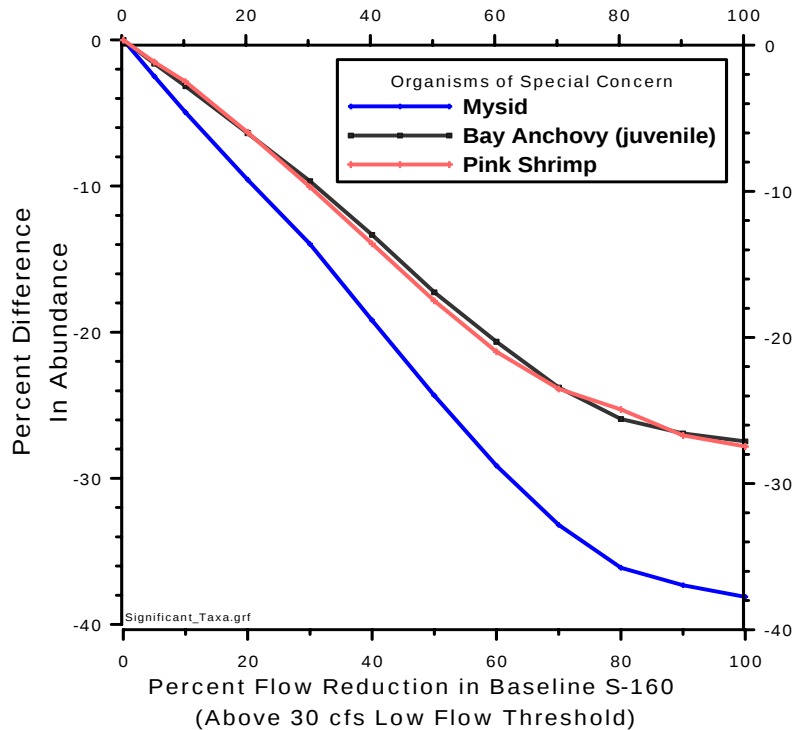
Figure 3-8 Abundance / Inflow Relationship for Three Significant Taxa
