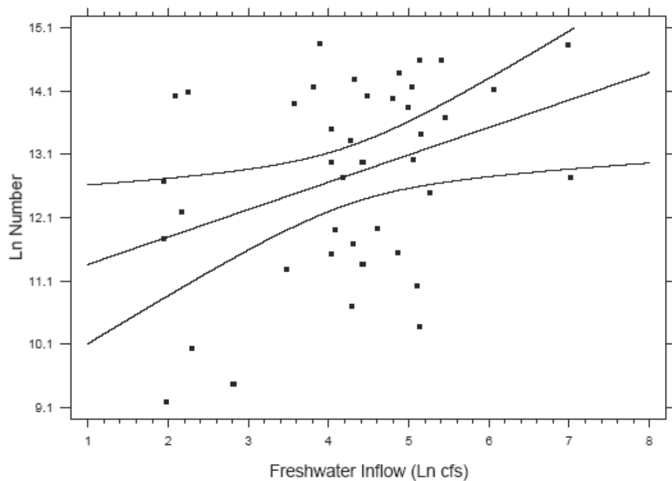
Figure 3-6 Example Lag Flow Abundance Regression - Mysids and Anchovies
