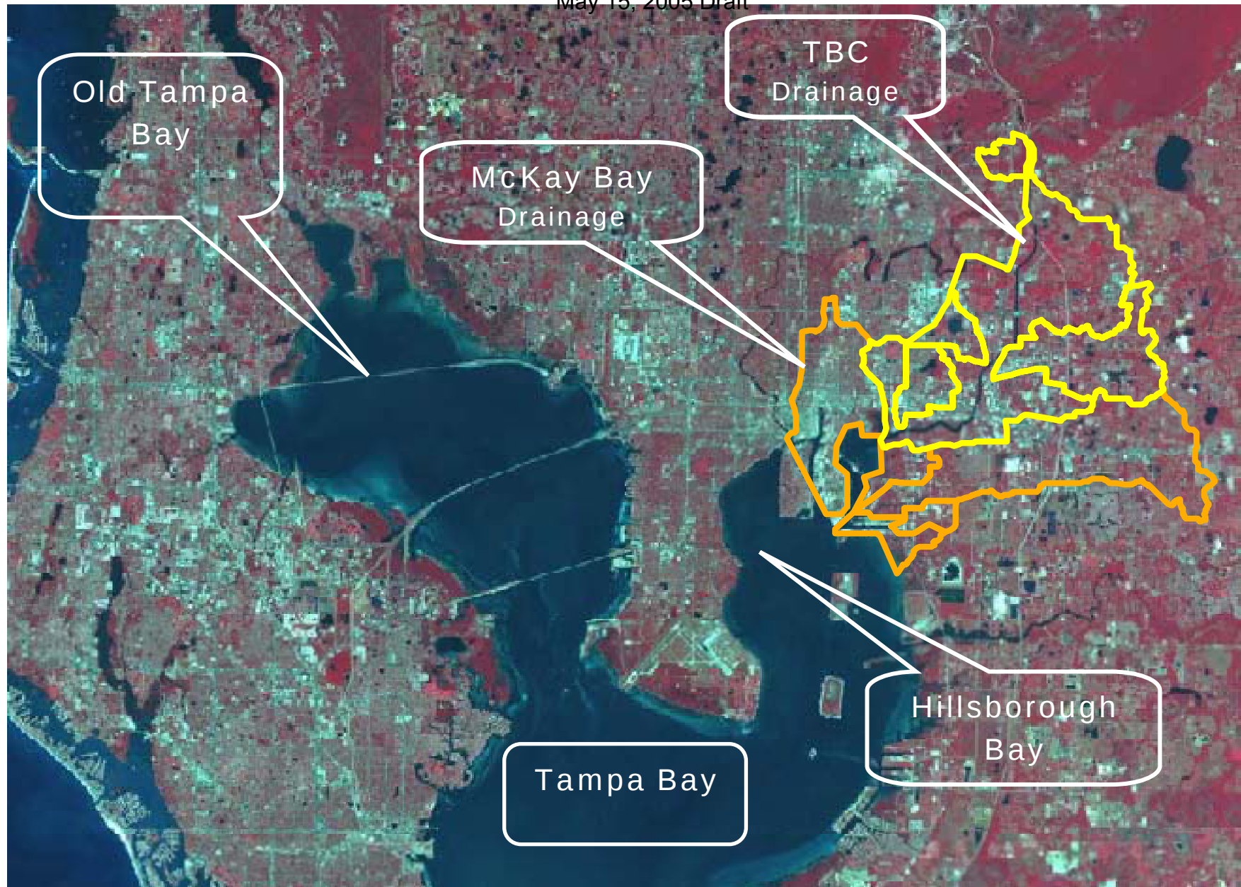
Figure 2-1 Location of McKay Bay / TBC Complex
