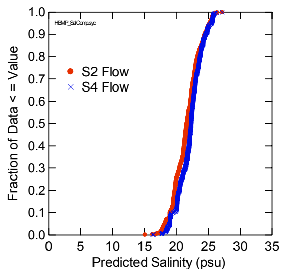
Figure 3-14 Palm River May Surface Salinities at Baseline and at Reduced Flow (see text)
