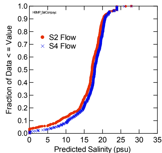
Figure 3-15 Palm River September Surface Salinities at Baseline and at Reduced Flow (see text)
