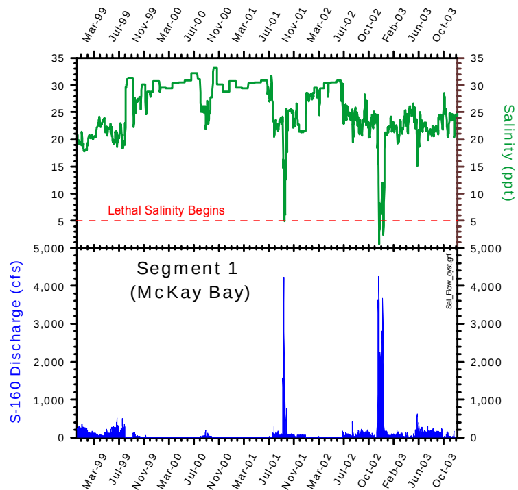
Figure 3-3 Modeled Salinity Time Series for TBC
