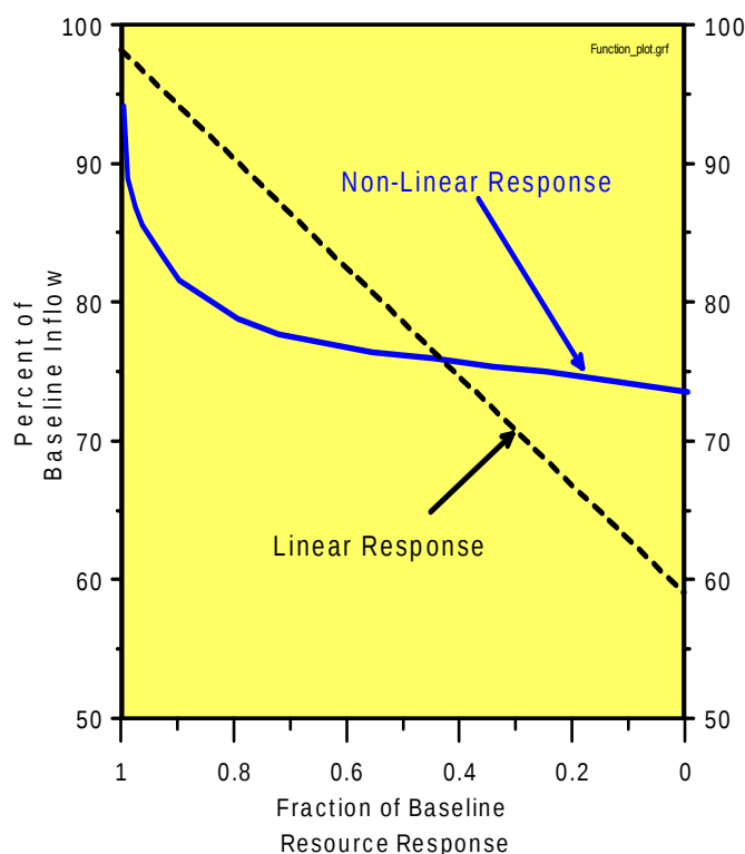
Figure 1-1 Examples of Linear and Non-Linear Response Variable
