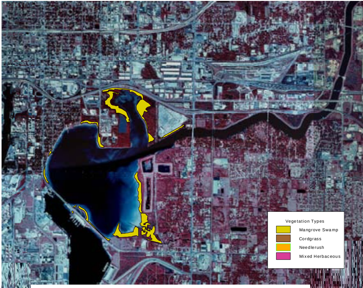
Figure 3-4 Emergent Vegetation in McKay Bay and Palm River
