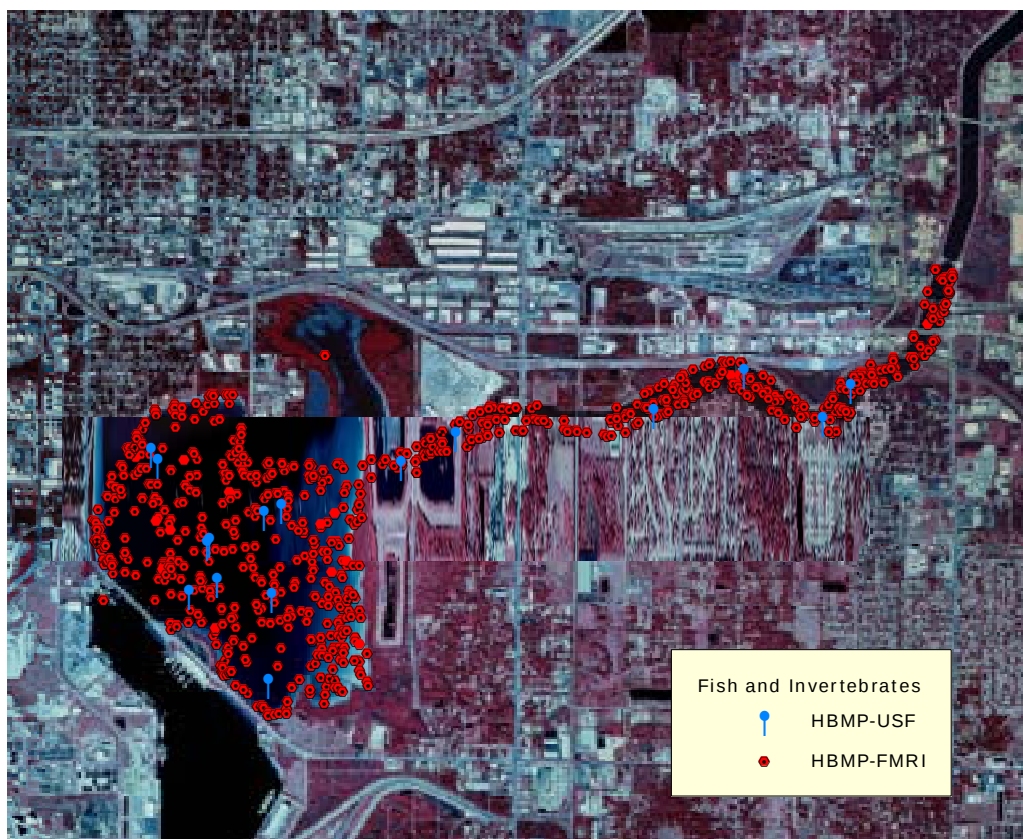
Figure 2-16 FMRI and USF Fish / Invertebrate Stations
