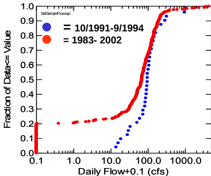
Figure 3-13 Comparison of S-160 Discharge on Sampling Days
