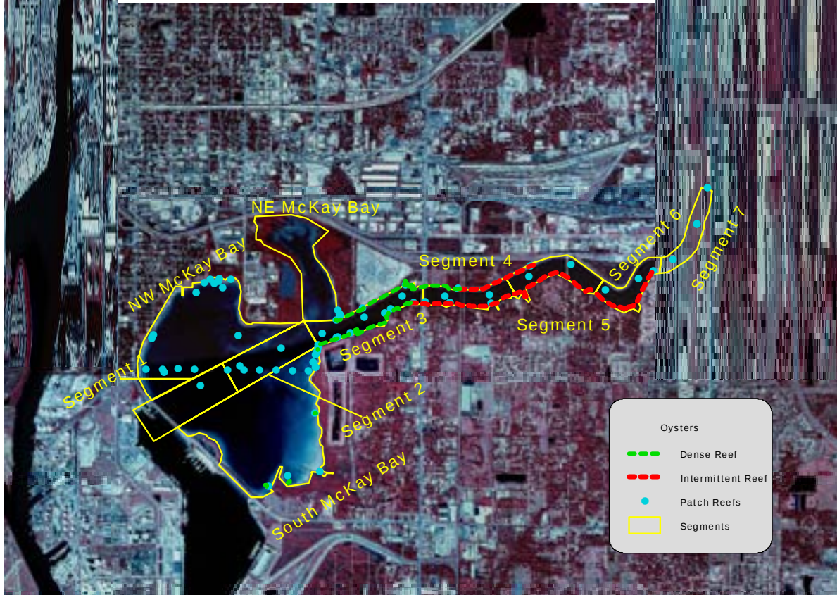
Figure 3-1 Oyster Communities Identified by Mote Marine Lab
