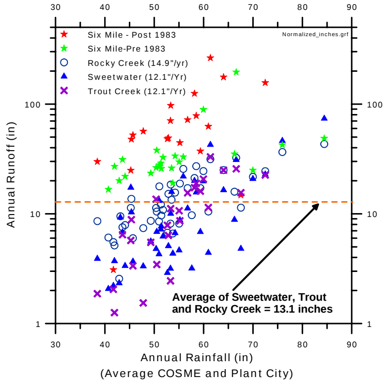
Figure 2-6 Regional Runoff/Rainfall Relationships (1957-2001)
