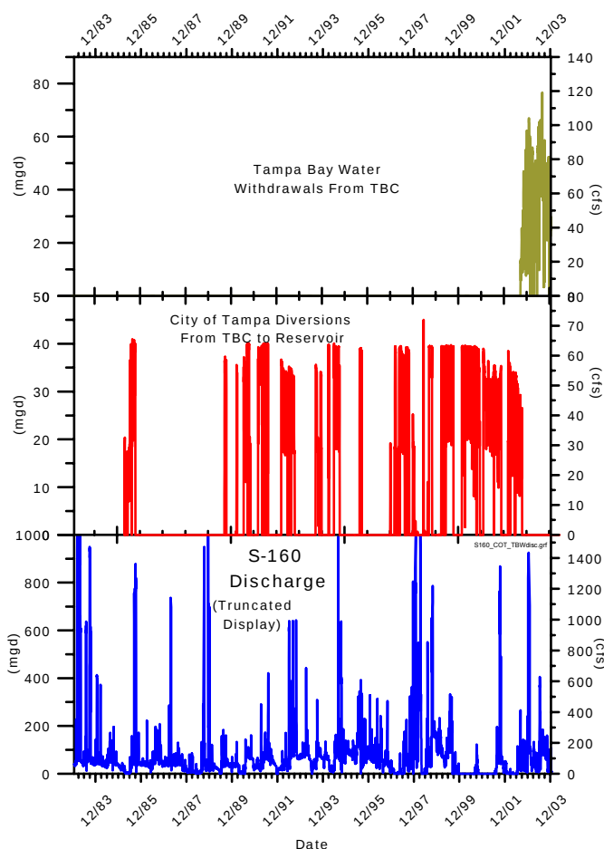
Figure 3-21 TBC Diversions and Discharges
