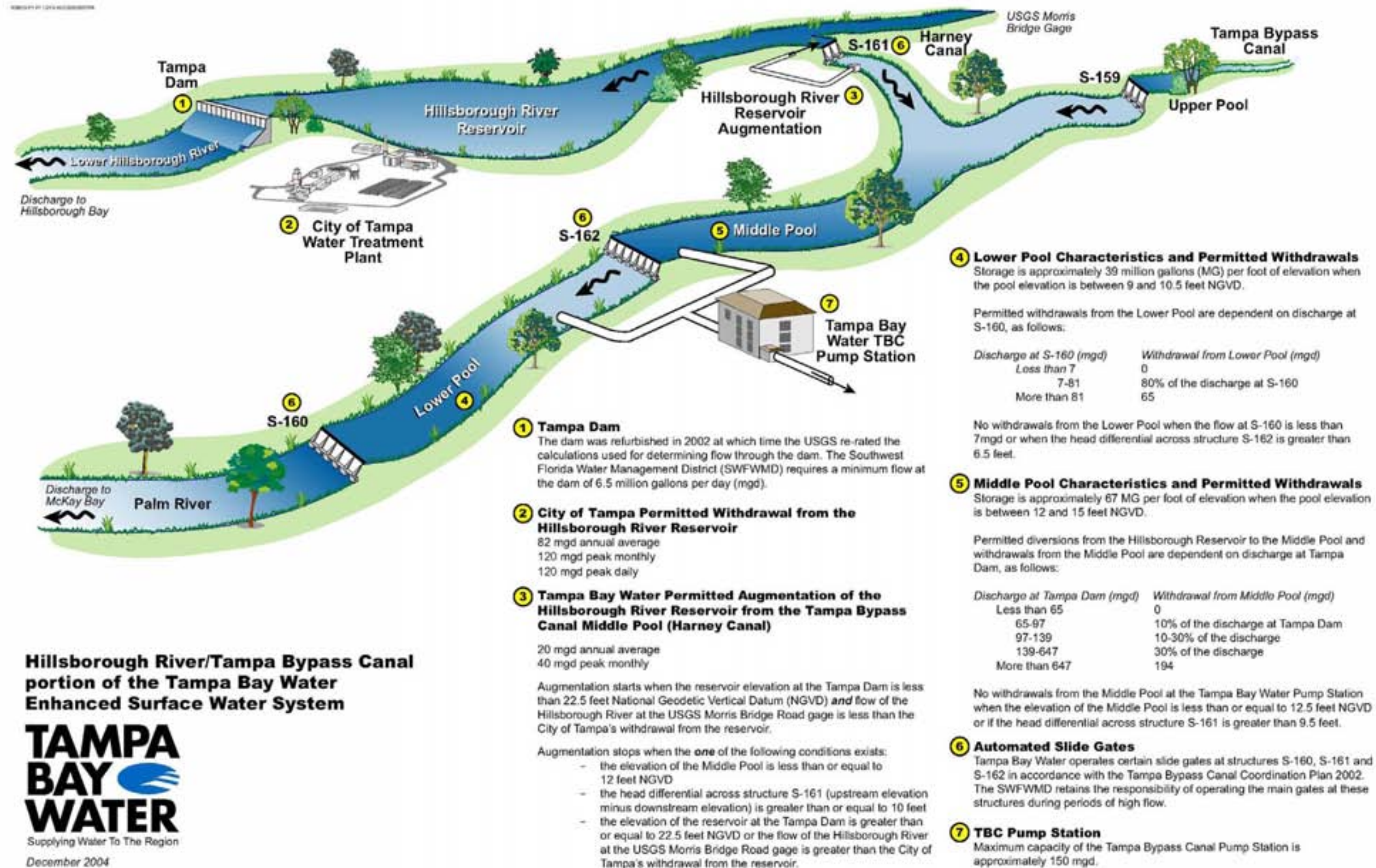
Figure 3 – 11 (Reproduced with Permission, TBW) TBC / Hillsborough Reservoir Permitted Withdrawals
