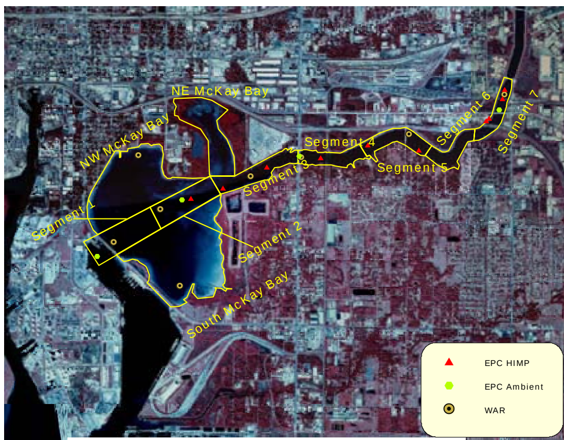
Figure 2-13 WAR, HIMP, EPCHC Ambient Stations
