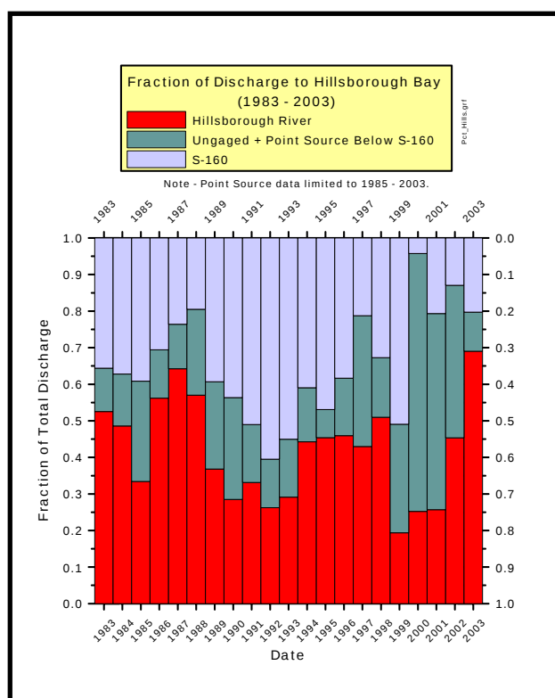
Figure 2-10 Relative Contribution of Freshwater to Upper Hillsborough Bay. Annual Average 1983-2003.
